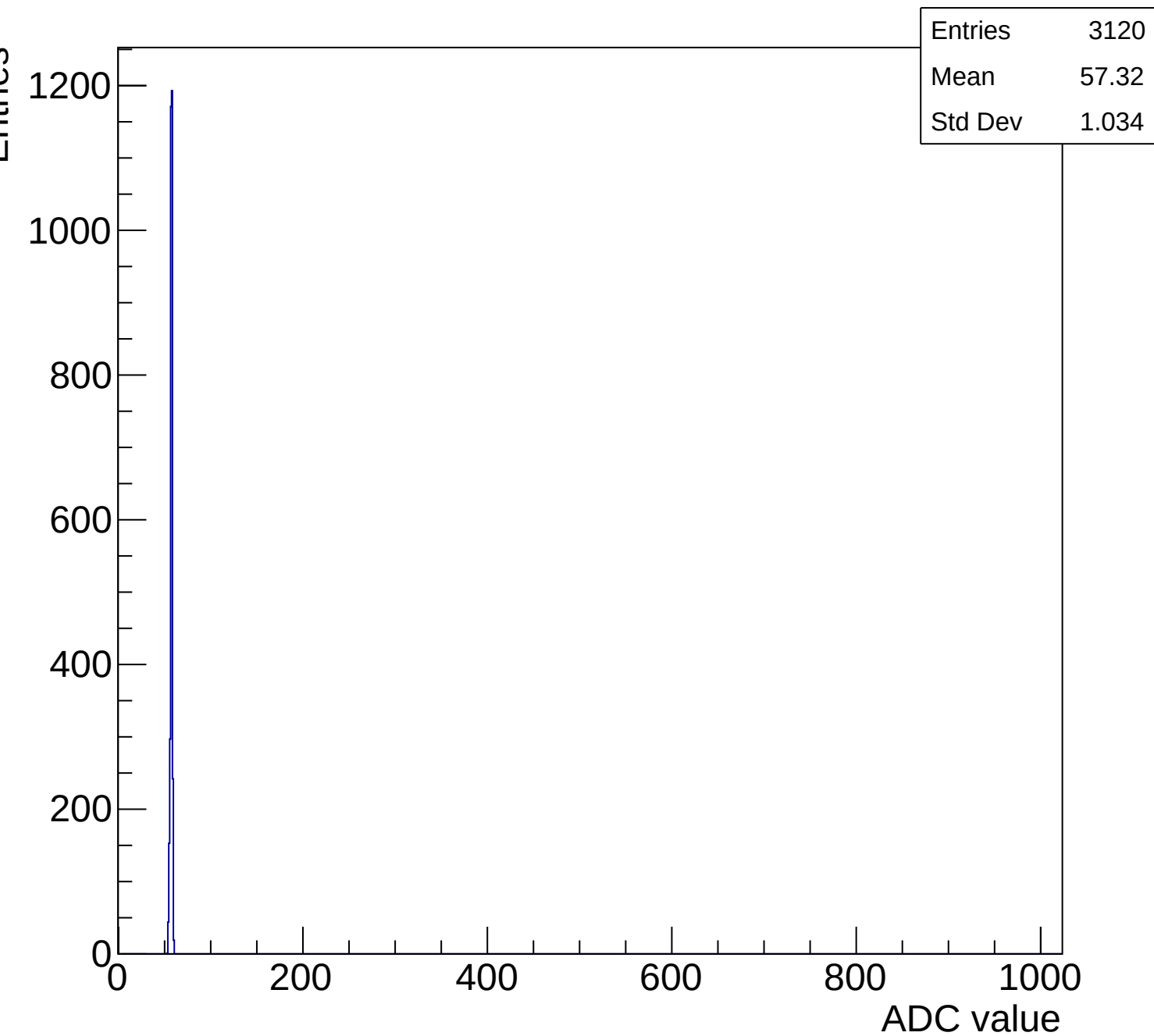
Peaktype 2 ped mcm0 saltro0 ch2 g3-s0-p1-s3
