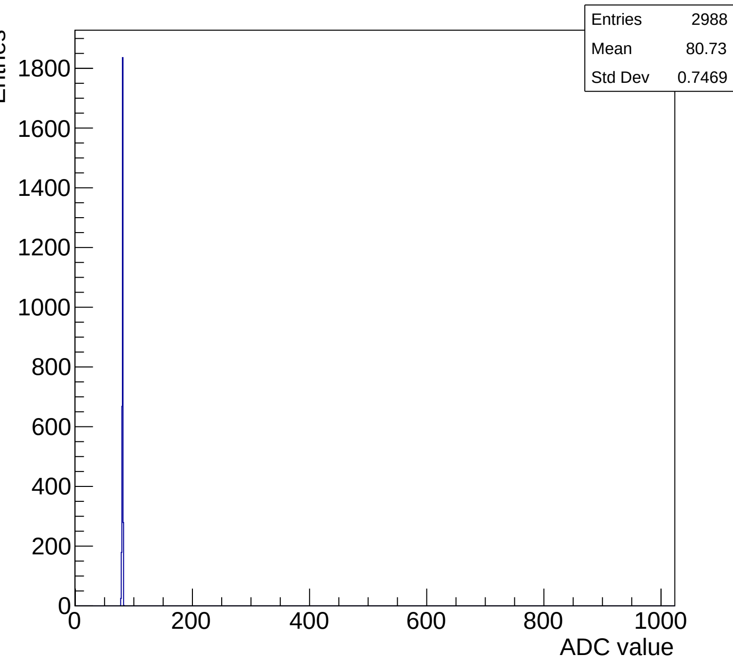
Peaktype 2 ped mcm0 saltro0 ch0 g1-s0-p1-s3
