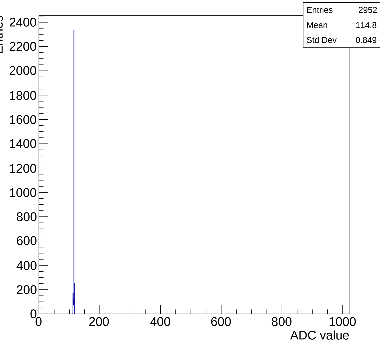
Peaktype 1 ped mcm0 saltro0 ch4 g0-s0-p1-s1
