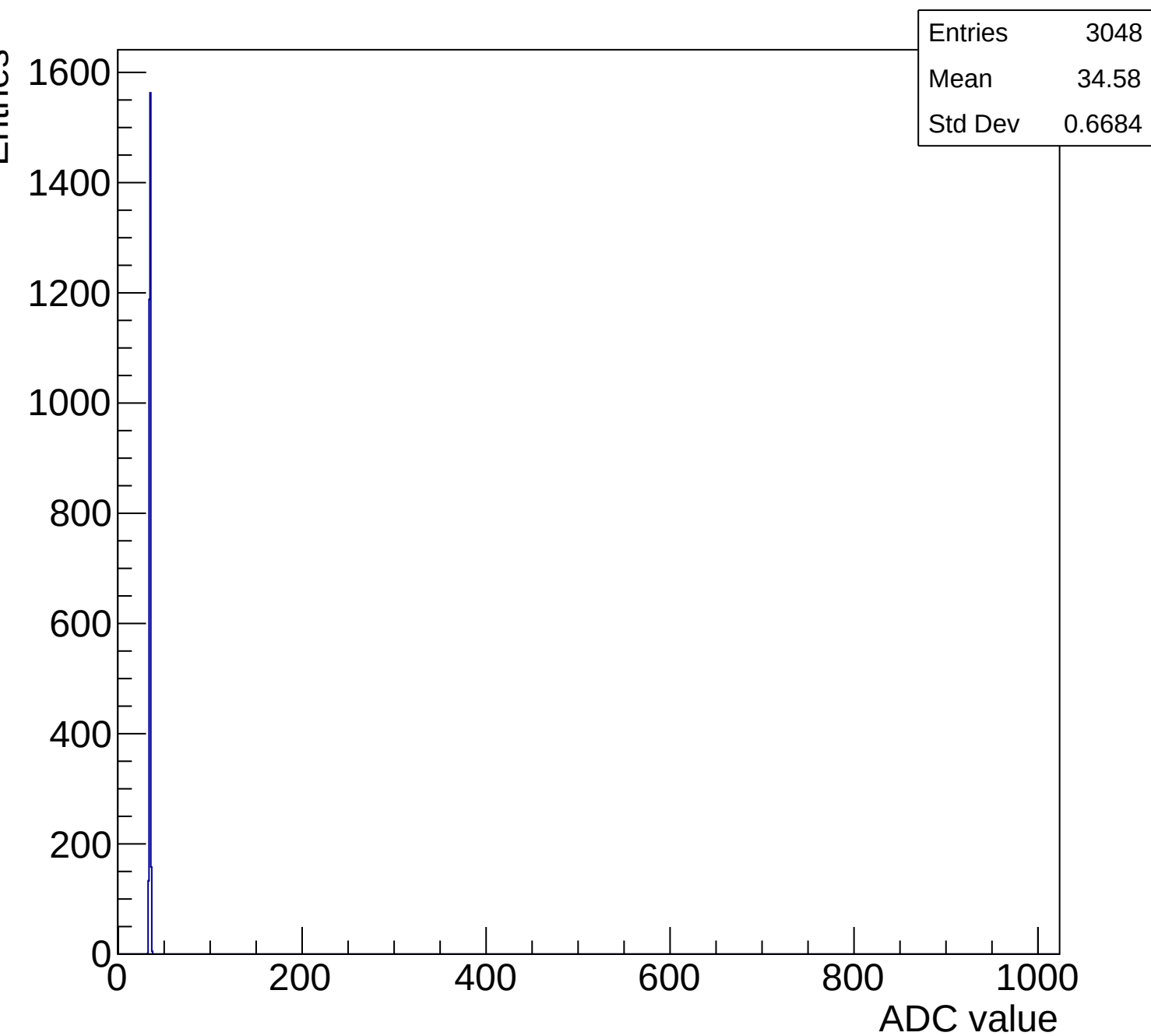
Peaktype 1 ped mcm0 saltro0 ch5 g3-s0-p1-s2-sh
