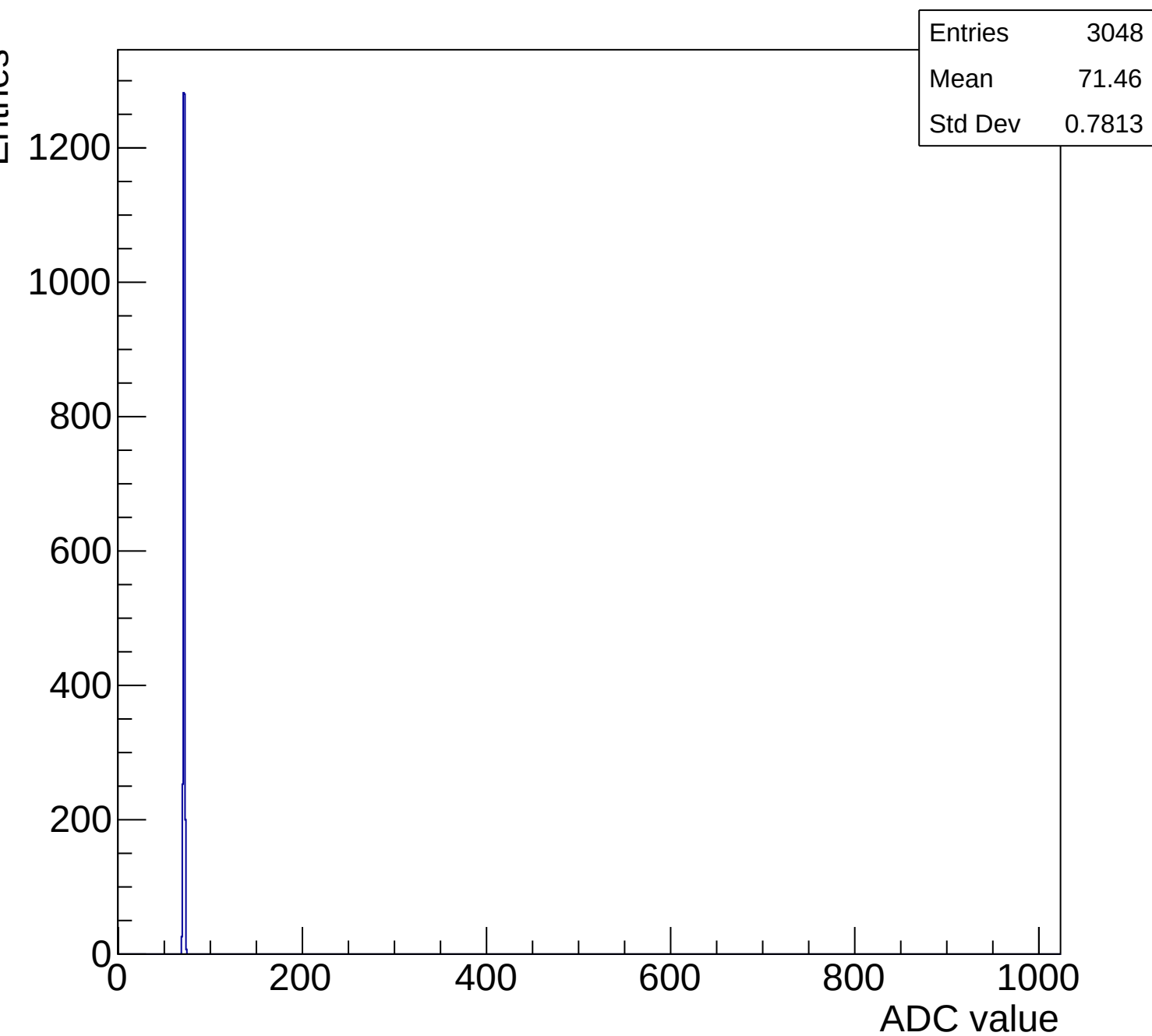
Peaktype 1 ped mcm0 saltro0 ch15 g3-s0-p1-s2-sh
