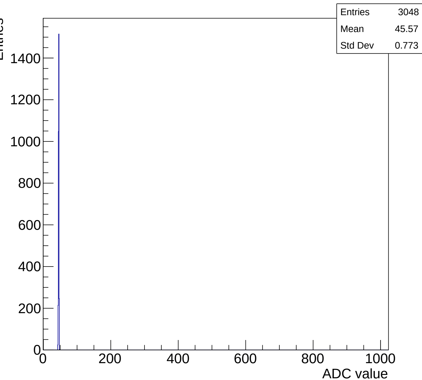
Peaktype 1 ped mcm0 saltro0 ch9 g3-s0-p1-s2-sh
