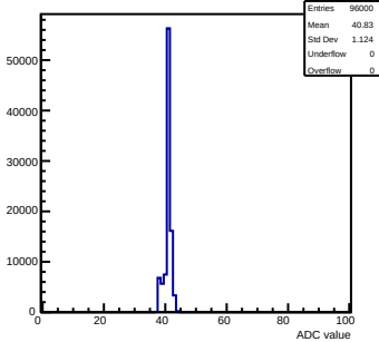
Pedestals mcm 0 ch 67 58ohm
