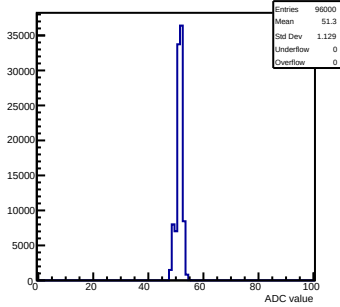
Pedestals mcm 0 ch 74 58ohm
