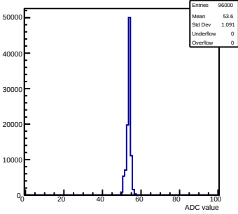
Pedestals mcm 0 ch 69 58ohm
