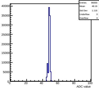
Pedestals mcm 0 ch 72 58ohm
