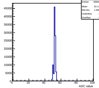
Pedestals mcm 0 ch 22 580hm
