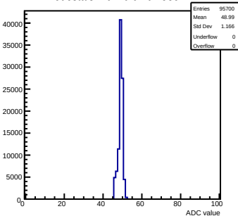
Pedestals mcm 0 ch 61 58ohm
