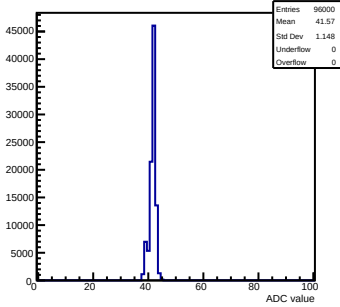
Pedestals mcm 0 ch 75 58ohm
