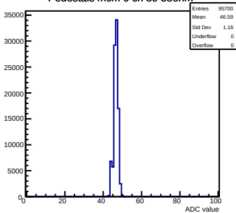
Pedestals mcm 0 ch 59 58ohm
