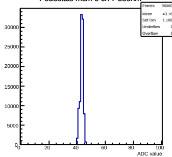
Pedestals mcm 0 ch 7 58ohm
