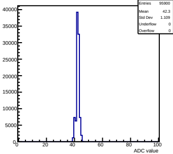
Pedestals mcm 0 ch 20 580hm
