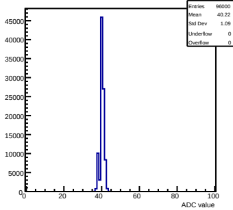
Pedestals mcm 0 ch 78 58ohm
