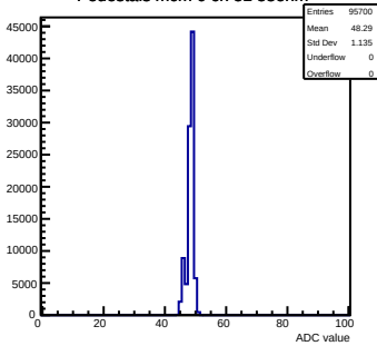
Pedestals mcm 0 ch 51 58ohm
