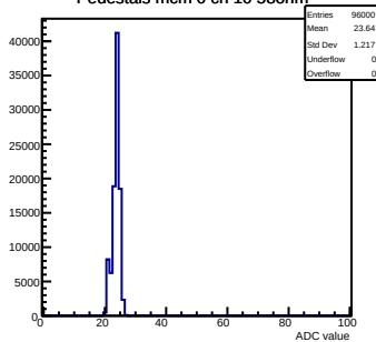
Pedestals mcm 0 ch 10 58ohm
