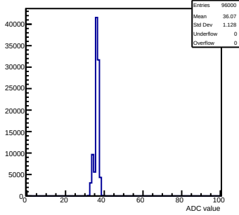
Pedestals mcm 0 ch 70 58ohm
