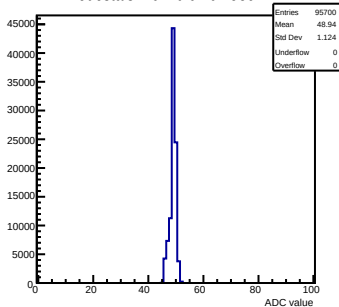
Pedestals mcm 0 ch 62 58ohm
