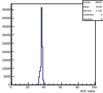
Pedestals mcm 0 ch 66 58ohm
