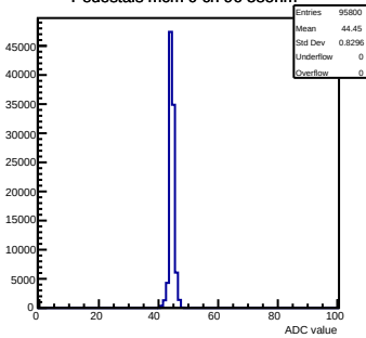
Pedestals mcm 0 ch 96 58ohm
