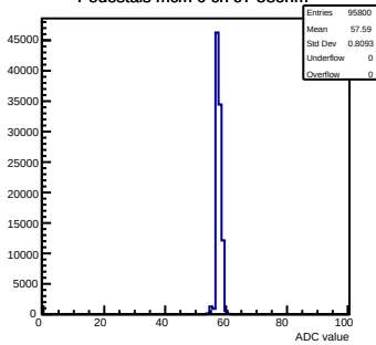
Pedestals mcm 0 ch 97 58ohm
