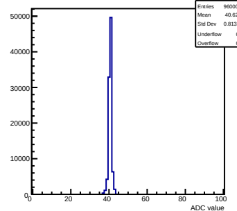
Pedestals mcm 0 ch 15 58ohm
