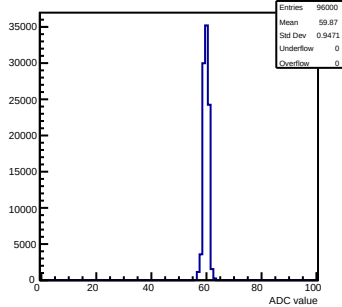
Pedestals mcm 0 ch 1 58ohm
