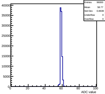
Pedestals mcm 0 ch 4 58ohm
