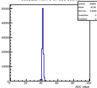
Pedestals mcm 0 ch 108 58ohm
