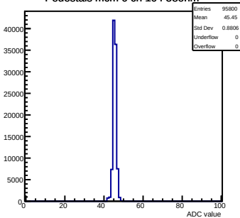
Pedestals mcm 0 ch 104 58ohm
