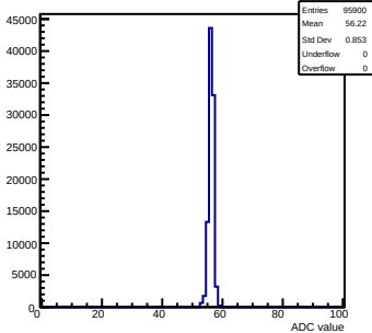
Pedestals mcm 0 ch 91 58ohm
