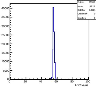
Pedestals mcm 0 ch 80 58ohm
