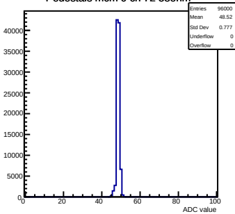
Pedestals mcm 0 ch 72 58ohm
