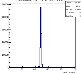
Pedestals mcm 0 ch 114 58ohm
