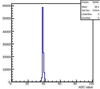
Pedestals mcm 0 ch 5 58ohm
