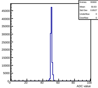
Pedestals mcm 0 ch 85 58ohm
