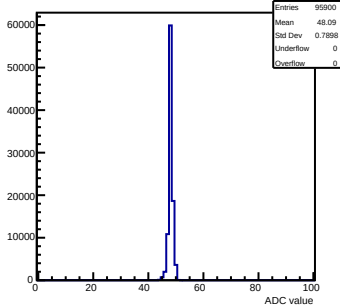
Pedestals mcm 0 ch 82 58ohm
