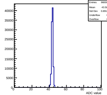
Pedestals mcm 0 ch 7 58ohm
