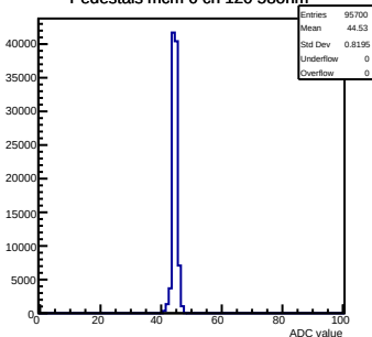
Pedestals mcm 0 ch 120 58ohm
