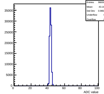
Pedestals mcm 0 ch 3 58ohm
