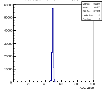
Pedestals mcm 0 ch 111 58ohm
