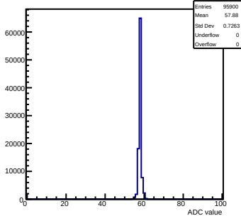
Pedestals mcm 0 ch 90 58ohm
