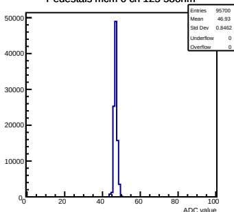
Pedestals mcm 0 ch 125 58ohm
