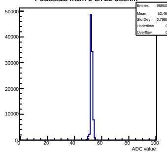
Pedestals mcm 0 ch 22 580hm
