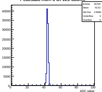
Pedestals mcm 0 ch 121 58ohm
