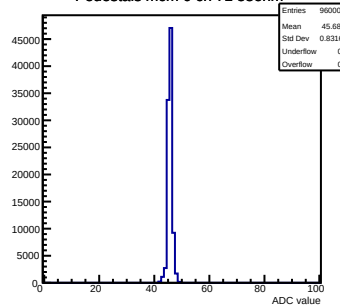
Pedestals mcm 0 ch 71 58ohm
