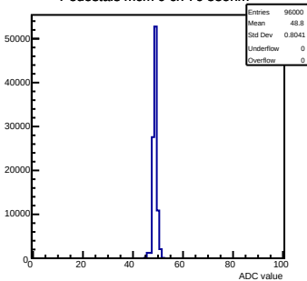
Pedestals mcm 0 ch 76 58ohm
