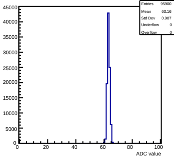
Pedestals mcm 0 ch 83 58ohm
