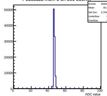
Pedestals mcm 0 ch 106 58ohm
