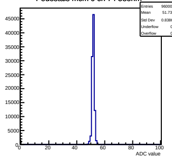
Pedestals mcm 0 ch 74 58ohm
