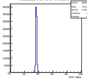
Pedestals mcm 0 ch 70 58ohm
