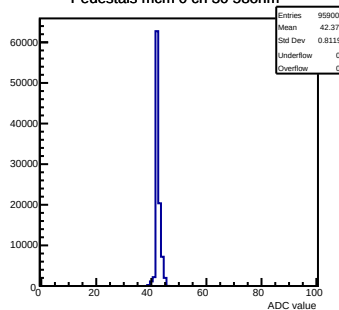
Pedestals mcm 0 ch 30 580hm
