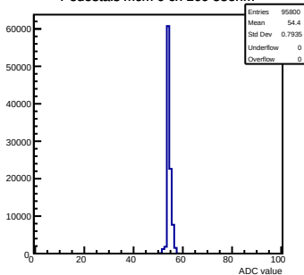
Pedestals mcm 0 ch 109 58ohm
