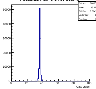
Pedestals mcm 0 ch 66 58ohm
