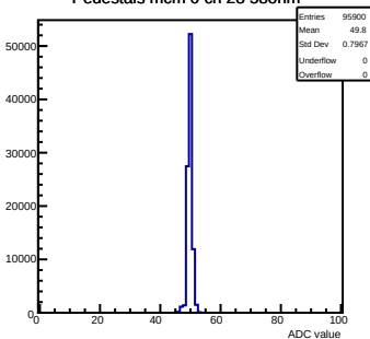
Pedestals mcm 0 ch 28 580hm
