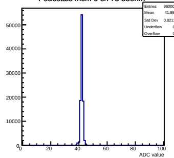
Pedestals mcm 0 ch 75 58ohm
