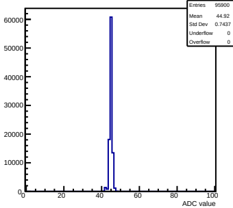
Pedestals mcm 0 ch 87 58ohm
