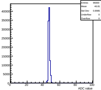
Pedestals mcm 0 ch 8 58ohm
