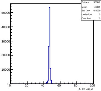
Pedestals mcm 0 ch 84 58ohm
