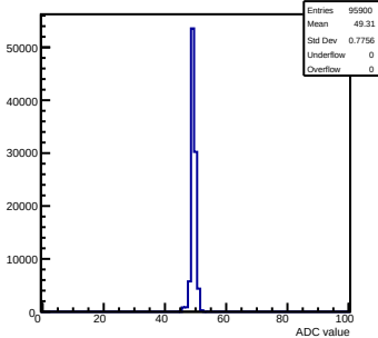
Pedestals mcm 0 ch 89 58ohm
