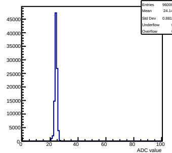
Pedestals mcm 0 ch 10 58ohm
