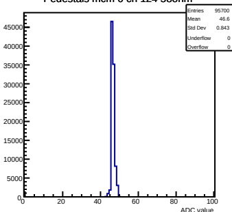
Pedestals mcm 0 ch 124 58ohm
