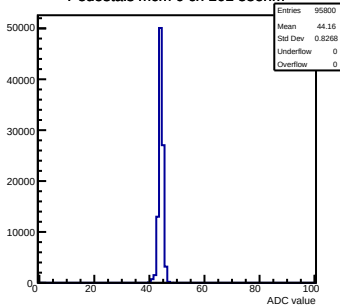
Pedestals mcm 0 ch 101 58ohm
