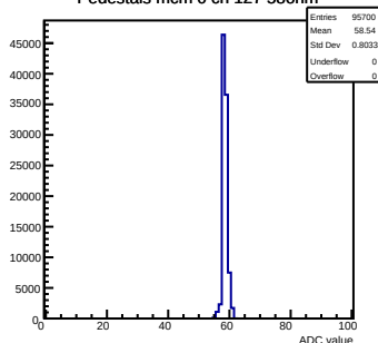
Pedestals mcm 0 ch 127 58ohm
