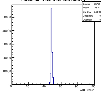
Pedestals mcm 0 ch 123 58ohm
