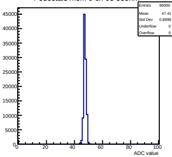
Pedestals mcm 0 ch 68 58ohm
