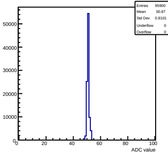
Pedestals mcm 0 ch 93 58ohm
