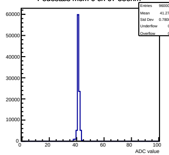
Pedestals mcm 0 ch 67 58ohm
