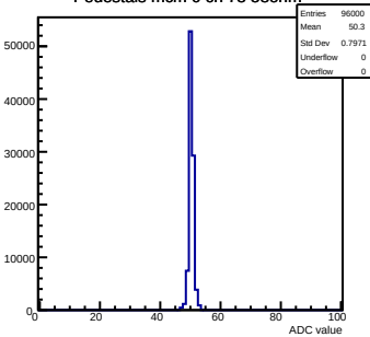
Pedestals mcm 0 ch 73 58ohm
