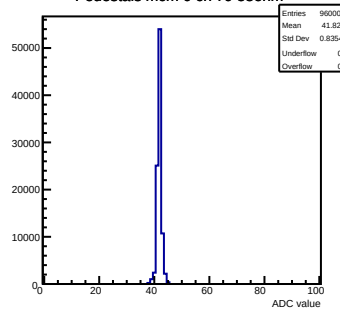
Pedestals mcm 0 ch 79 58ohm
