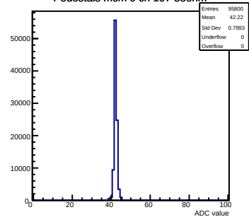
Pedestals mcm 0 ch 107 58ohm
