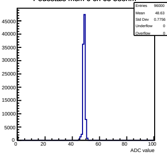
Pedestals mcm 0 ch 65 58ohm
