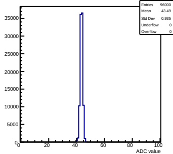
Pedestals mcm 0 ch 9 58ohm
