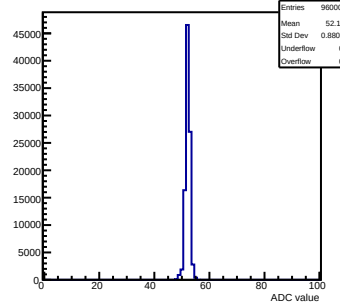
Pedestals mcm 0 ch 6 58ohm
