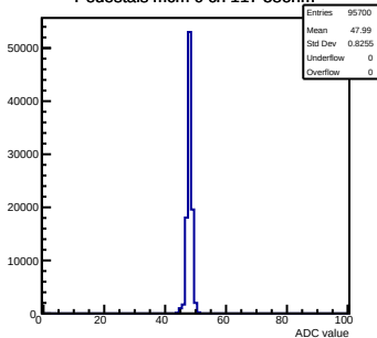
Pedestals mcm 0 ch 117 58ohm
