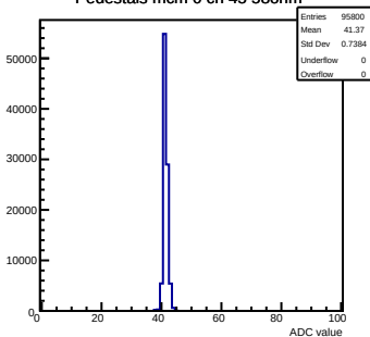
Pedestals mcm 0 ch 45 58ohm
