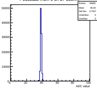
Pedestals mcm 0 ch 37 58ohm
