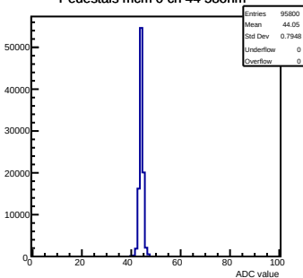
Pedestals mcm 0 ch 44 58ohm
