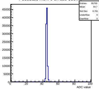
Pedestals mcm 0 ch 120 58ohm
