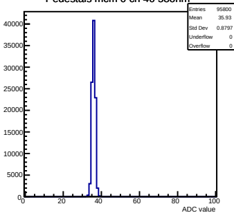
Pedestals mcm 0 ch 40 58ohm
