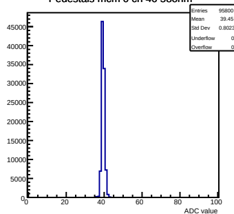
Pedestals mcm 0 ch 46 58ohm
