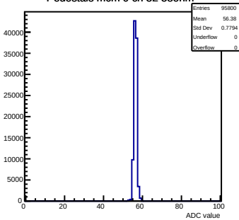
Pedestals mcm 0 ch 32 58ohm
