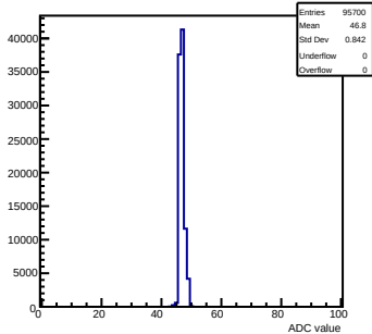
Pedestals mcm 0 ch 124 58ohm
