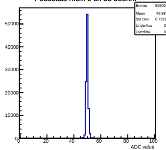
Pedestals mcm 0 ch 38 58ohm
