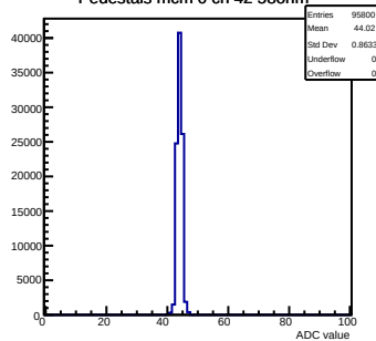
Pedestals mcm 0 ch 42 58ohm
