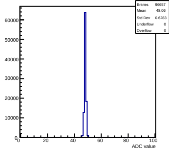
Pedestals mcm 0 ch 59 58ohm
