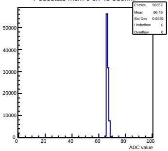
Pedestals mcm 0 ch 49 58ohm
