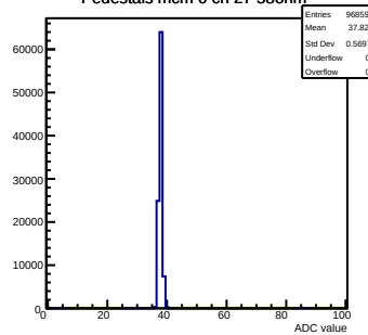
Pedestals mcm 0 ch 27 58ohm
