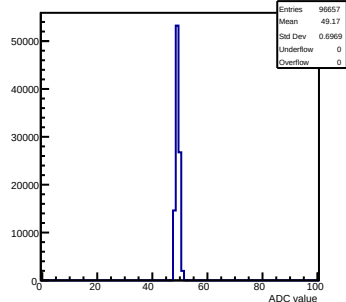
Pedestals mcm 0 ch 58 58ohm
