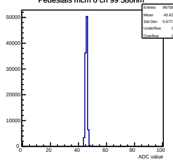
Pedestals mcm 0 ch 99 58ohm
