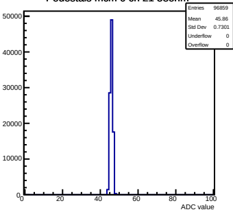
Pedestals mcm 0 ch 21 58ohm
