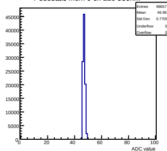
Pedestals mcm 0 ch 126 58ohm
