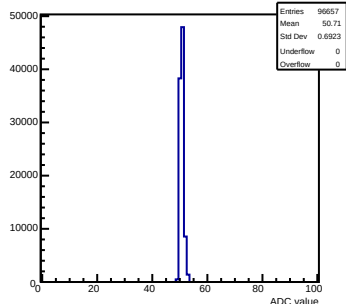
Pedestals mcm 0 ch 63 58ohm
