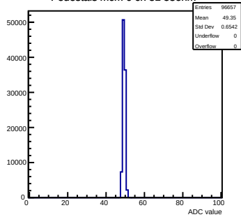
Pedestals mcm 0 ch 51 58ohm
