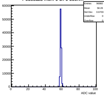
Pedestals mcm 0 ch 0 58ohm
