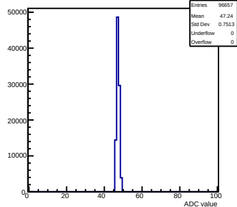
Pedestals mcm 0 ch 54 58ohm
