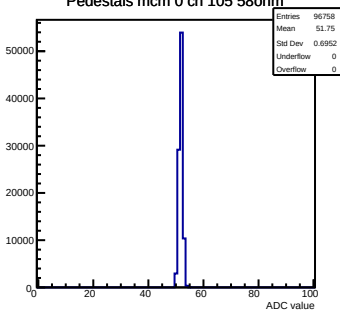
Pedestals mcm 0 ch 105 58ohm
