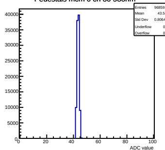
Pedestals mcm 0 ch 30 58ohm
