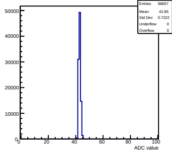
Pedestals mcm 0 ch 55 58ohm
