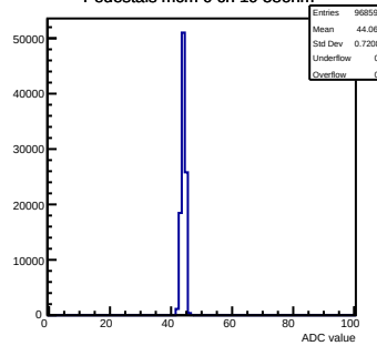
Pedestals mcm 0 ch 19 58ohm
