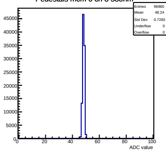
Pedestals mcm 0 ch 8 58ohm
