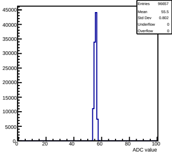
Pedestals mcm 0 ch 52 58ohm
