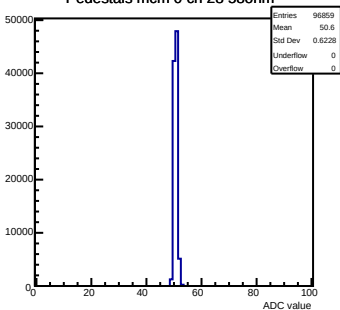
Pedestals mcm 0 ch 28 58ohm
