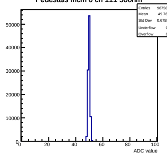
Pedestals mcm 0 ch 111 58ohm
