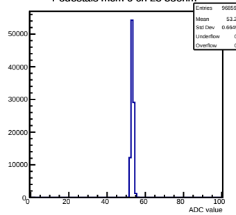
Pedestals mcm 0 ch 23 58ohm
