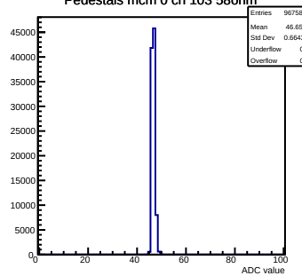
Pedestals mcm 0 ch 103 58ohm
