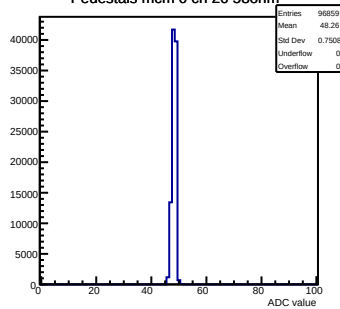
Pedestals mcm 0 ch 26 58ohm
