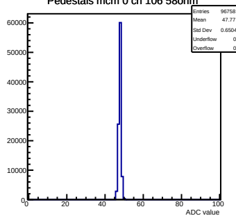
Pedestals mcm 0 ch 106 58ohm
