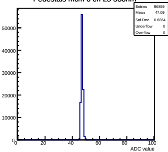
Pedestals mcm 0 ch 25 58ohm
