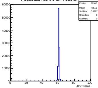
Pedestals mcm 0 ch 4 58ohm
