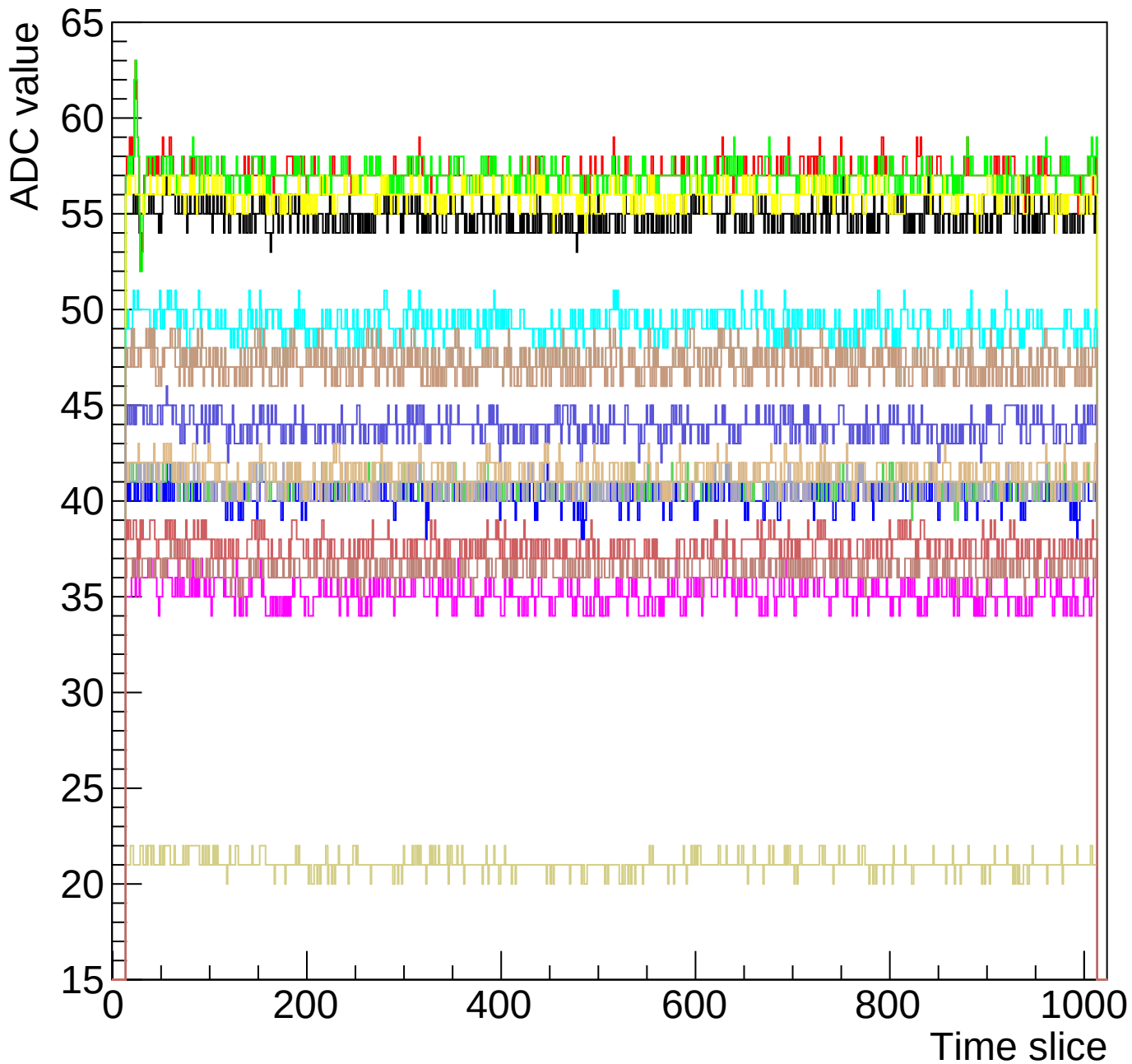
Run 120 event 10 mcm 0 chip 0 58ohm
