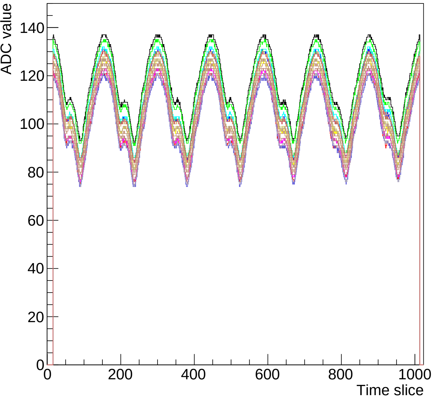
Run 123 event 10 mcm 0 chip 2 0ohm
