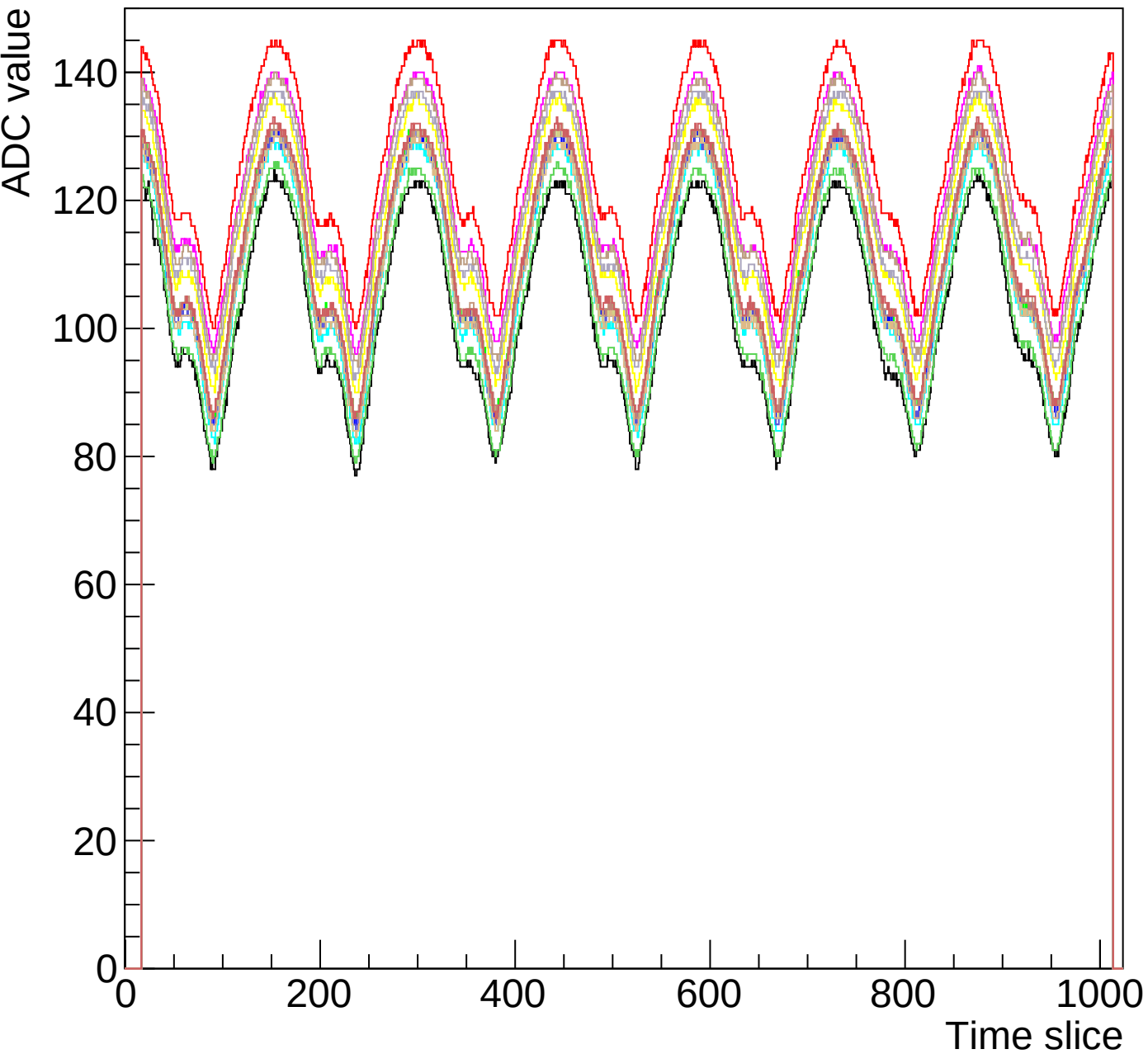
Run 123 event 10 mcm 0 chip 3 0ohm
