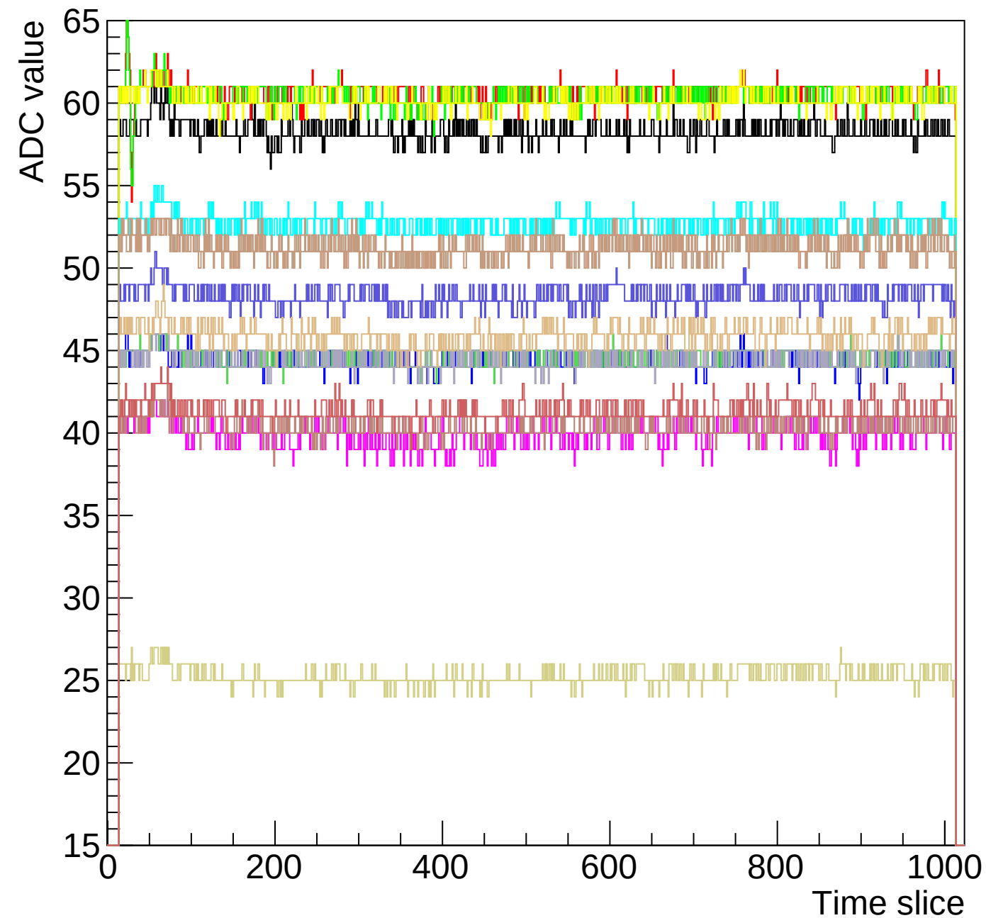
Run 120 event 1000 mcm 0 chip 0 58ohm
