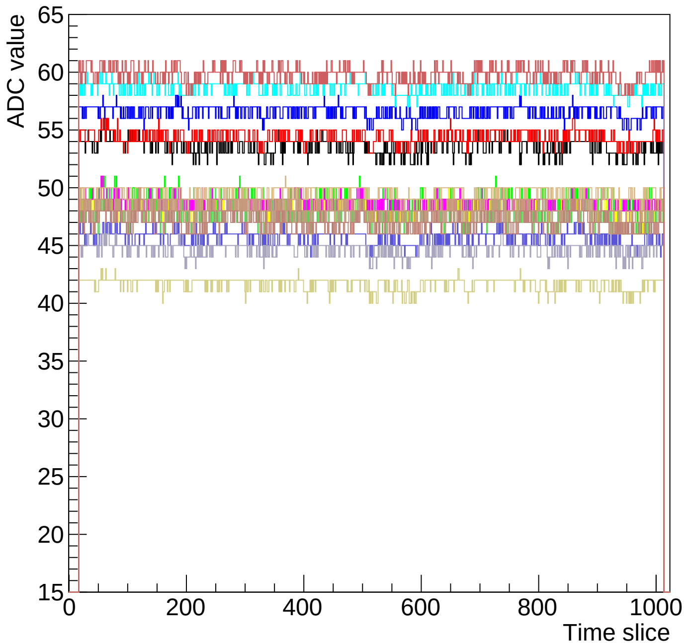
Run 120 event 995 mcm 0 chip 7 58ohm
