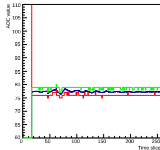
Run 0 Time mcm 0 chip 3 chan 7 256
