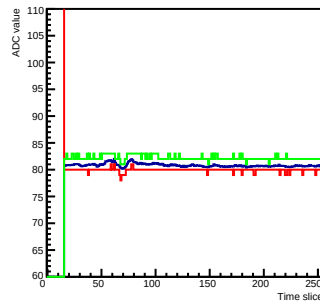
Run 0 Time mcm 0 chip 2 chan 6 256
