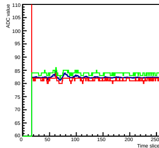
Run 0 Time mcm 0 chip 3 chan 11 256
