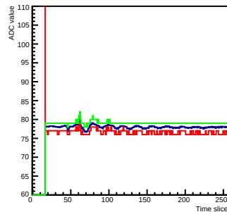
Run 0 Time mcm 0 chip 3 chan 3 256
