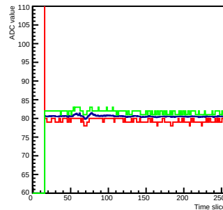
Run 0 Time mcm 0 chip 2 chan 11 256
