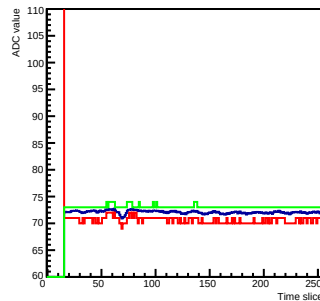
Run 0 Time mcm 0 chip 2 chan 14 256
