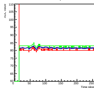
Run 0 Time mcm 0 chip 1 chan 8 256
