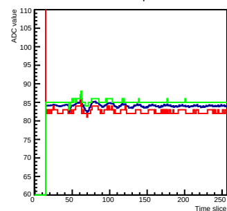
Run 0 Time mcm 0 chip 1 chan 11 256
