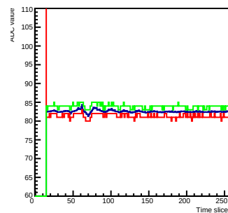
Run 0 Time mcm 0 chip 1 chan 12 256
