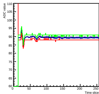
Run 0 Time mcm 0 chip 0 chan 1 256
