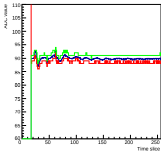
Run 0 Time mcm 0 chip 3 chan 0 256
