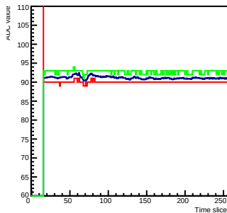
Run 0 Time mcm 0 chip 2 chan 4 256
