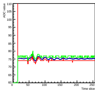
Run 0 Time mcm 0 chip 1 chan 1 256
