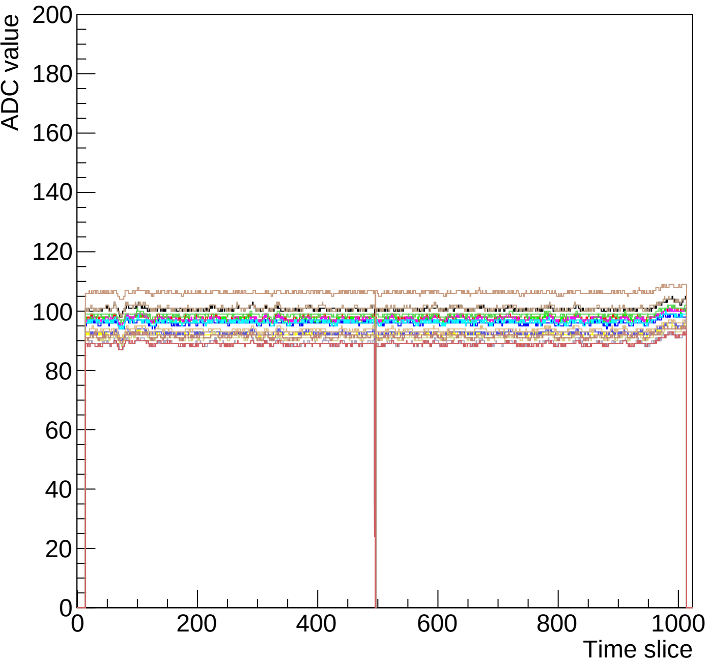
Run 0 event 3 mcm 0 chip 4 mcm11-1000
