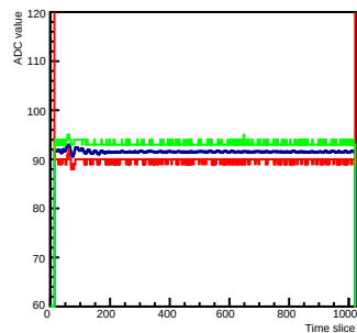
Run 0 Time mcm 0 chip 4 chan 15 mcm23
