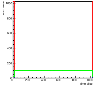
Run 0 Time mcm 0 chip 7 chan 7 s0-test
