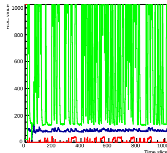
Run 3 Time mcm 0 chip 6 chan 15 s1-all
