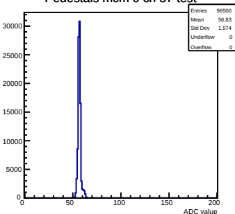
Pedestals mcm 0 ch 57 test
