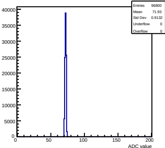
Pedestals mcm 0 ch 5 test
