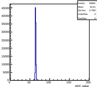
Pedestals mcm 0 ch 8 test
