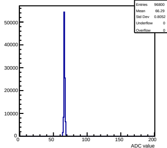
Pedestals mcm 0 ch 73 test
