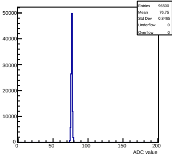
Pedestals mcm 0 ch 124 test
