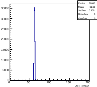
Pedestals mcm 0 ch 9 test
