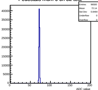
Pedestals mcm 0 ch 52 test
