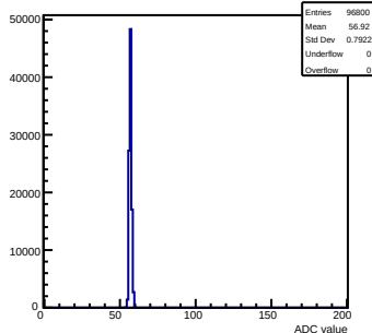
Pedestals mcm 0 ch 7 test
