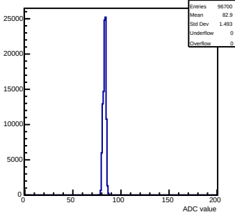
Pedestals mcm 0 ch 80 test
