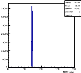
Pedestals mcm 0 ch 120 test
