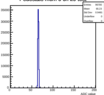
Pedestals mcm 0 ch 29 test
