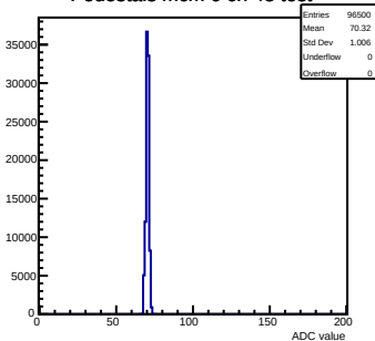
Pedestals mcm 0 ch 48 test
