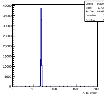
Pedestals mcm 0 ch 103 test
