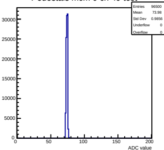
Pedestals mcm 0 ch 49 test
