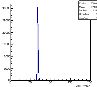
Pedestals mcm 0 ch 14 test
