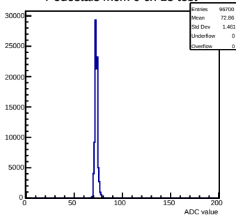
Pedestals mcm 0 ch 18 test
