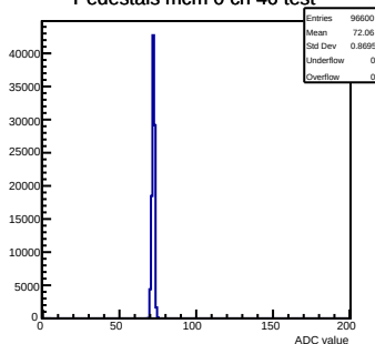
Pedestals mcm 0 ch 46 test
