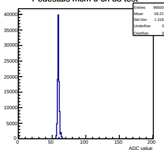
Pedestals mcm 0 ch 58 test
