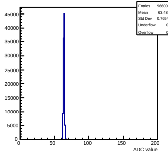
Pedestals mcm 0 ch 107 test
