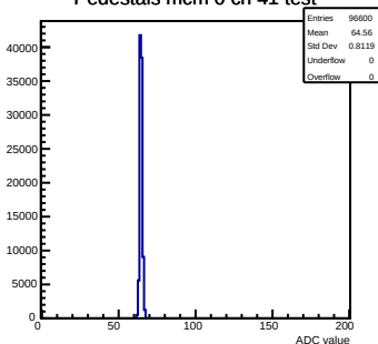
Pedestals mcm 0 ch 41 test
