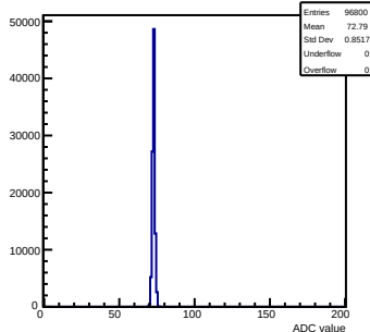
Pedestals mcm 0 ch 11 test
