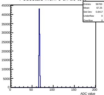
Pedestals mcm 0 ch 16 test
