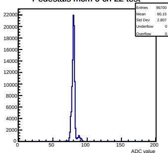
Pedestals mcm 0 ch 22 test
