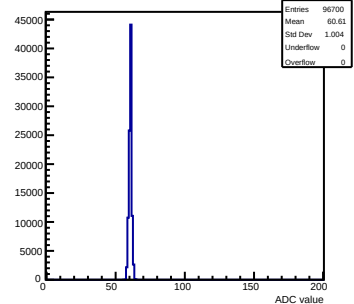
Pedestals mcm 0 ch 83 test
