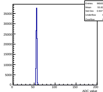
Pedestals mcm 0 ch 123 test
