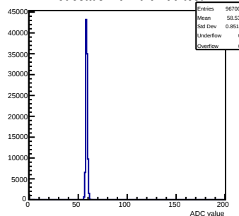
Pedestals mcm 0 ch 90 test
