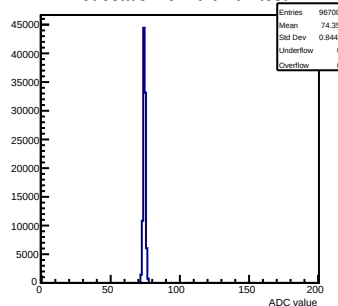
Pedestals mcm 0 ch 94 test
