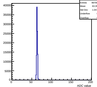
Pedestals mcm 0 ch 82 test
