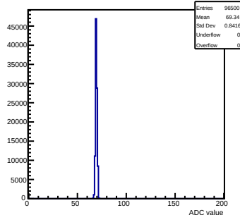
Pedestals mcm 0 ch 118 test
