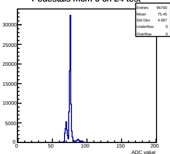
Pedestals mcm 0 ch 24 test
