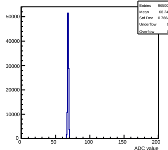
Pedestals mcm 0 ch 119 test
