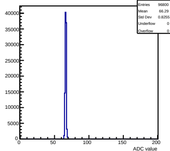
Pedestals mcm 0 ch 74 test
