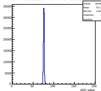
Pedestals mcm 0 ch 86 test
