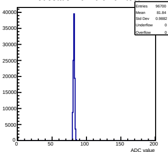
Pedestals mcm 0 ch 92 test
