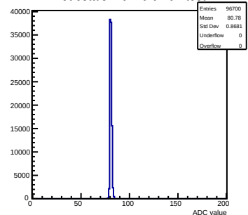
Pedestals mcm 0 ch 91 test
