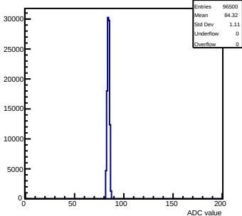
Pedestals mcm 0 ch 112 test
