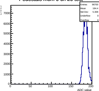
Pedestals mcm 0 ch 26 test
