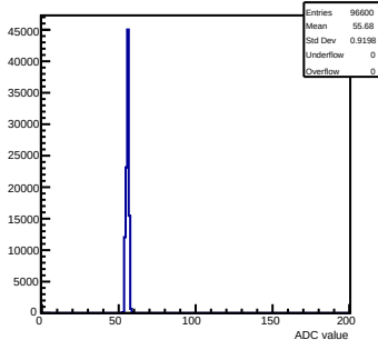
Pedestals mcm 0 ch 96 test
