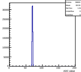
Pedestals mcm 0 ch 78 test
