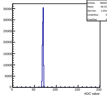
Pedestals mcm 0 ch 114 test
