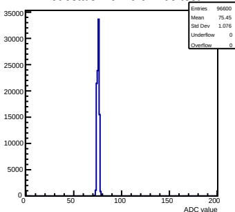
Pedestals mcm 0 ch 105 test
