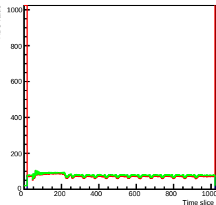
Run 2 Time mcm 0 chip 7 chan 12 s2-test2
