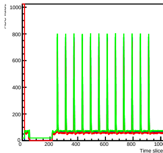
Run 1 Time mcm 0 chip 2 chan 2 s1-test0
