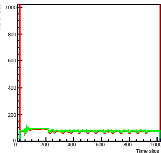
Run 2 Time mcm 0 chip 4 chan 12 s2-test0
