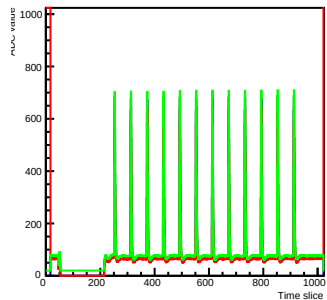
Run 2 Time mcm 0 chip 3 chan 1 s2-test0
