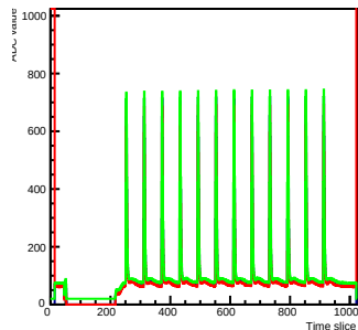
Run 2 Time mcm 0 chip 4 chan 13 s2-test0
