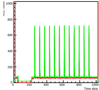
Run 2 Time mcm 0 chip 2 chan 13 s2-test0
