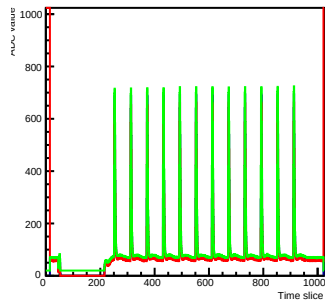
Run 2 Time mcm 0 chip 1 chan 1 s2-test0
