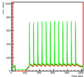
Run 2 Time mcm 0 chip 3 chan 15 s2-test0
