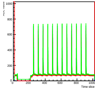
Run 2 Time mcm 0 chip 5 chan 1 s2-test0
