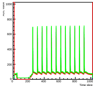
Run 2 Time mcm 0 chip 7 chan 7 s2-test0
