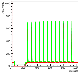
Run 2 Time mcm 0 chip 6 chan 3 s2-test0
