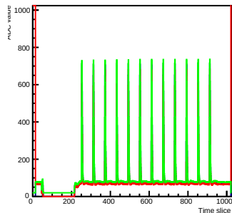
Run 2 Time mcm 0 chip 4 chan 5 s2-test0
