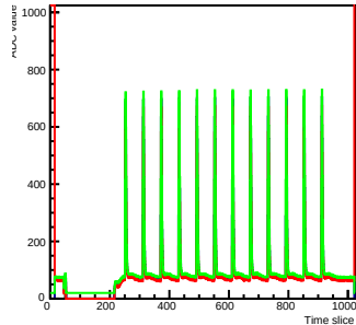
Run 2 Time mcm 0 chip 5 chan 13 s2-test0
