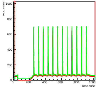
Run 2 Time mcm 0 chip 7 chan 11 s2-test2
