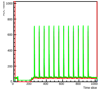
Run 2 Time mcm 0 chip 3 chan 13 s2-test2
