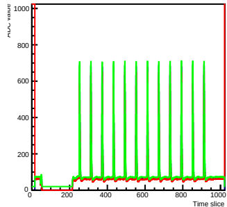
Run 2 Time mcm 0 chip 6 chan 5 s2-test2
