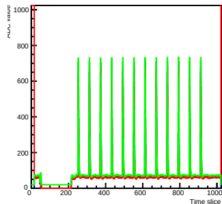
Run 2 Time mcm 0 chip 2 chan 13 s2-test2
