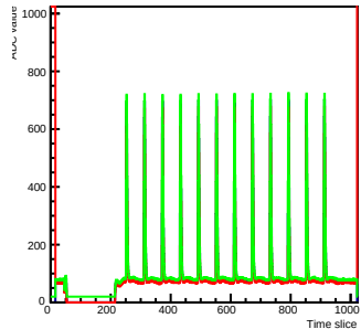
Run 2 Time mcm 0 chip 6 chan 13 s2-test2
