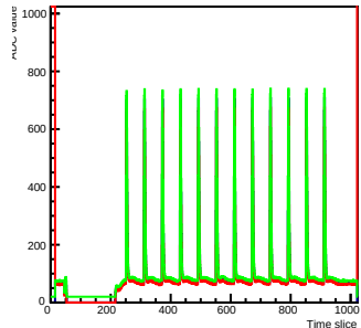
Run 2 Time mcm 0 chip 5 chan 13 s2-test2
