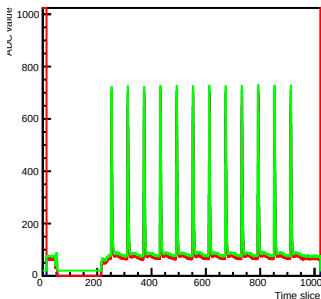
Run 2 Time mcm 0 chip 0 chan 11 s2-test2
