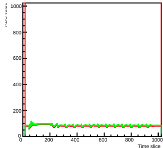
Run 2 Time mcm 0 chip 7 chan 14 s2-test2
