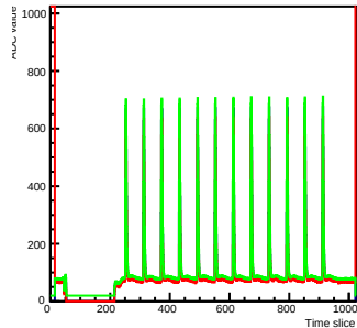
Run 2 Time mcm 0 chip 5 chan 1 s2-test4
