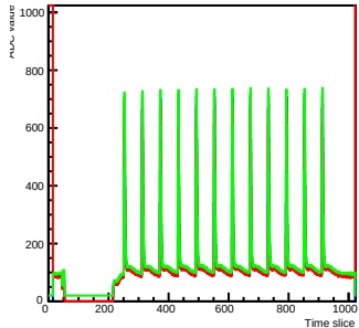
Run 2 Time mcm 0 chip 1 chan 9 s2-test4
