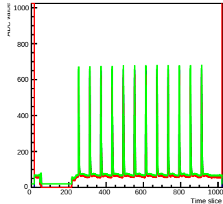
Run 2 Time mcm 0 chip 5 chan 9 s2-test4
