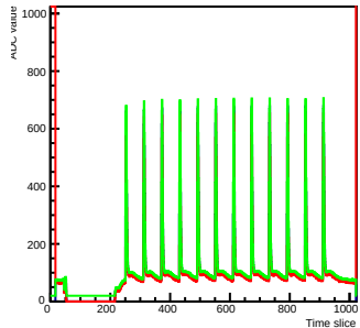
Run 2 Time mcm 0 chip 3 chan 15 s2-test4
