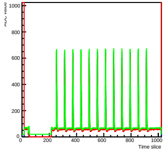
Run 2 Time mcm 0 chip 2 chan 9 s2-test4
