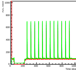
Run 2 Time mcm 0 chip 5 chan 7 s2-test4
