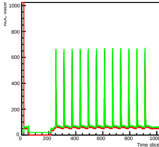
Run 2 Time mcm 0 chip 2 chan 11 s2-test4
