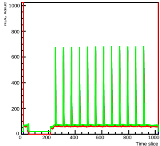
Run 2 Time mcm 0 chip 1 chan 13 s2-test4
