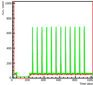
Run 2 Time mcm 0 chip 1 chan 15 s2-test4
