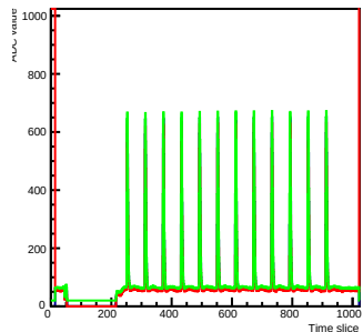
Run 2 Time mcm 0 chip 0 chan 9 s2-test4
