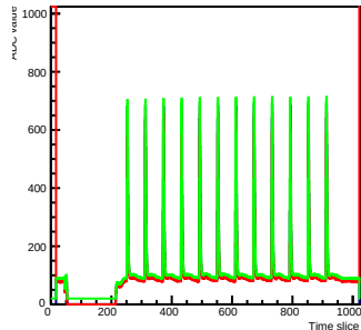
Run 2 Time mcm 0 chip 7 chan 13 s2-test4
