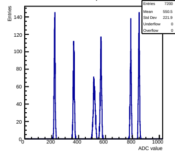
Pulse mcm 0 chip 4 chan 0 test
