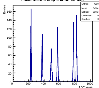
Pulse mcm 0 chip 6 chan 10 test
