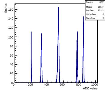
Pulse mcm 0 chip 1 chan 0 test
