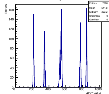
Pulse mcm 0 chip 1 chan 8 test
