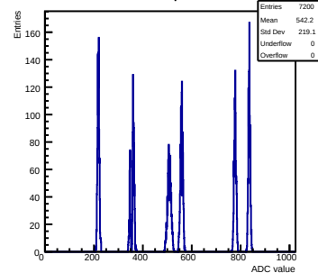
Pulse mcm 0 chip 4 chan 4 test
