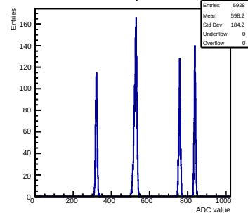
Pulse mcm 0 chip 1 chan 4 test
