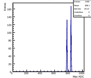
Max mcm 0 chip 4 chan 4 test
