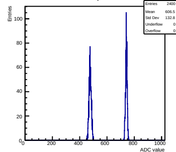
Pulse mcm 0 chip 7 chan 2 test
