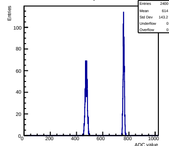
Pulse mcm 0 chip 7 chan 6 test
