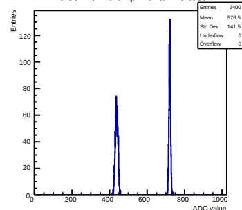
Pulse mcm 0 chip 7 chan 10 test
