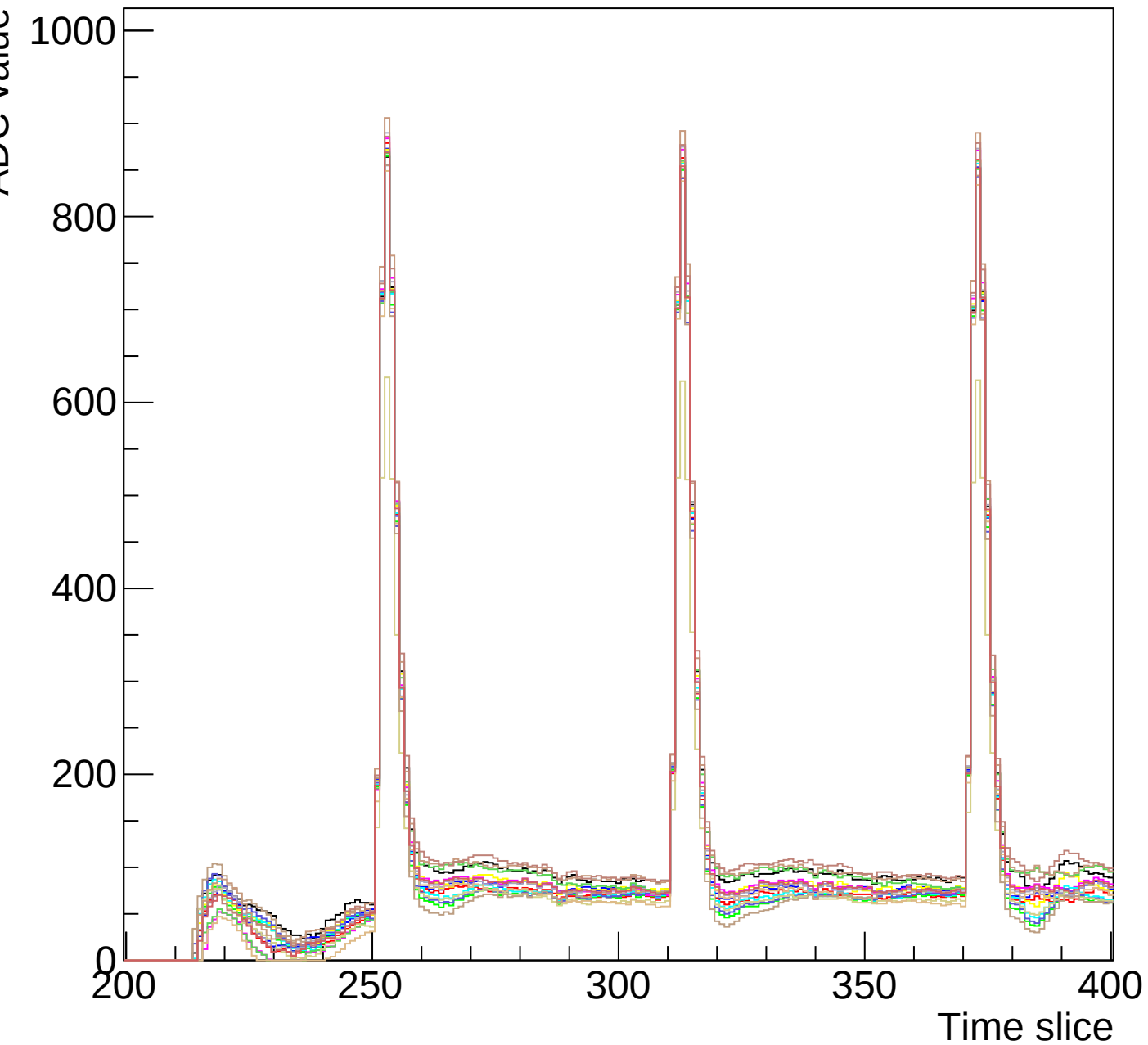
Run 0 event 10 mcm 0 chip 7 clk0-s3-zoom
