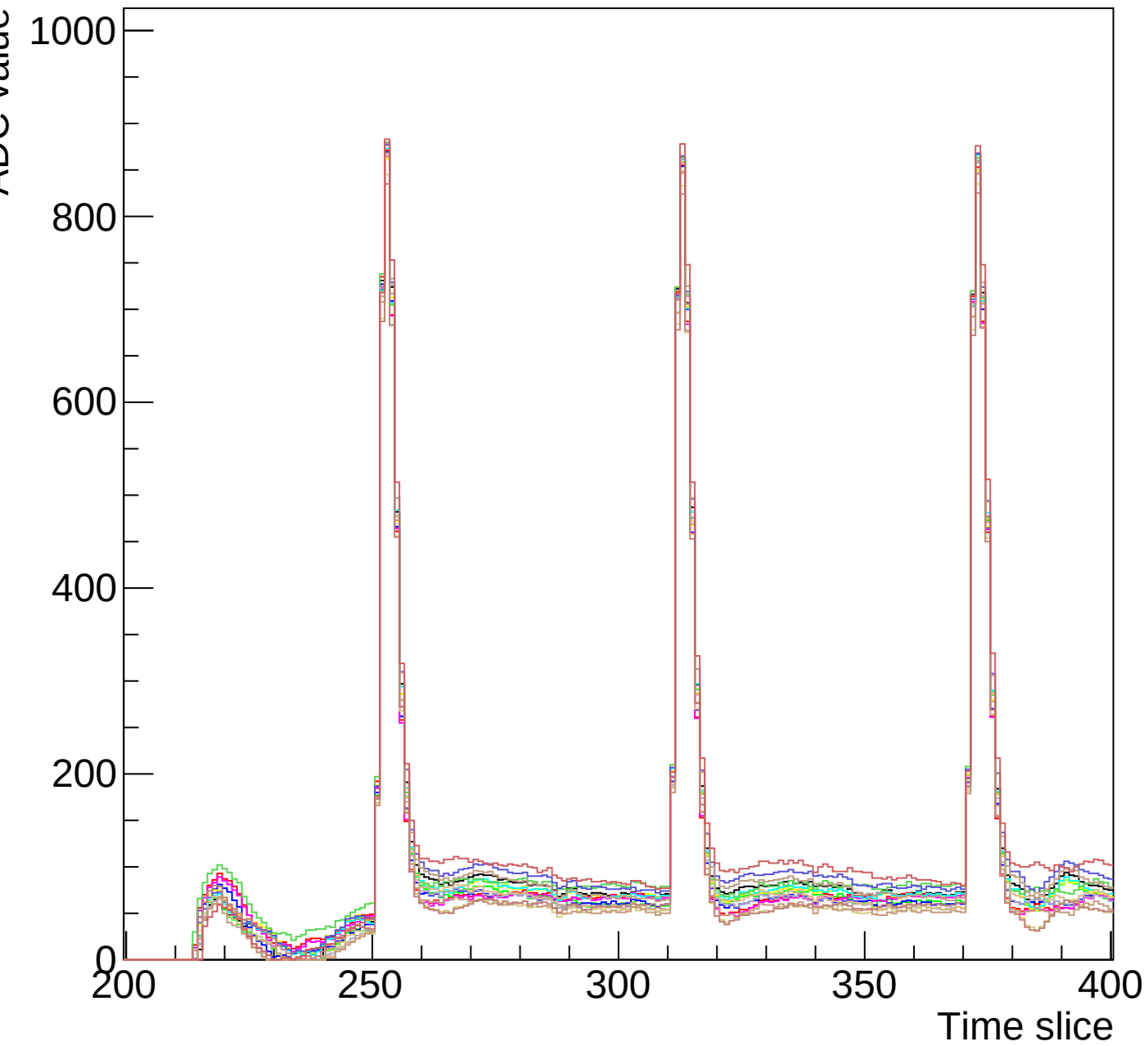
Run 0 event 10 mcm 0 chip 3 clk0-s3-zoom
