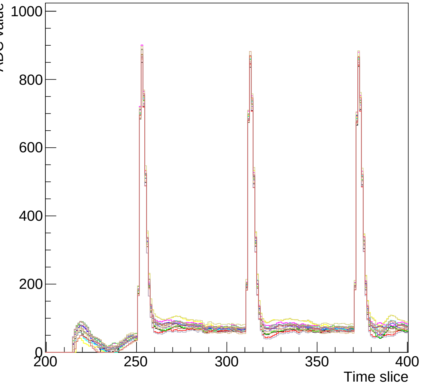
Run 0 event 10 mcm 0 chip 2 clk0-s3-zoom
