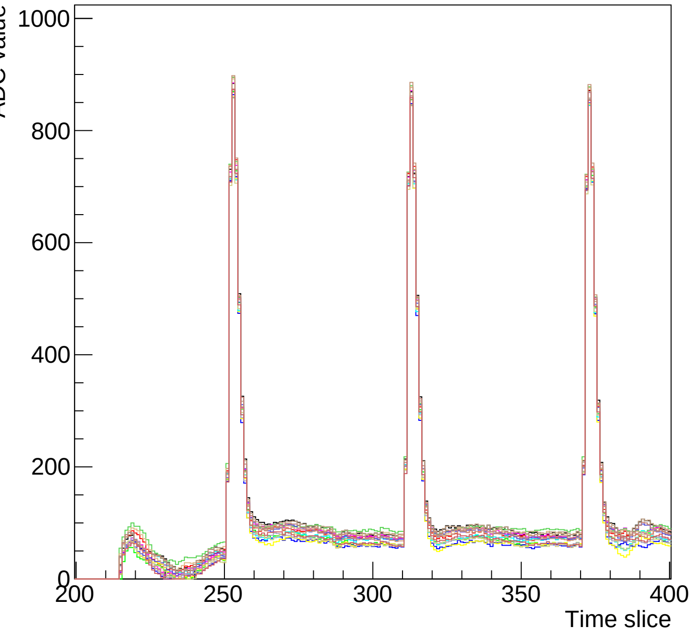
Run 0 event 10 mcm 0 chip 5 clk0-s3-zoom
