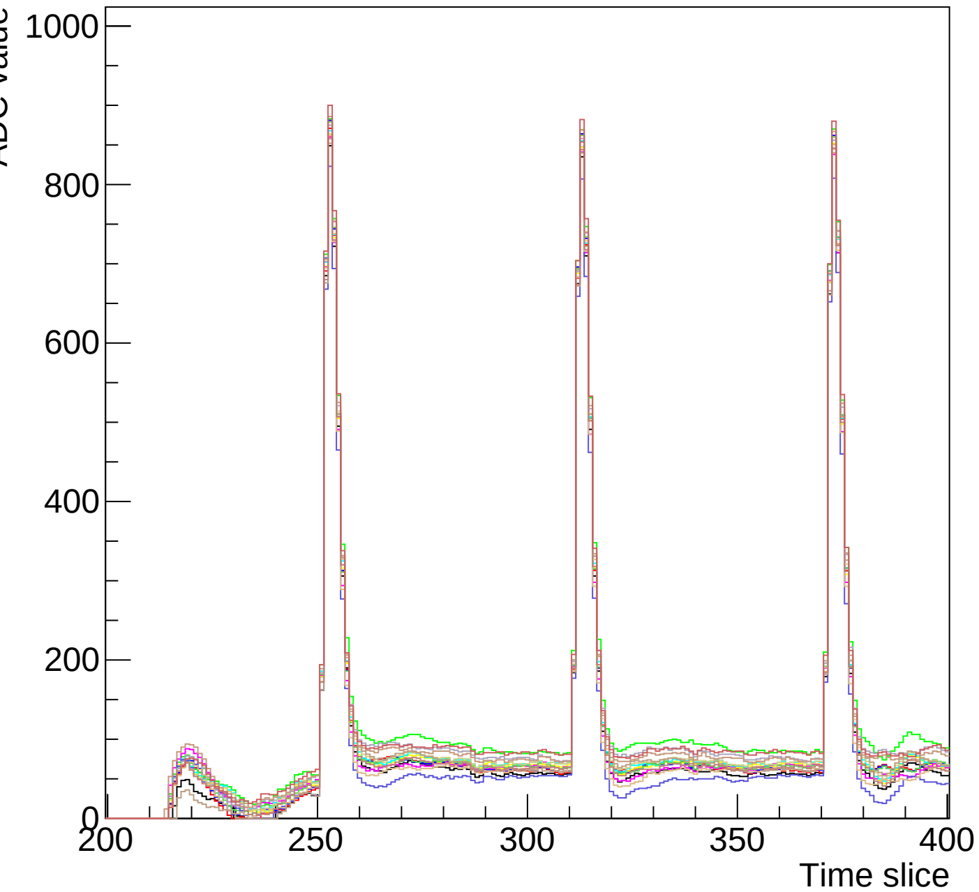
Run 0 event 10 mcm 0 chip 6 clk0-s3-zoom
