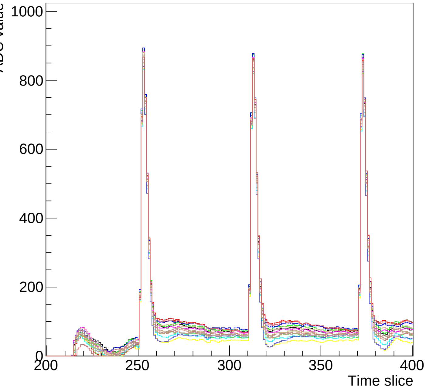
Run 0 event 10 mcm 0 chip 0 clk0-s3-zoom
