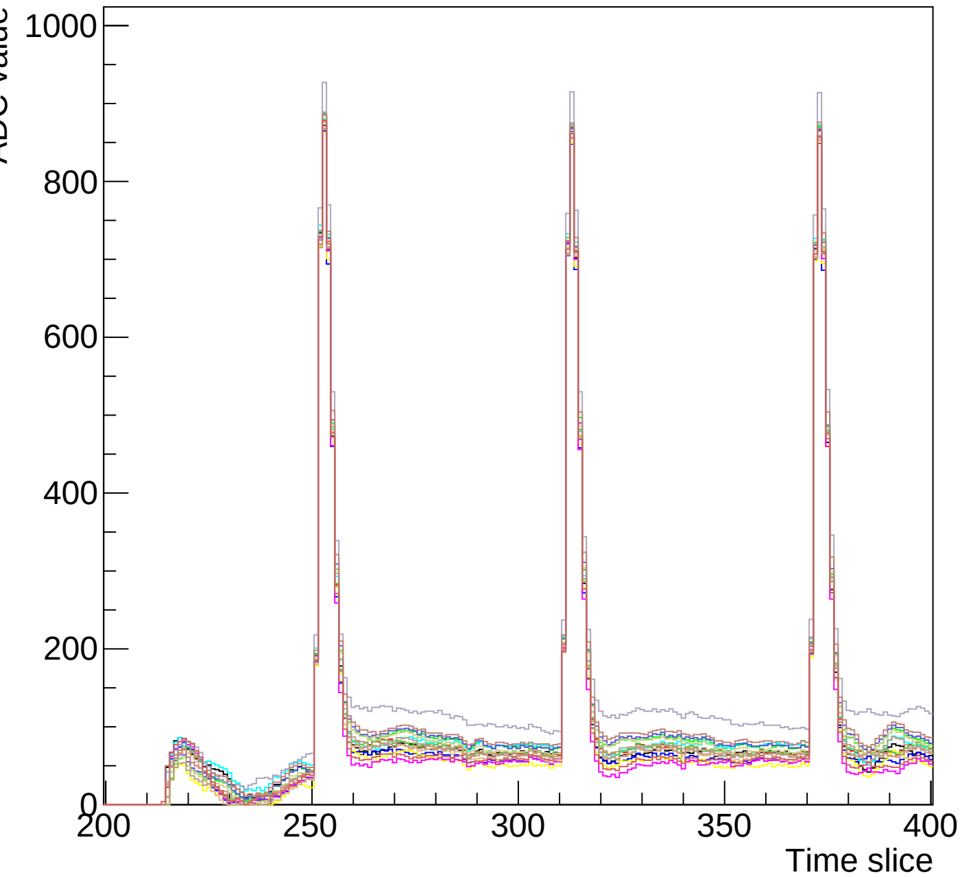
Run 0 event 10 mcm 0 chip 1 clk0-s3-zoom
