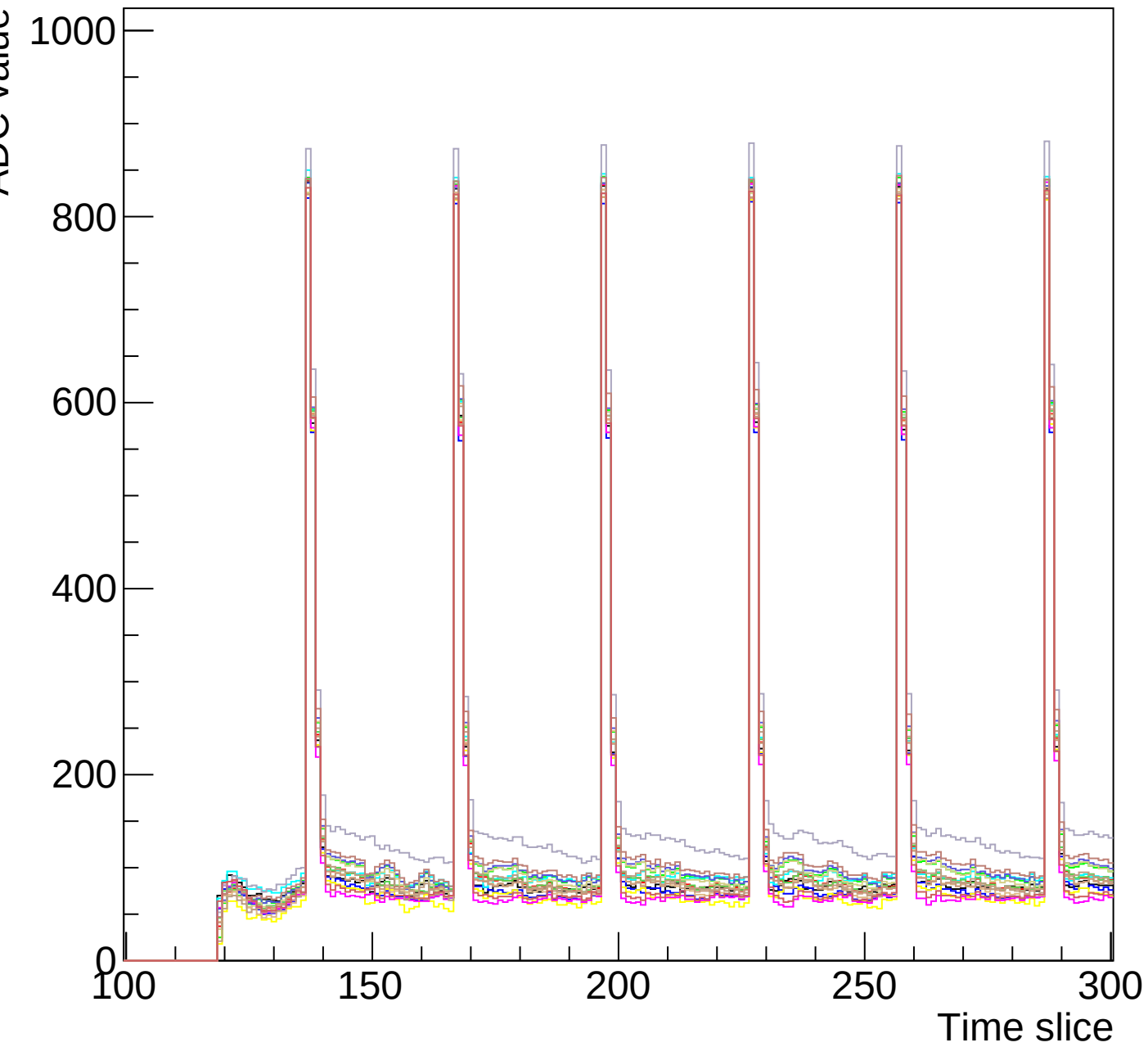
Run 1 event 10 mcm 0 chip 1 clk1-s3-zoom
