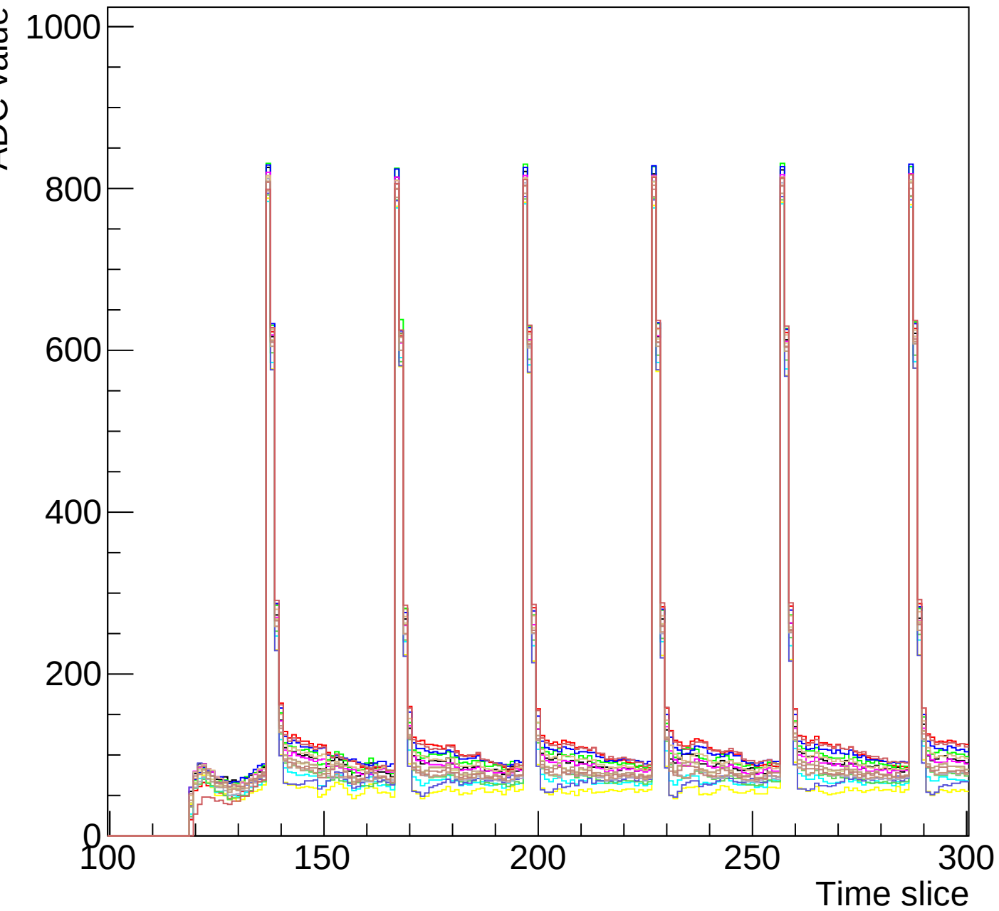
Run 1 event 10 mcm 0 chip 0 clk1-s3-zoom
