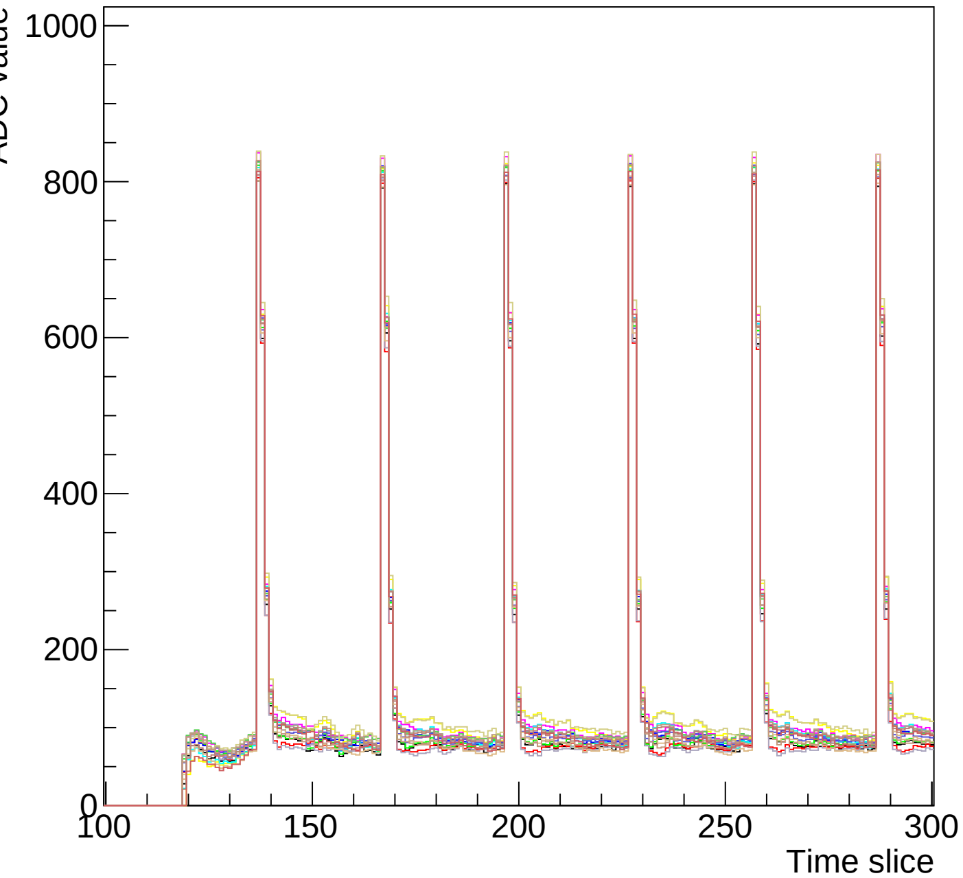
Run 1 event 10 mcm 0 chip 2 clk1-s3-zoom
