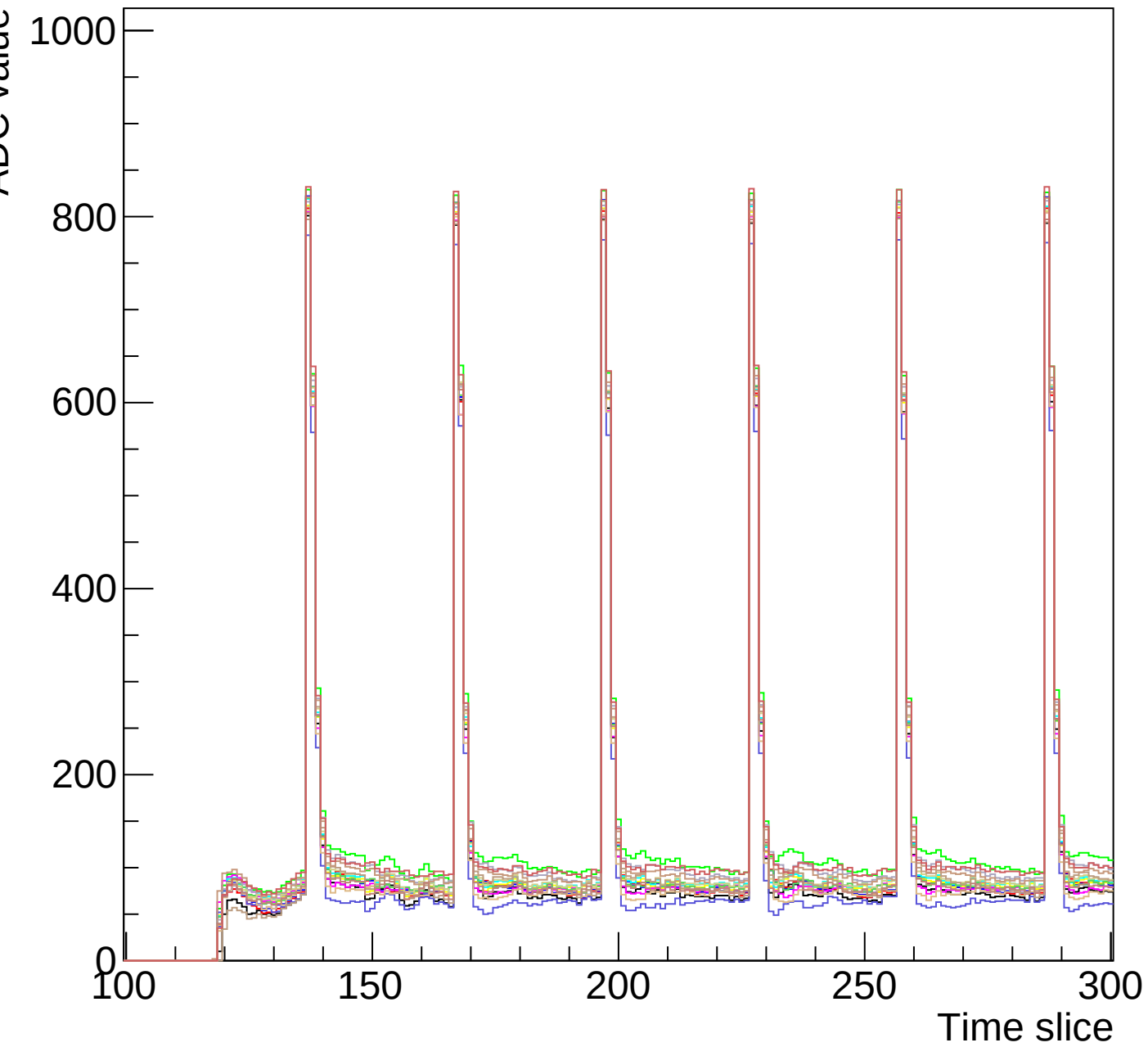
Run 1 event 10 mcm 0 chip 6 clk1-s3-zoom
