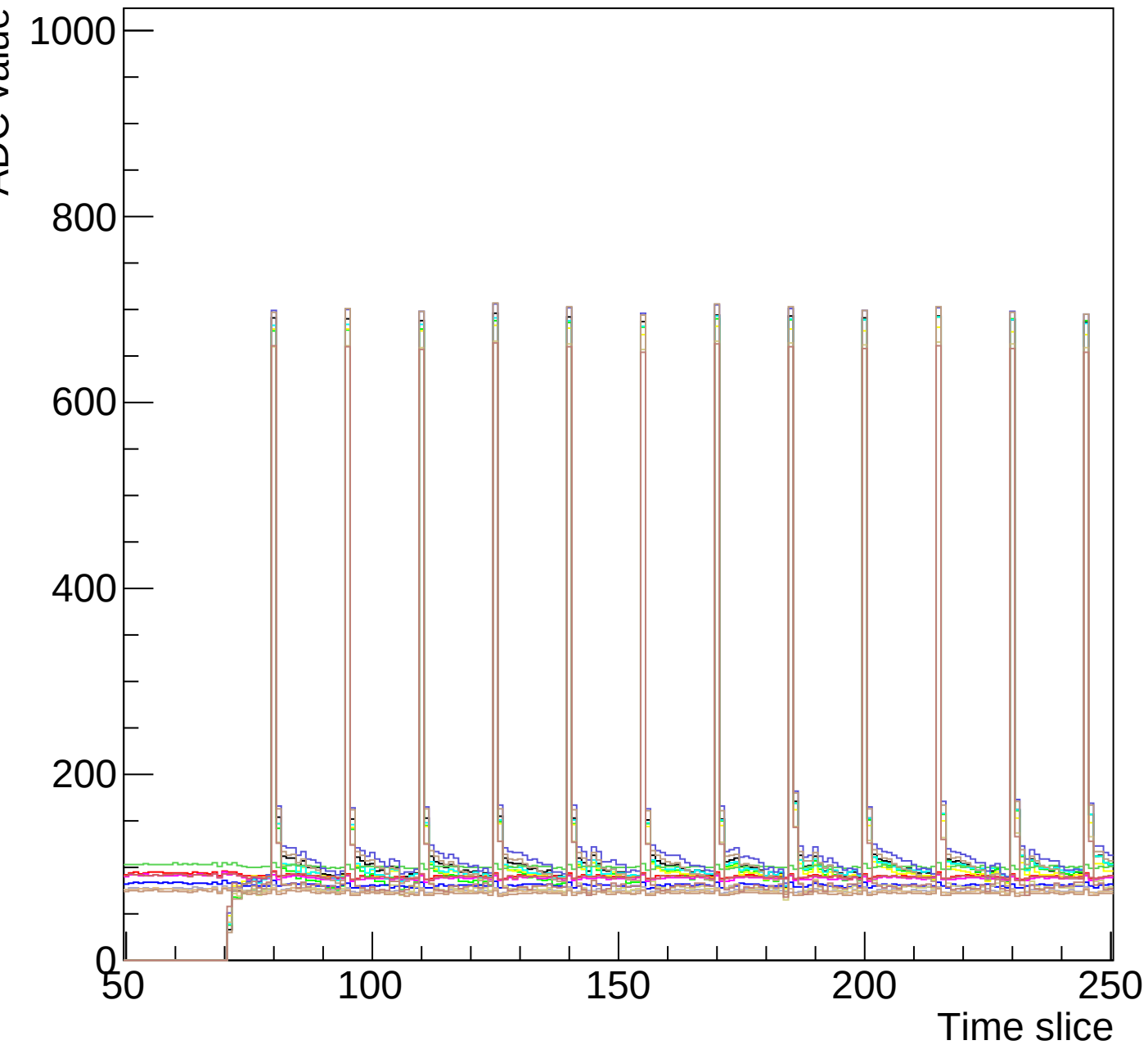
Run 4 event 2 mcm 0 chip 3 clk2-s1-zoom
