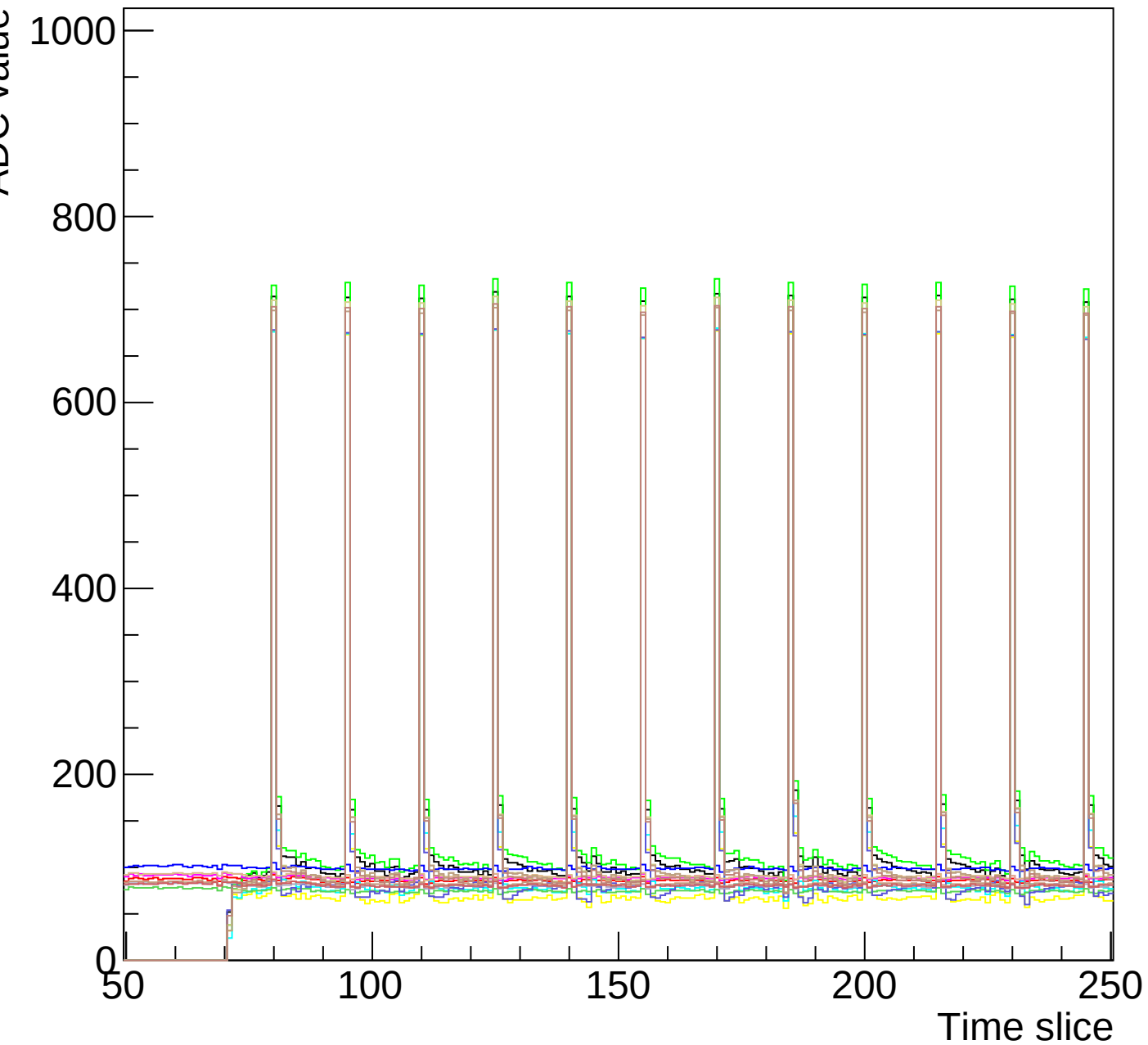
Run 4 event 2 mcm 0 chip 0 clk2-s1-zoom
