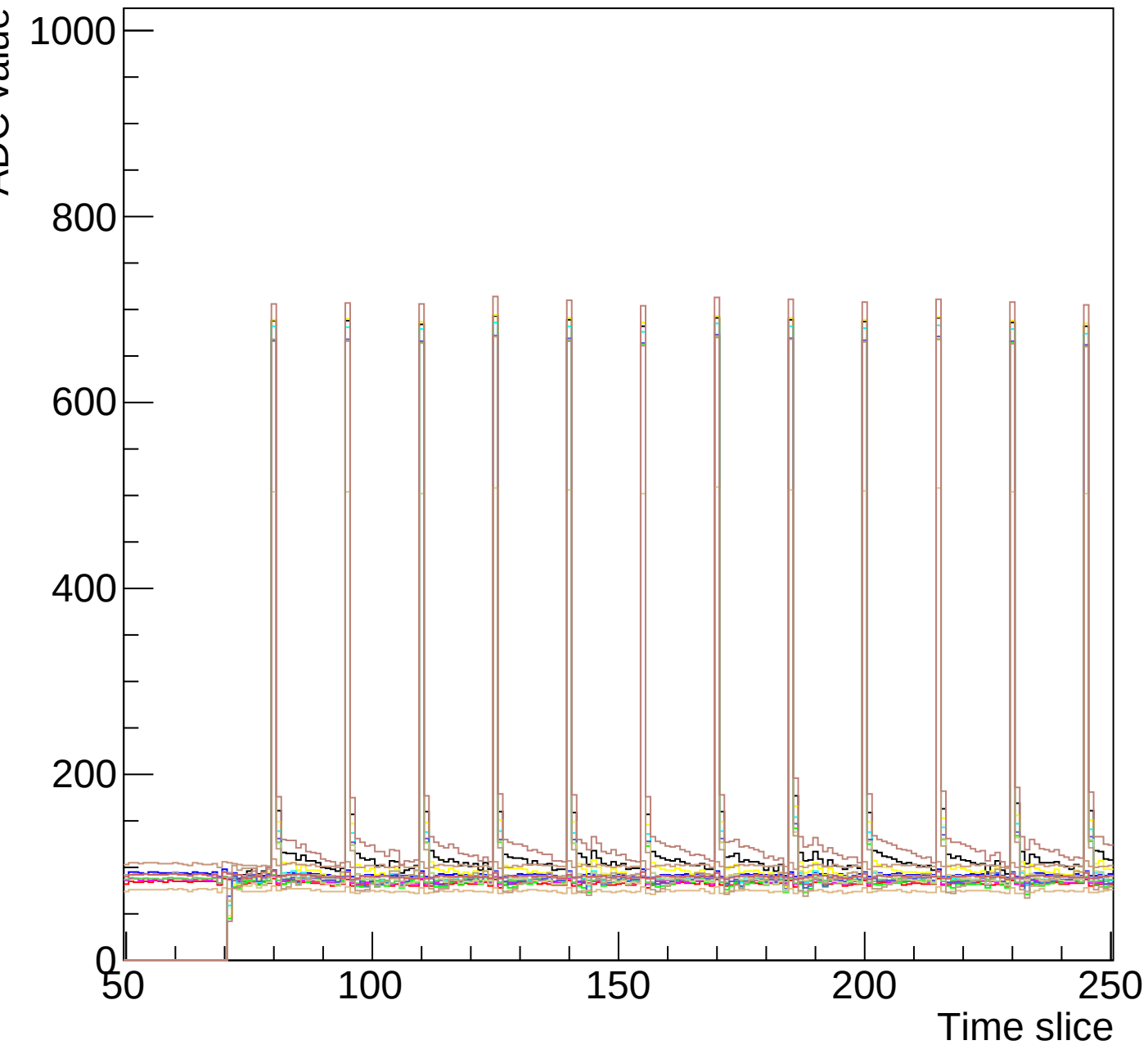
Run 4 event 2 mcm 0 chip 7 clk2-s1-zoom
