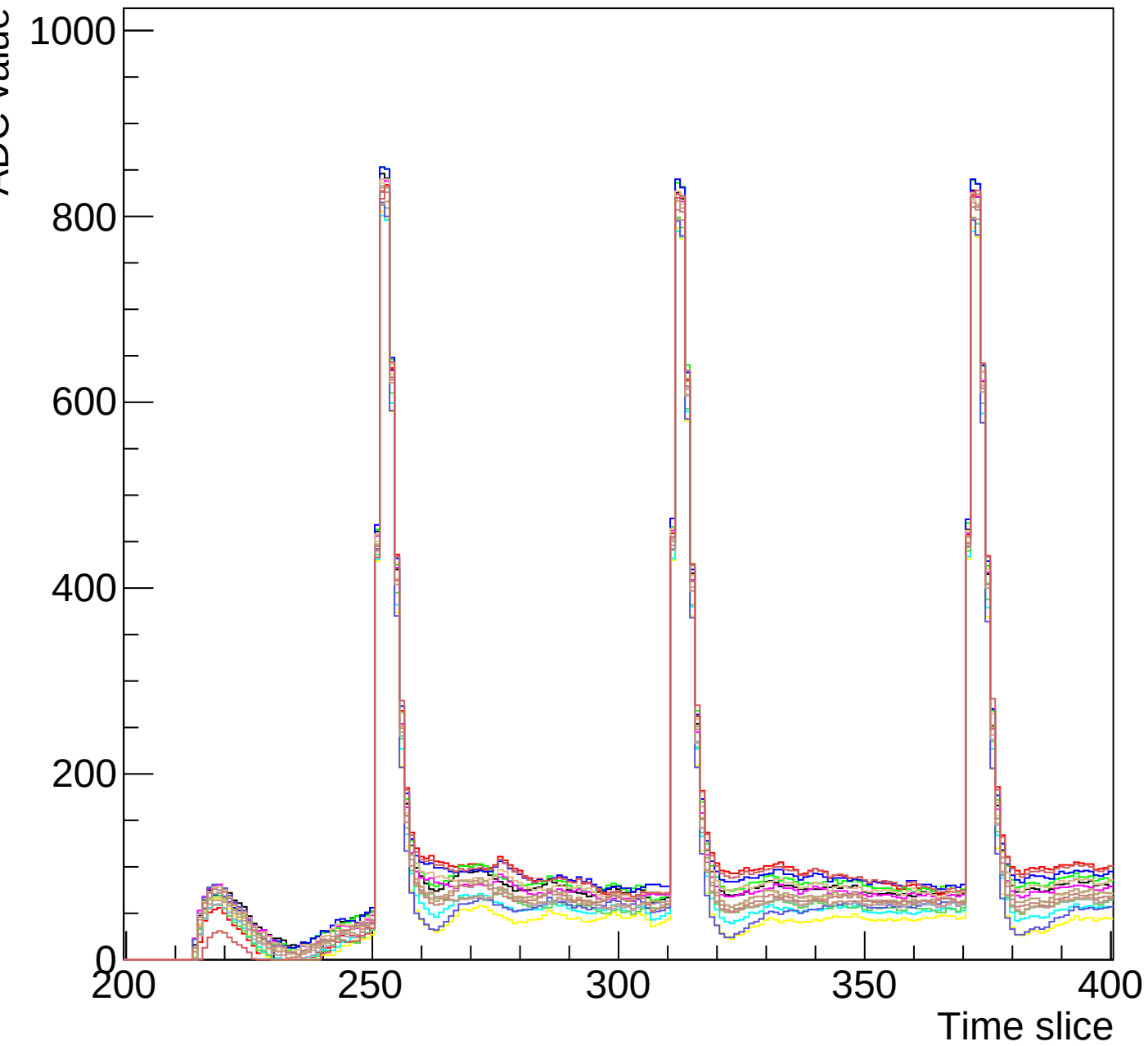
Run 0 event 5 mcm 0 chip 0 clk0-s3-zoom
