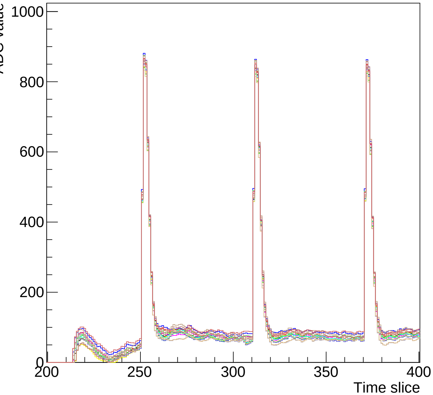
Run 0 event 5 mcm 0 chip 4 clk0-s3-zoom
