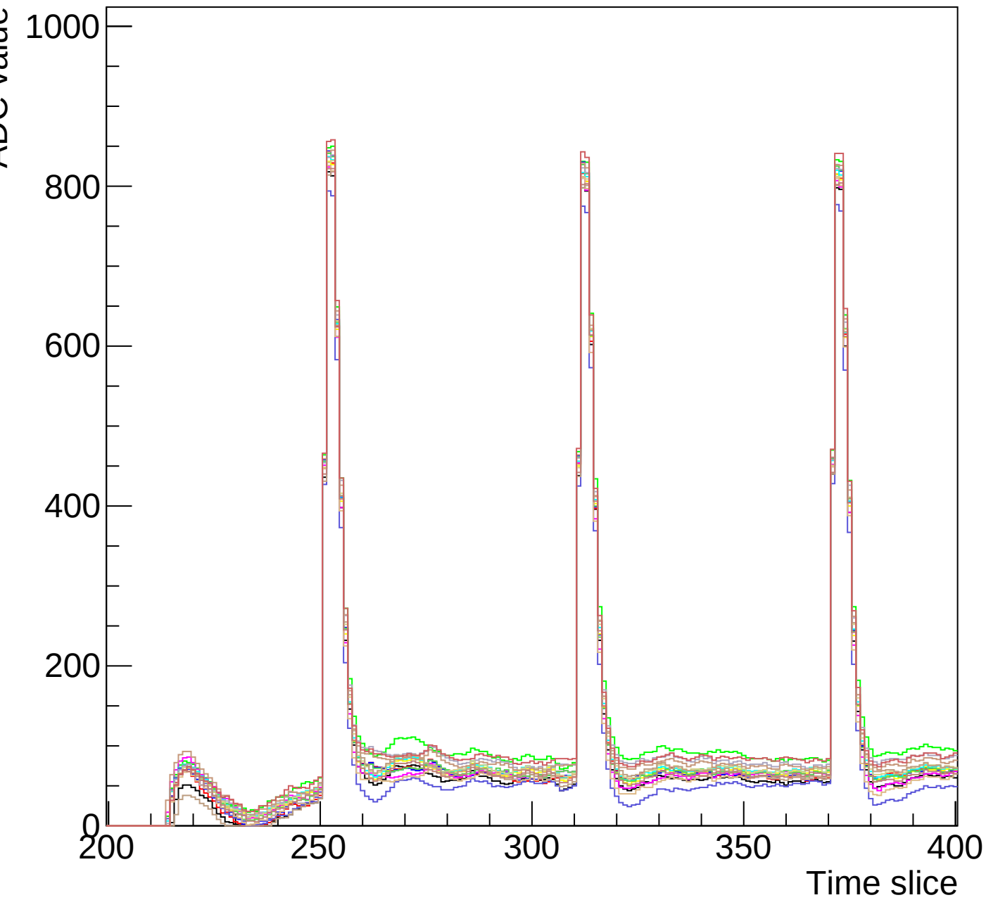
Run 0 event 5 mcm 0 chip 6 clk0-s3-zoom
