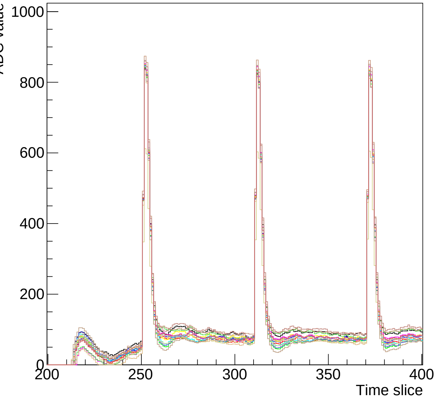
Run 0 event 5 mcm 0 chip 7 clk0-s3-zoom
