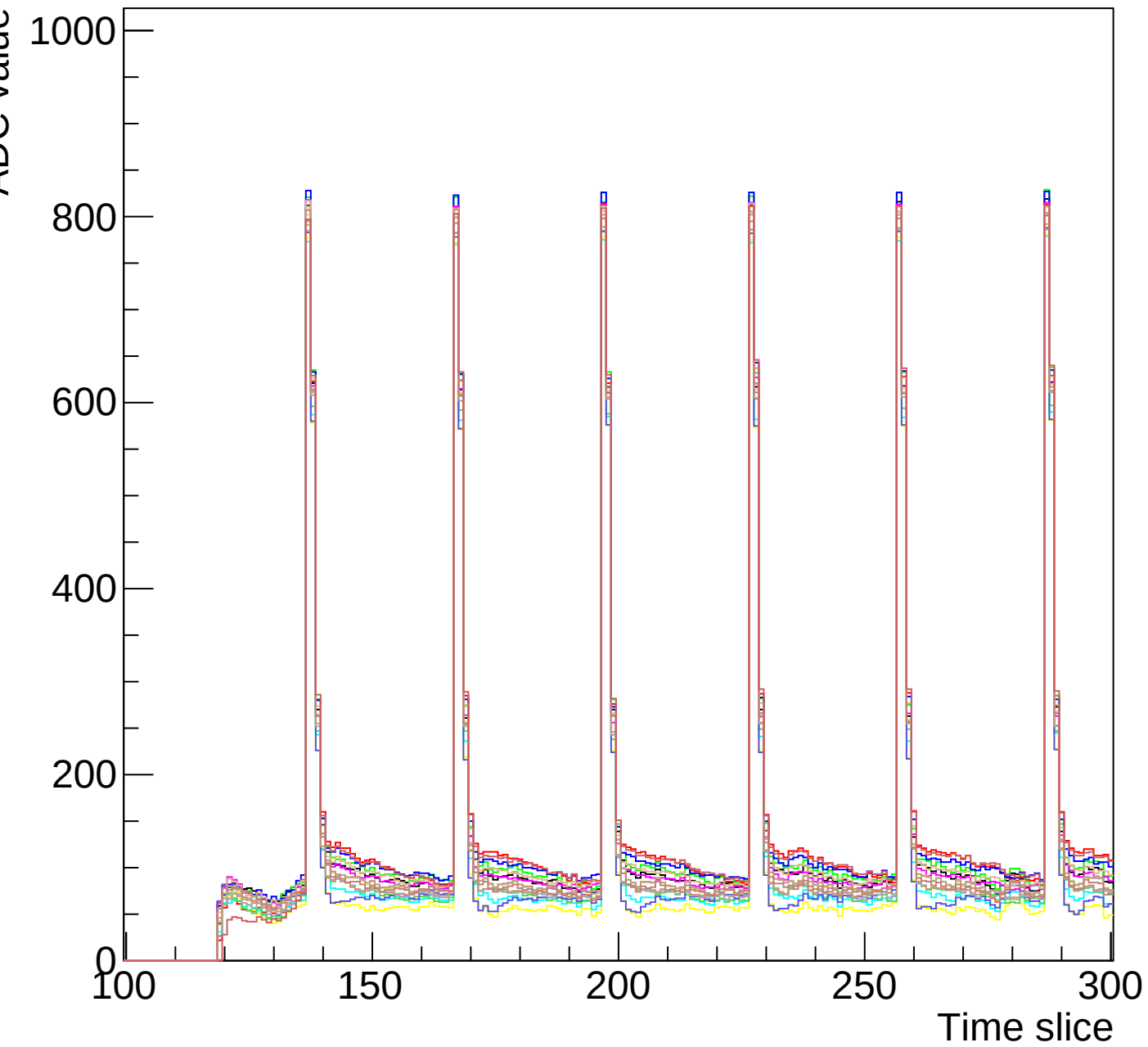
Run 1 event 5 mcm 0 chip 0 clk1-s3-zoom
