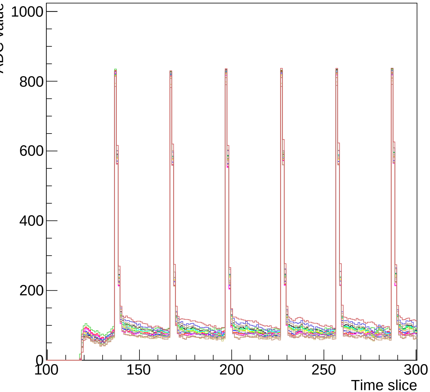
Run 1 event 5 mcm 0 chip 3 clk1-s3-zoom
