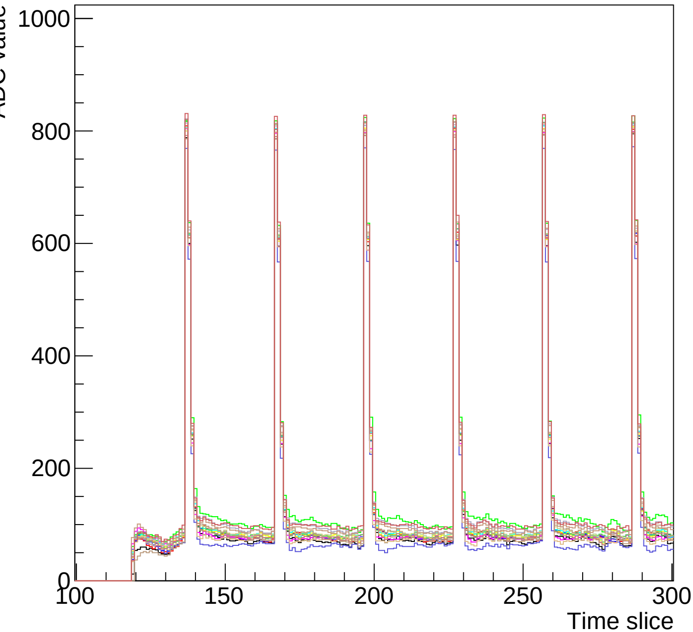
Run 1 event 5 mcm 0 chip 6 clk1-s3-zoom
