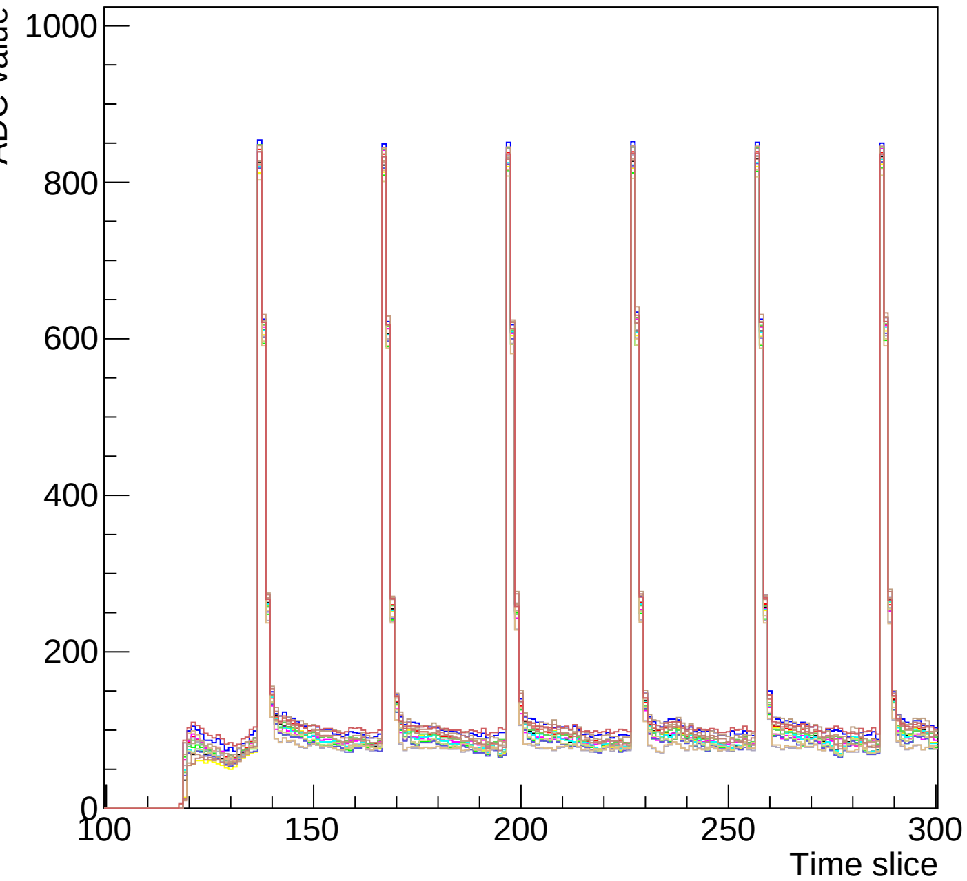
Run 1 event 5 mcm 0 chip 4 clk1-s3-zoom
