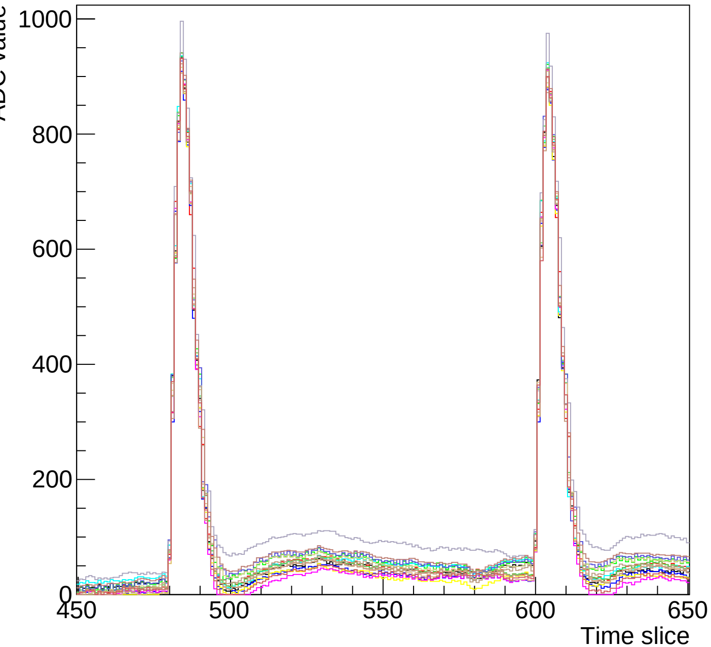
Run 3 event 5 mcm 0 chip 1 clk3-s3-zoom1
