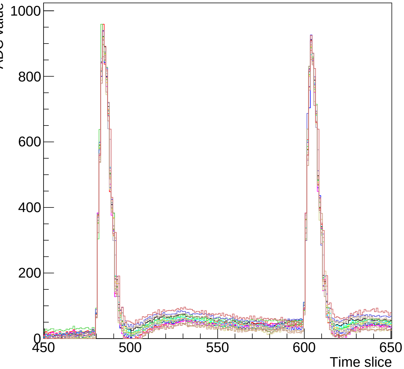
Run 3 event 5 mcm 0 chip 3 clk3-s3-zoom1
