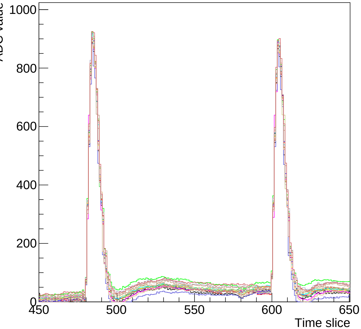
Run 3 event 5 mcm 0 chip 6 clk3-s3-zoom1
