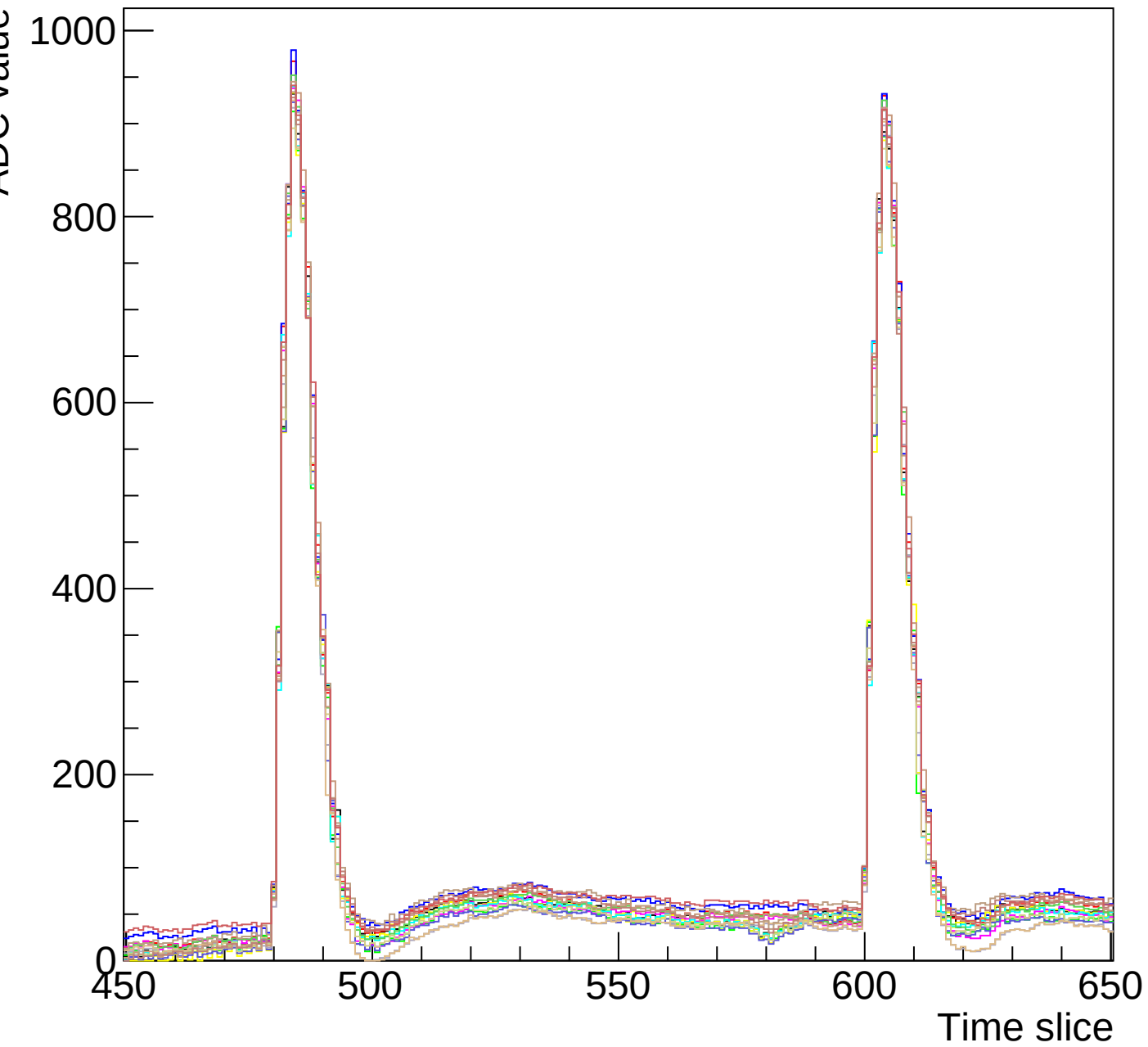
Run 3 event 5 mcm 0 chip 4 clk3-s3-zoom1
