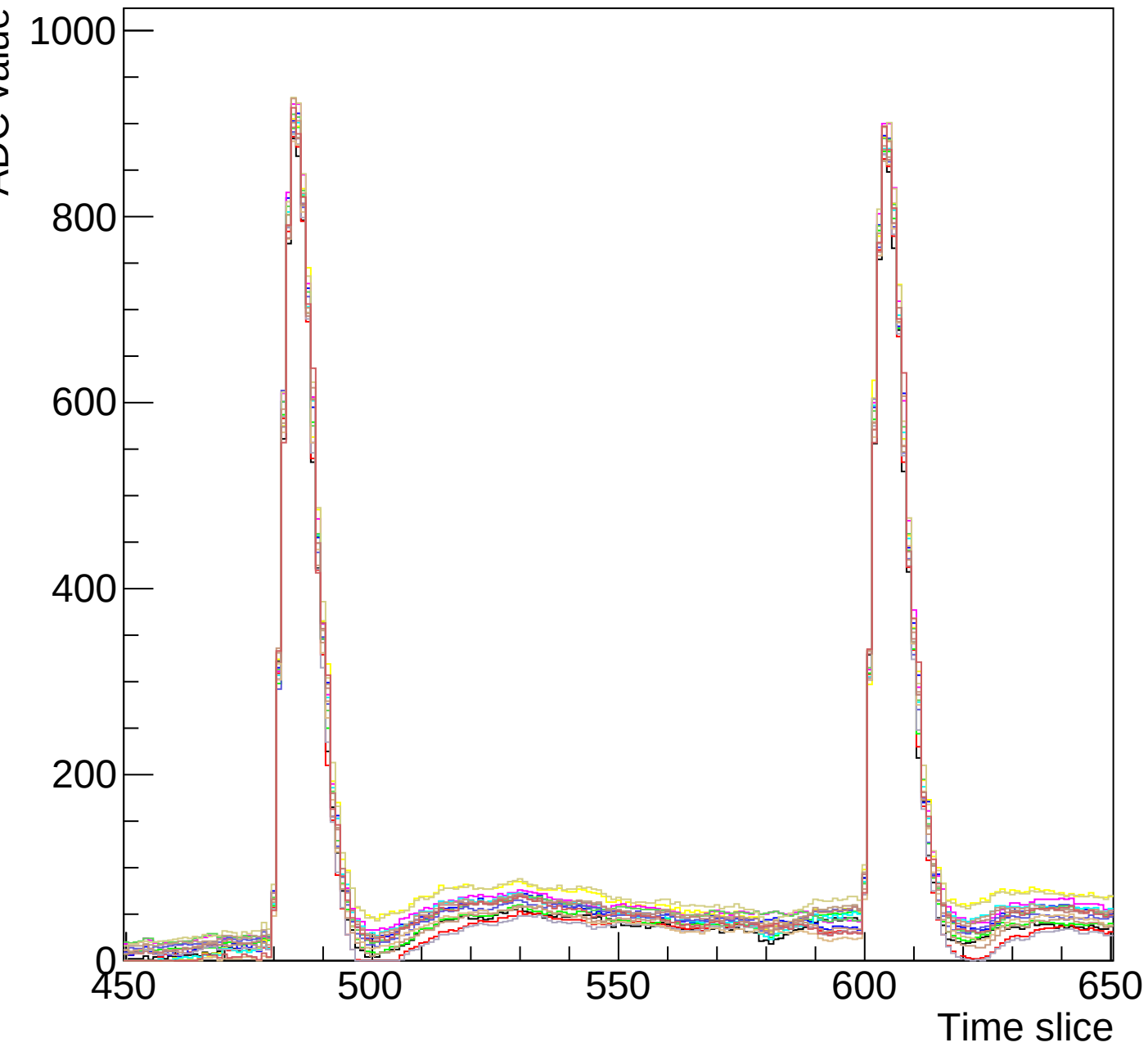
Run 3 event 5 mcm 0 chip 2 clk3-s3-zoom1
