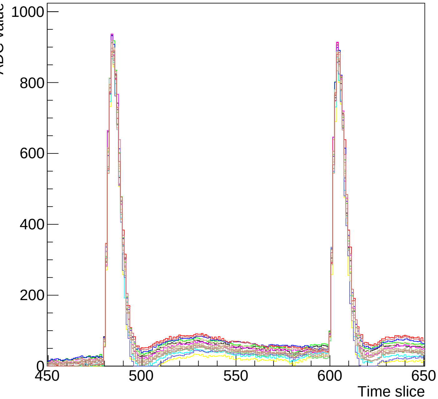
Run 3 event 5 mcm 0 chip 0 clk3-s3-zoom1
