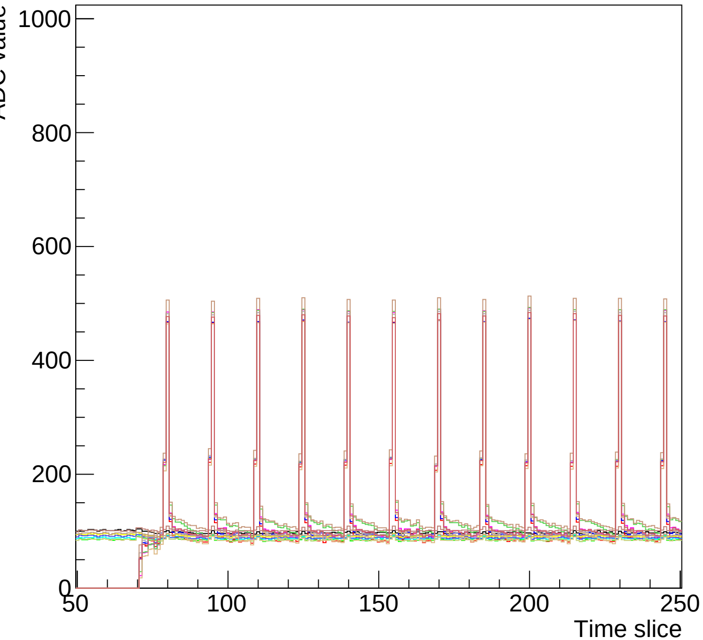
Run 5 event 5 mcm 0 chip 7 clk2-s2-zoom
