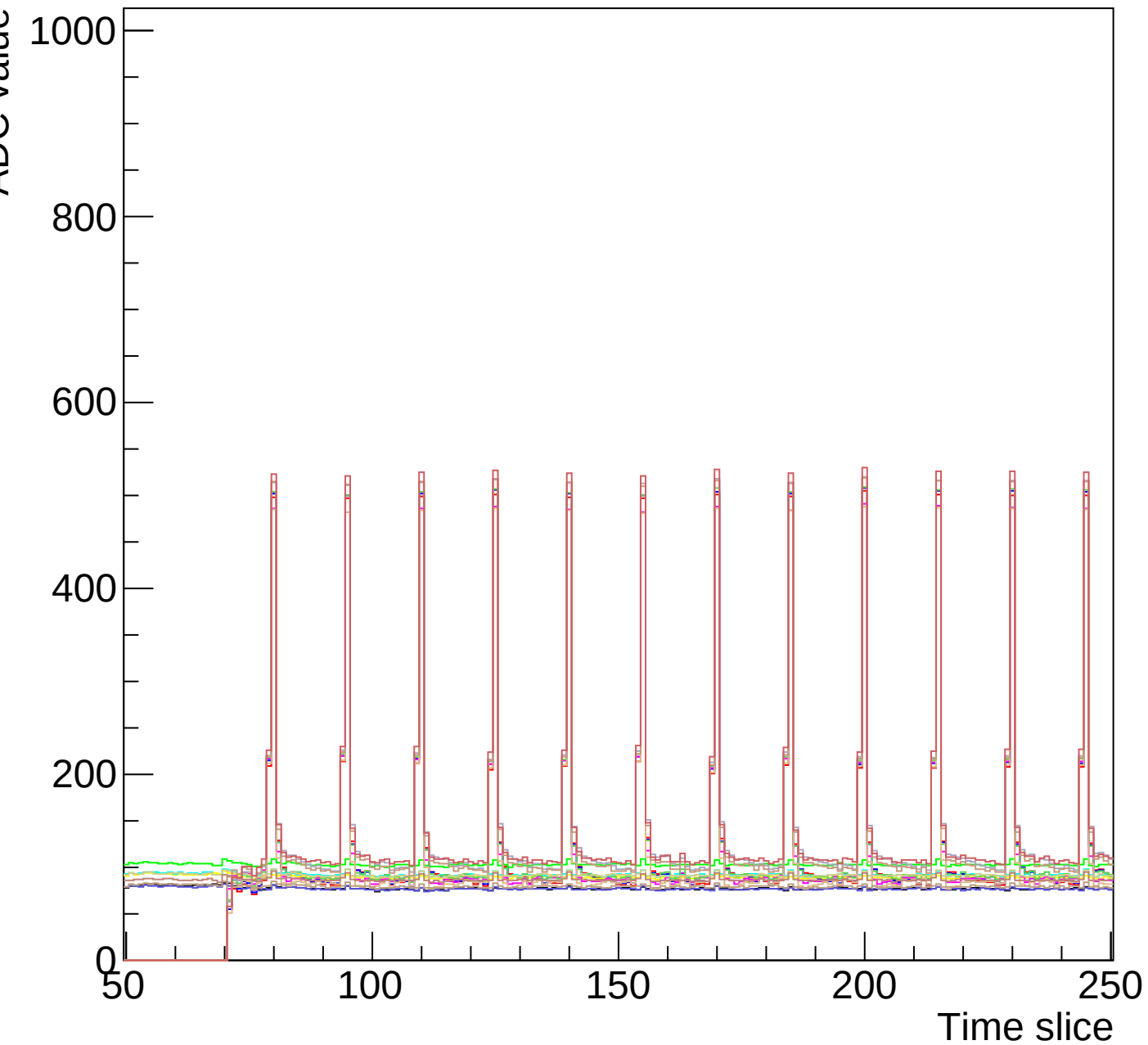
Run 5 event 5 mcm 0 chip 6 clk2-s2-zoom
