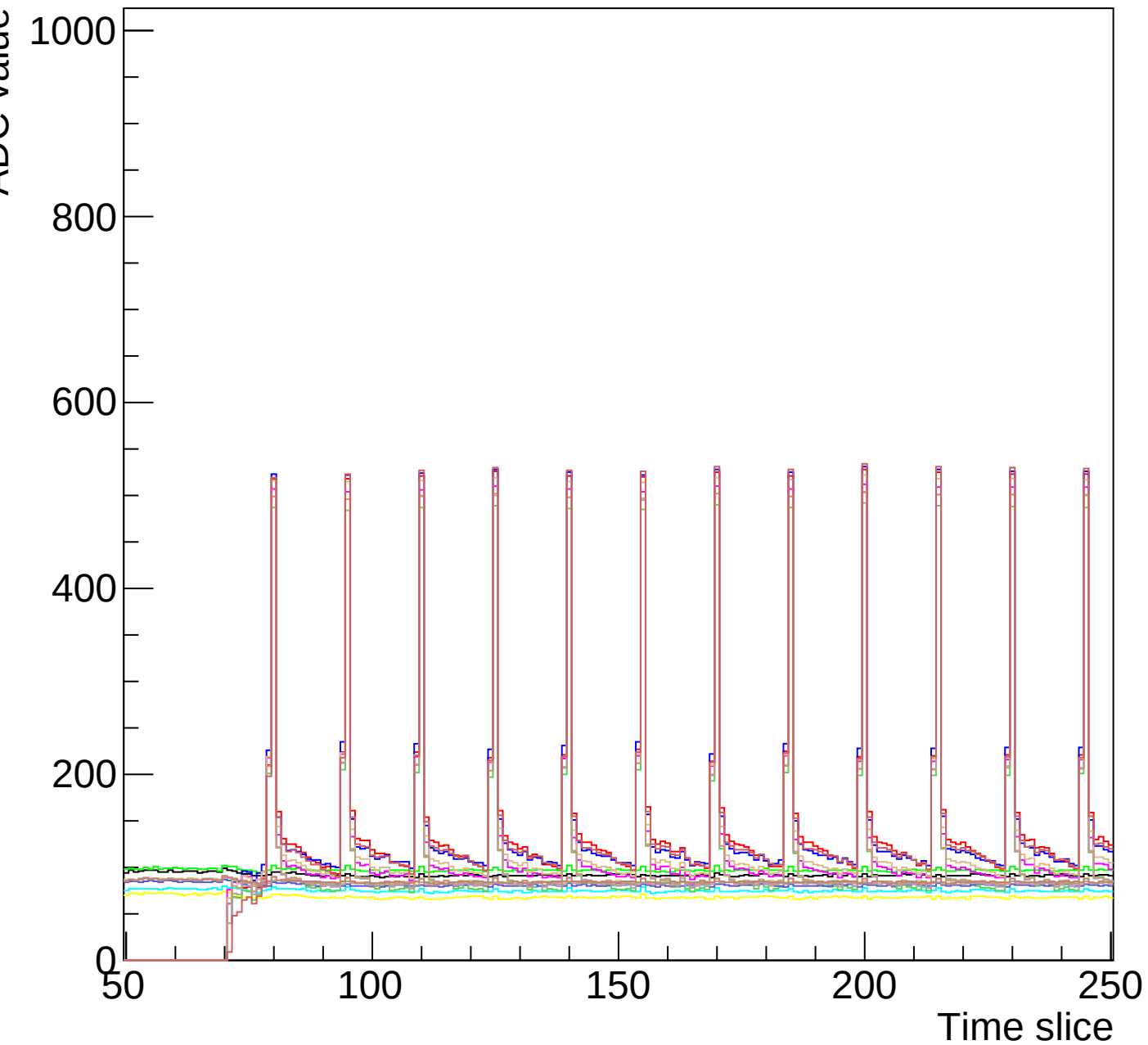
Run 5 event 5 mcm 0 chip 0 clk2-s2-zoom
