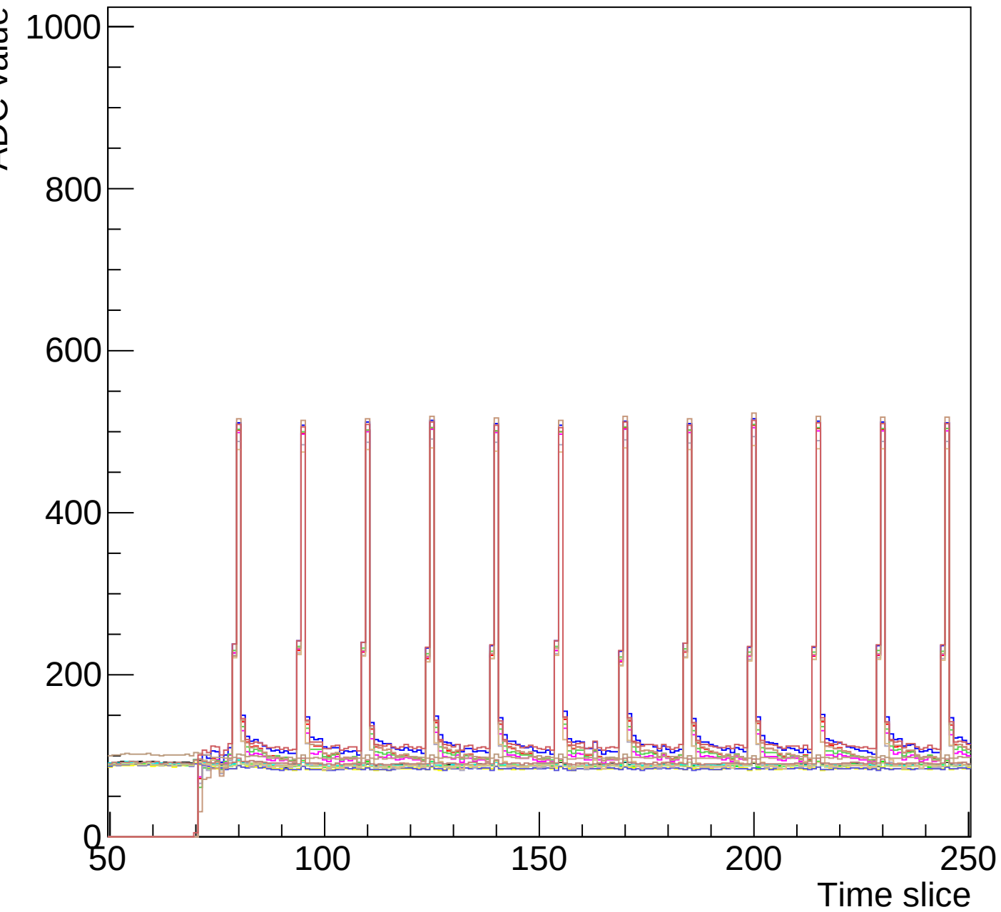
Run 5 event 5 mcm 0 chip 4 clk2-s2-zoom
