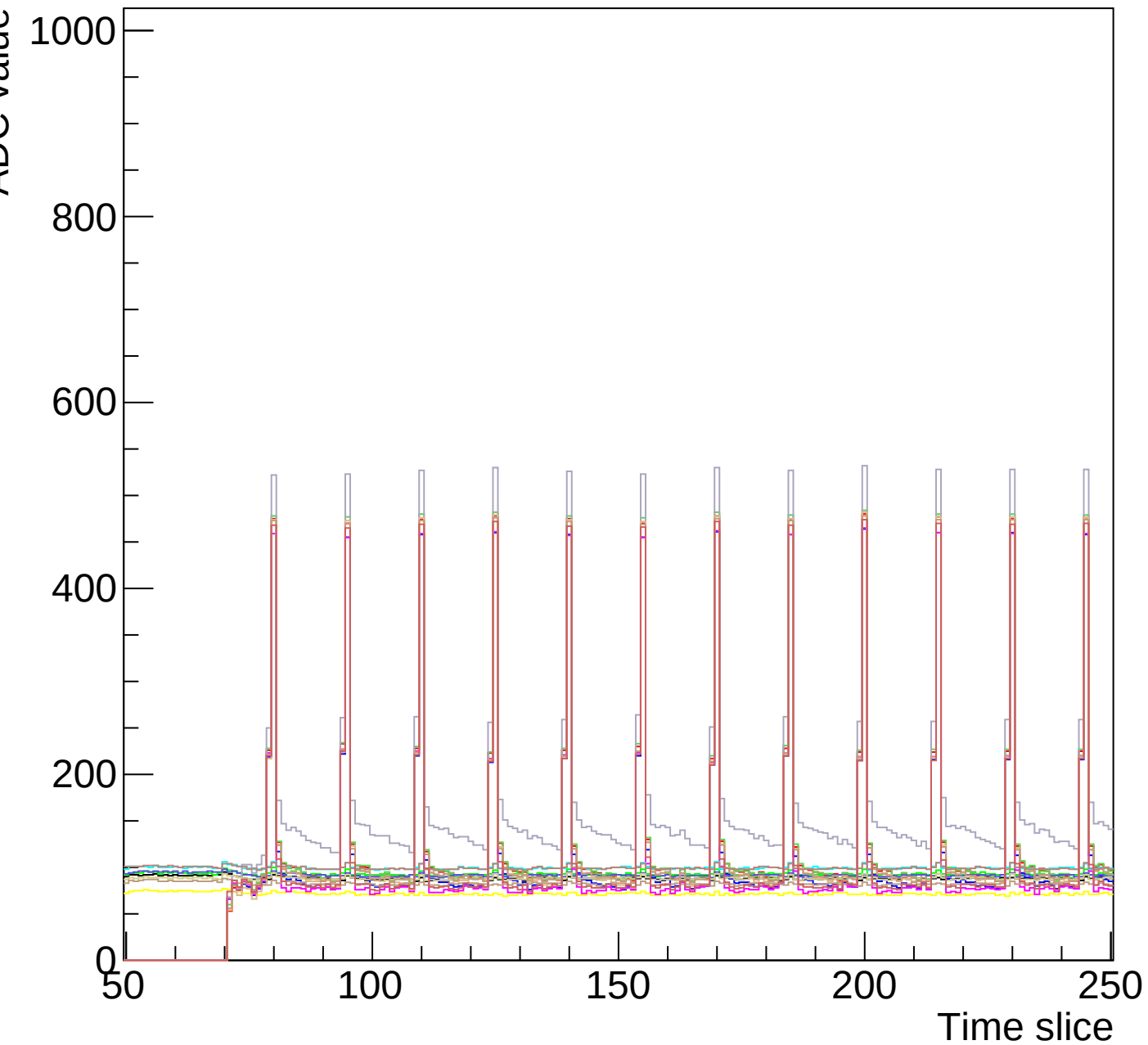
Run 5 event 5 mcm 0 chip 1 clk2-s2-zoom
