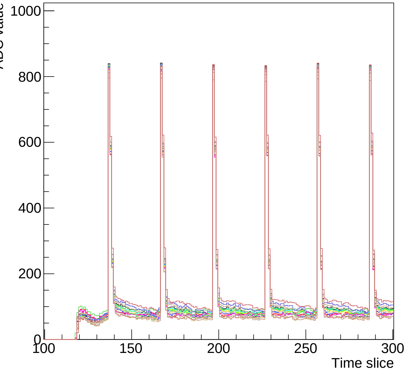
Run 1 event 6 mcm 0 chip 3 clk1-s3-zoom
