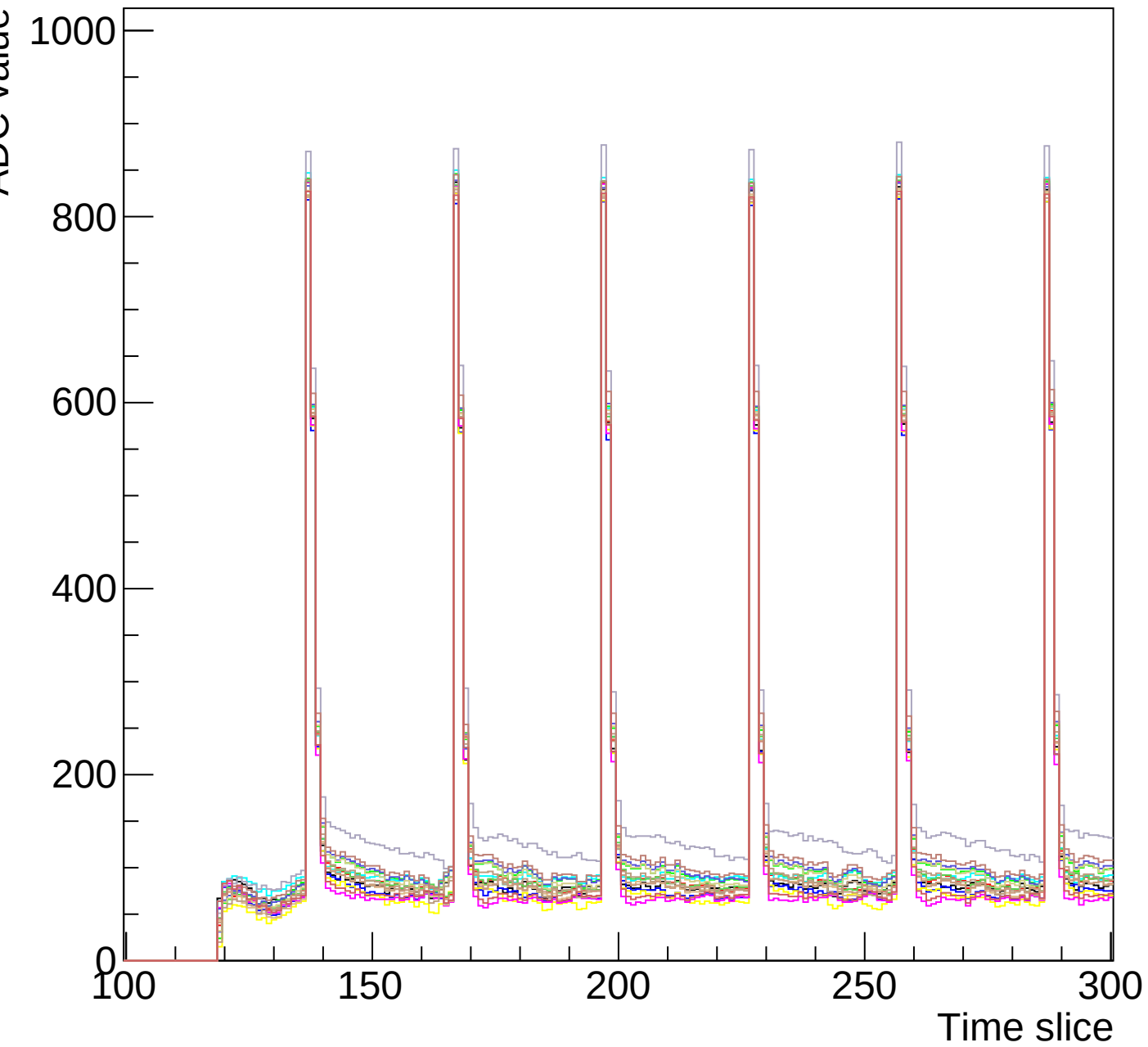
Run 1 event 6 mcm 0 chip 1 clk1-s3-zoom
