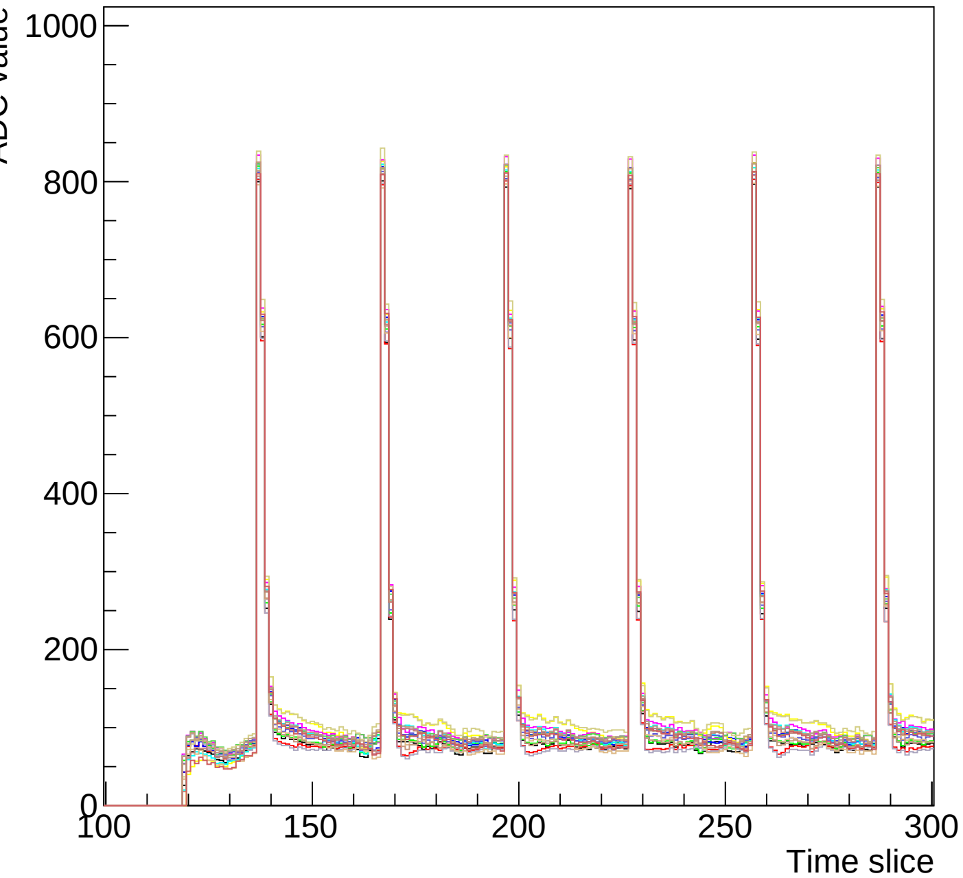
Run 1 event 6 mcm 0 chip 2 clk1-s3-zoom
