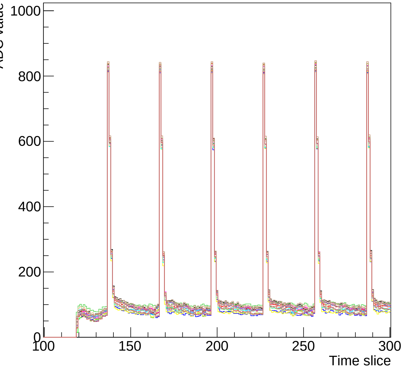
Run 1 event 6 mcm 0 chip 5 clk1-s3-zoom
