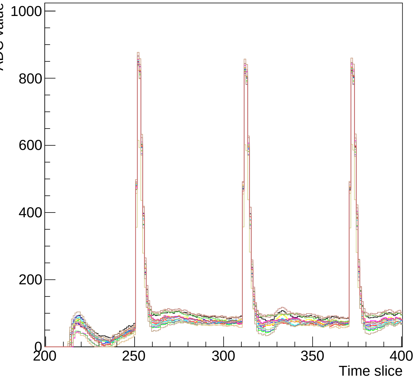
Run 0 event 7 mcm 0 chip 7 clk0-s3-zoom
