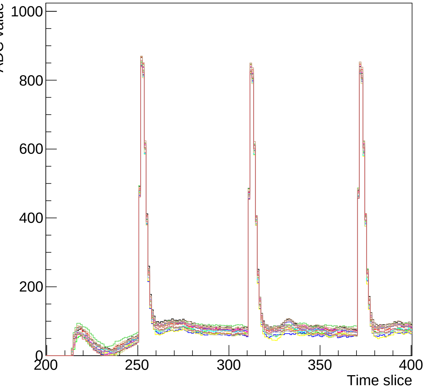
Run 0 event 7 mcm 0 chip 5 clk0-s3-zoom
