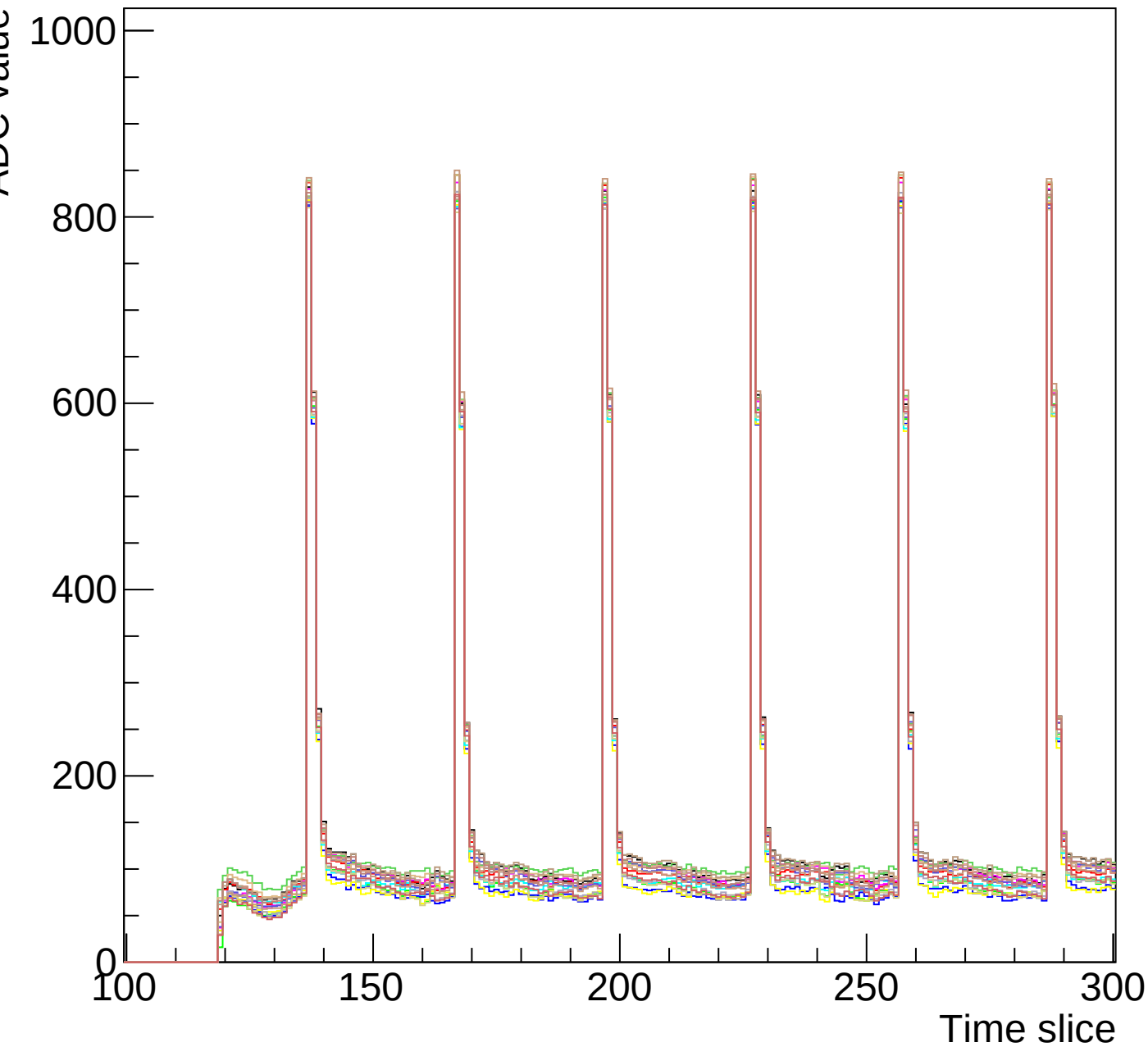
Run 1 event 7 mcm 0 chip 5 clk1-s3-zoom
