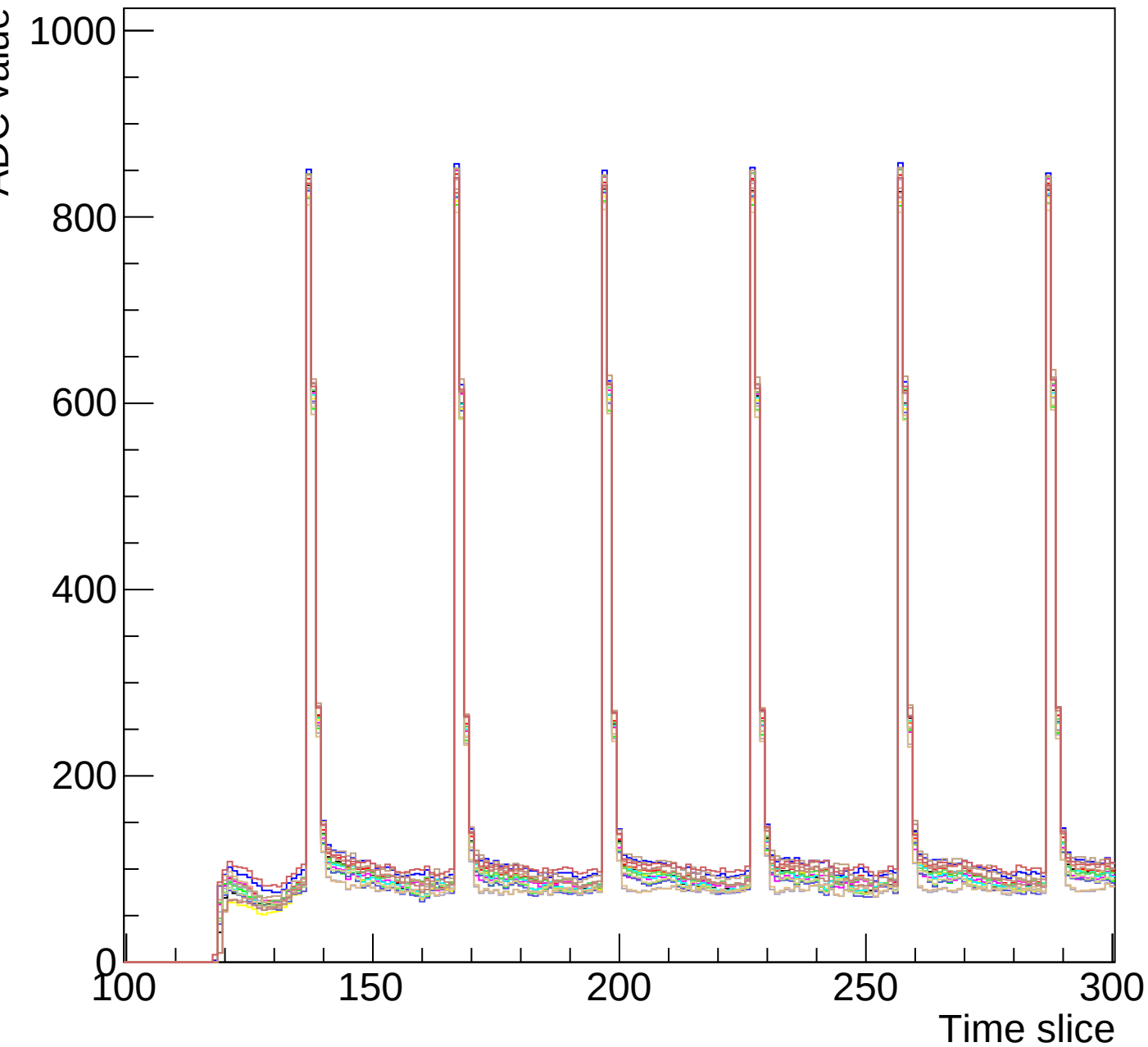
Run 1 event 7 mcm 0 chip 4 clk1-s3-zoom
