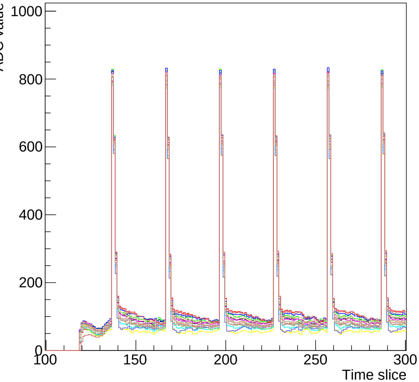
Run 1 event 7 mcm 0 chip 0 clk1-s3-zoom
