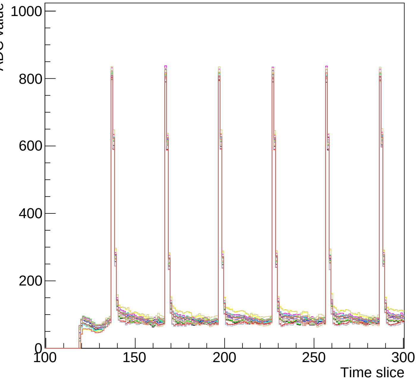
Run 1 event 7 mcm 0 chip 2 clk1-s3-zoom
