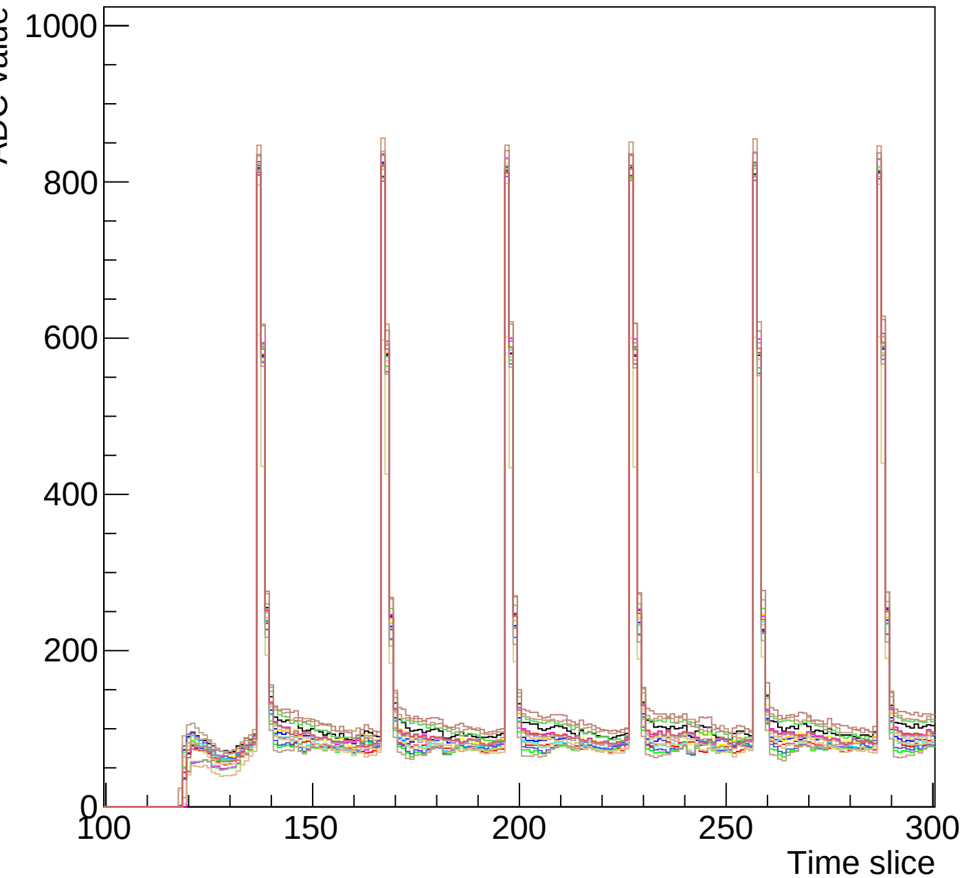
Run 1 event 7 mcm 0 chip 7 clk1-s3-zoom
