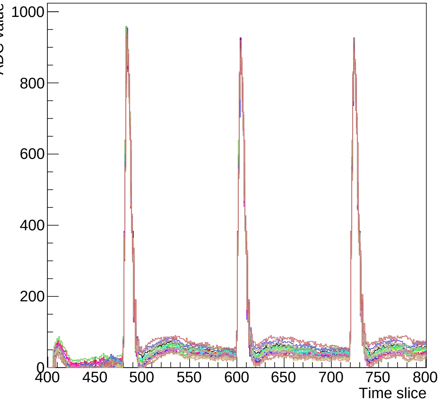
Run 3 event 7 mcm 0 chip 3 clk3-s3-zoom
