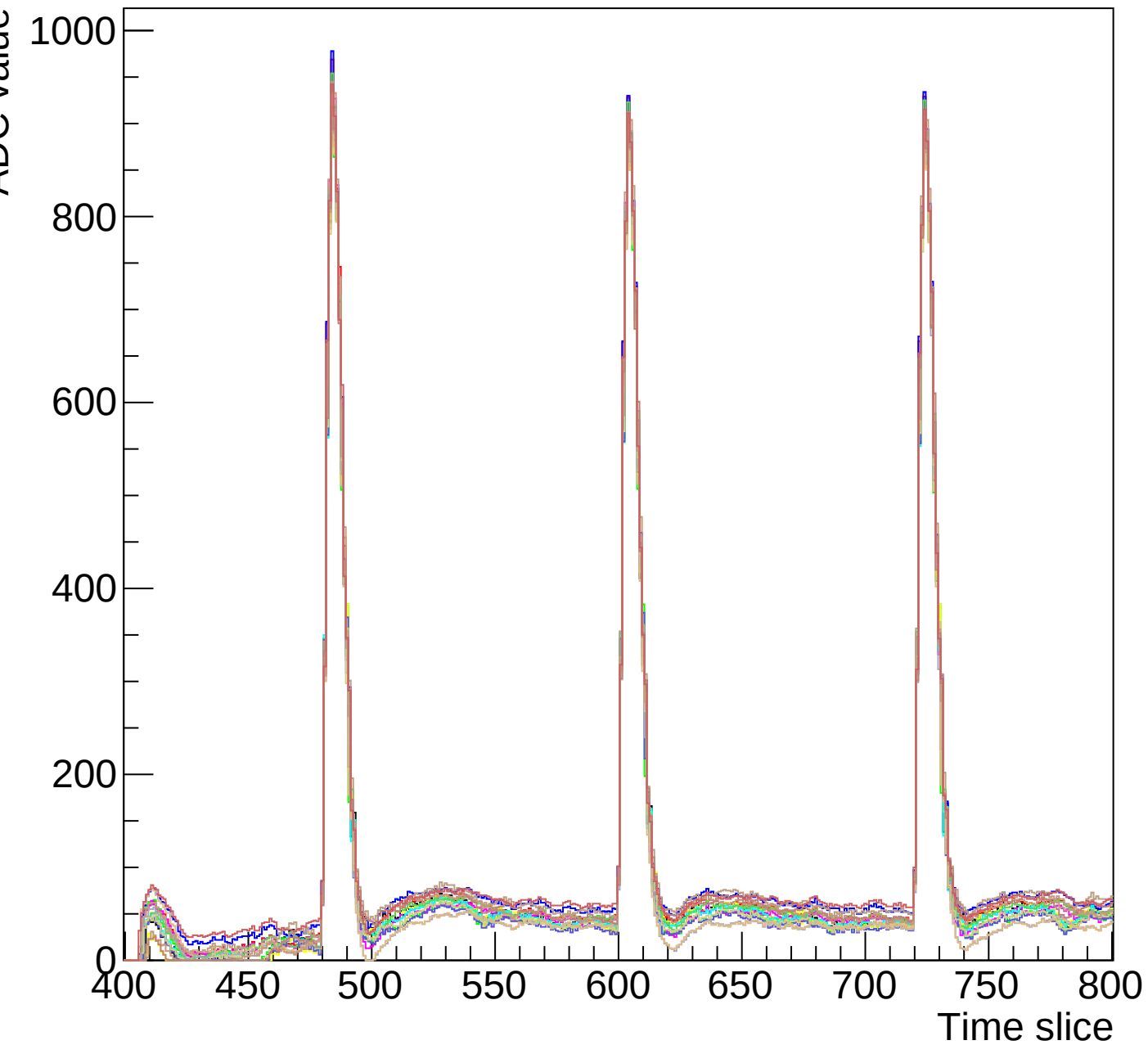
Run 3 event 7 mcm 0 chip 4 clk3-s3-zoom
