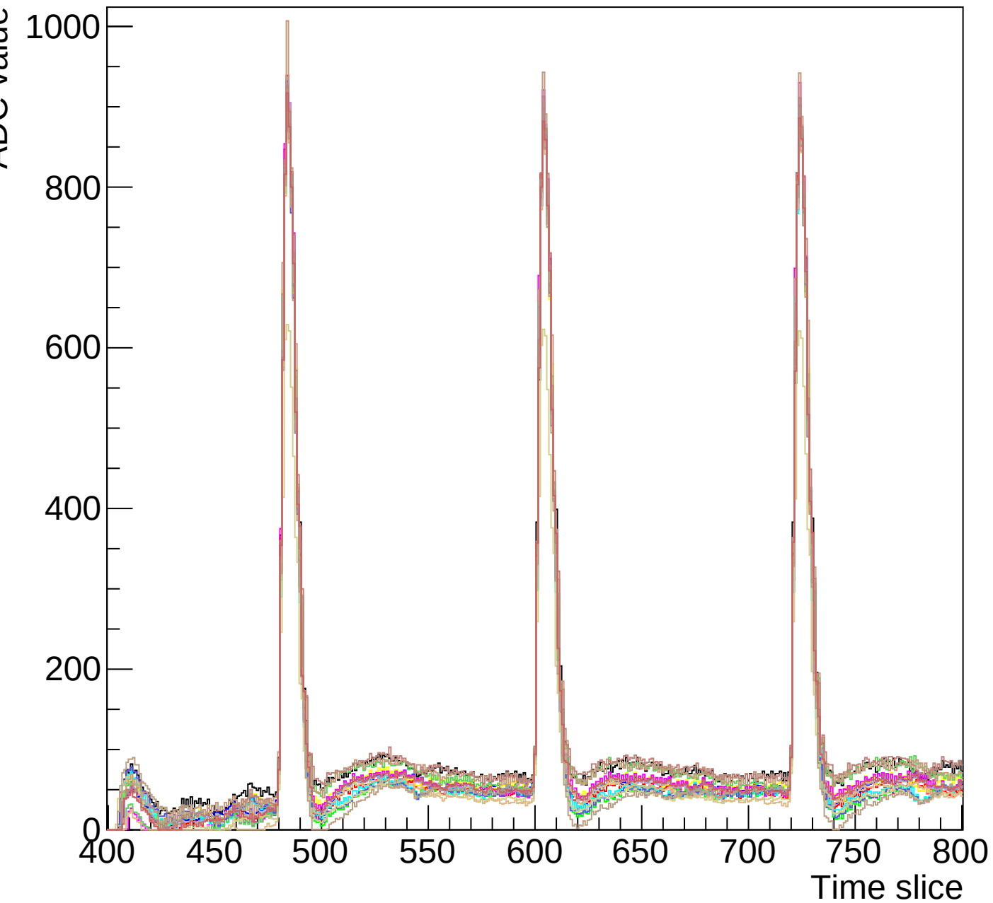
Run 3 event 7 mcm 0 chip 7 clk3-s3-zoom
