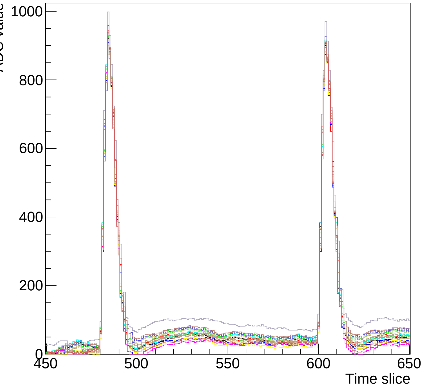
Run 3 event 7 mcm 0 chip 1 clk3-s3-zoom1
