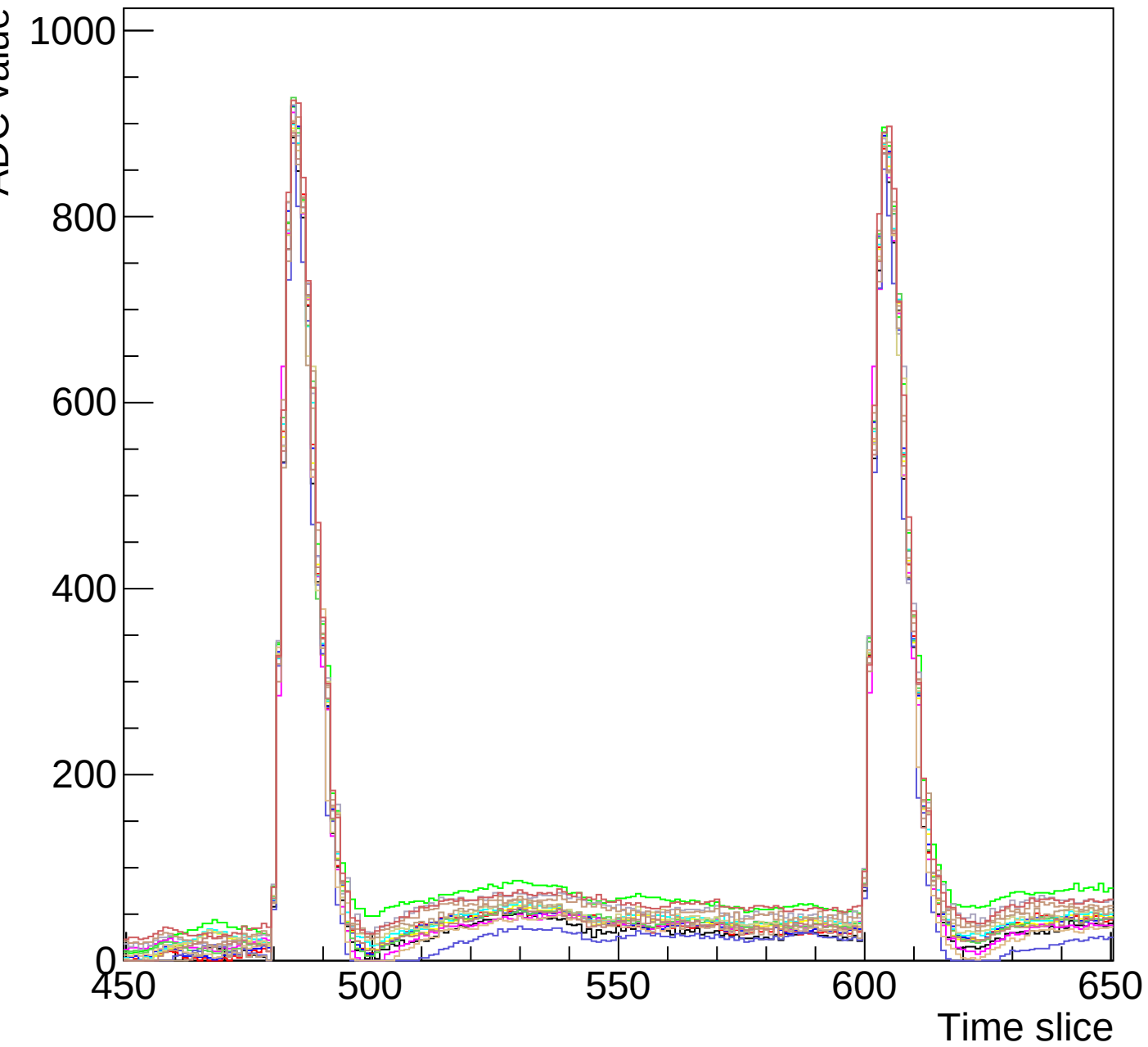
Run 3 event 7 mcm 0 chip 6 clk3-s3-zoom1
