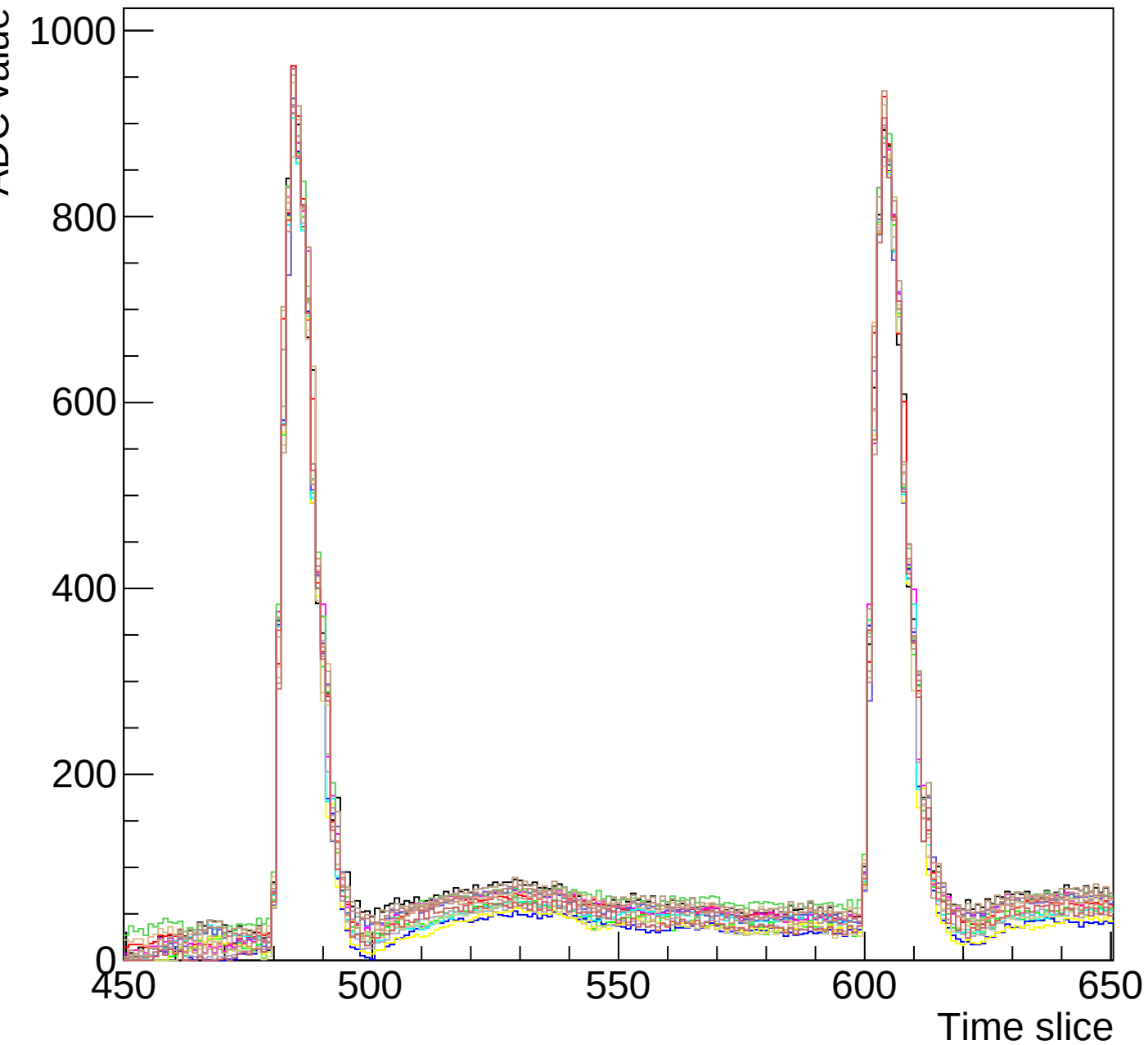
Run 3 event 7 mcm 0 chip 5 clk3-s3-zoom1
