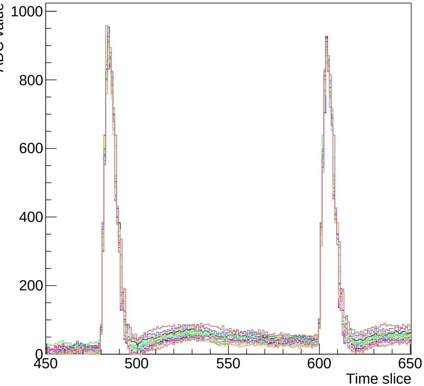
Run 3 event 7 mcm 0 chip 3 clk3-s3-zoom1
