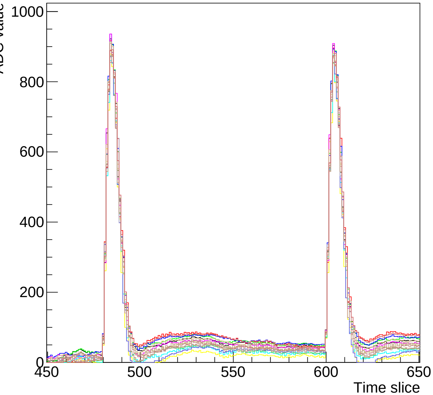
Run 3 event 7 mcm 0 chip 0 clk3-s3-zoom1
