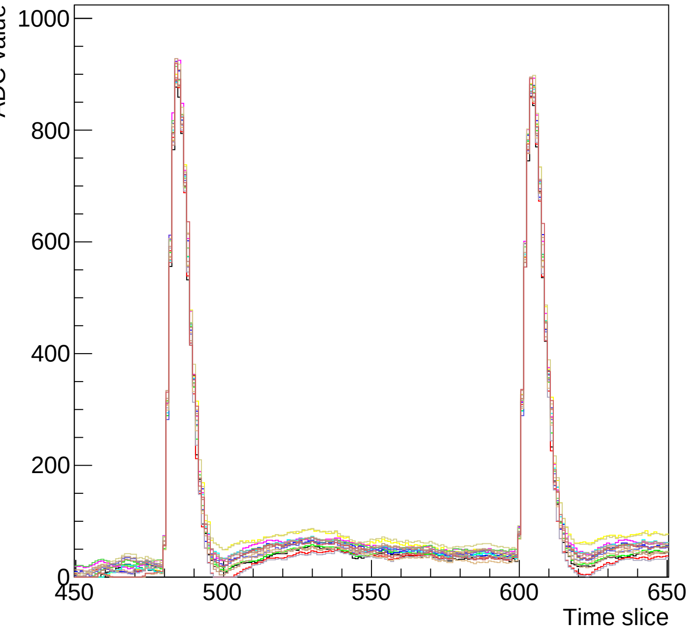
Run 3 event 7 mcm 0 chip 2 clk3-s3-zoom1
