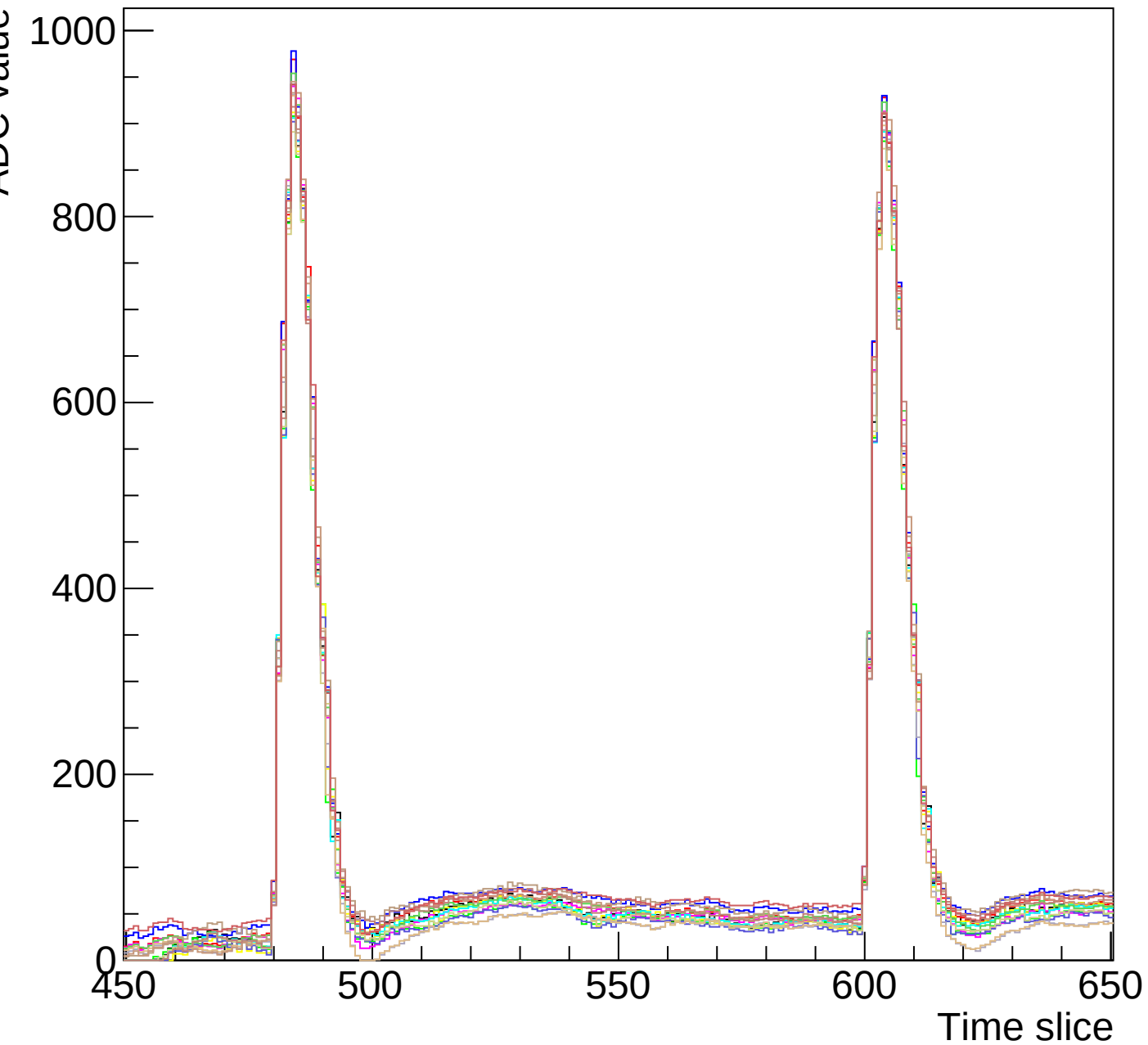
Run 3 event 7 mcm 0 chip 4 clk3-s3-zoom1
