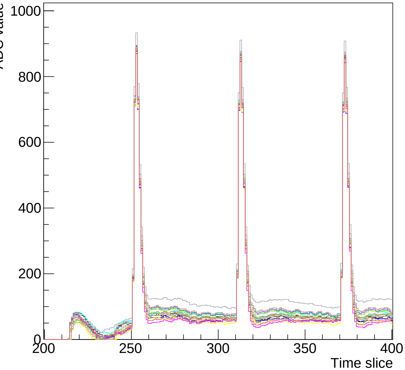
Run 0 event 8 mcm 0 chip 1 clk0-s3-zoom
