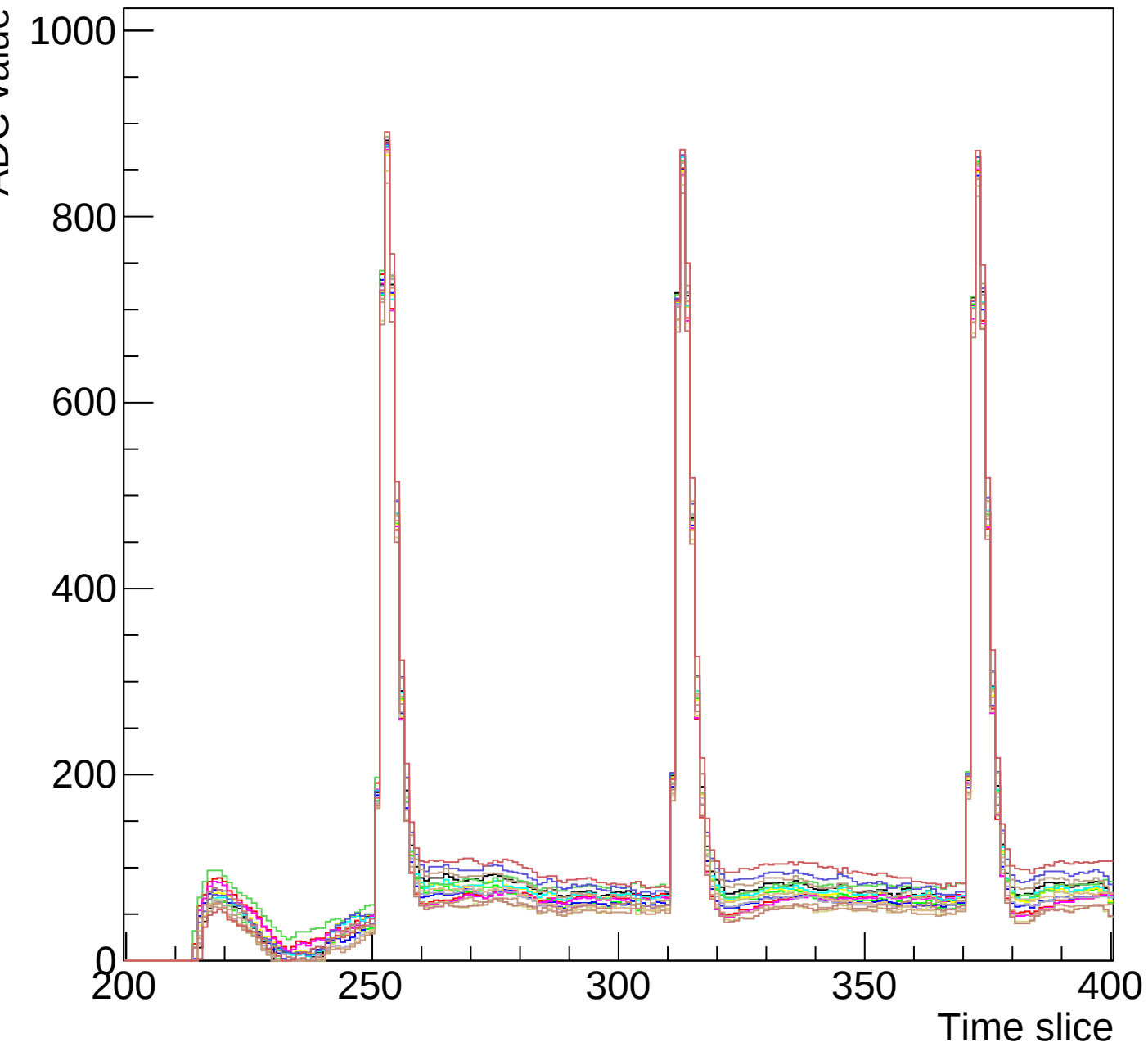
Run 0 event 8 mcm 0 chip 3 clk0-s3-zoom
