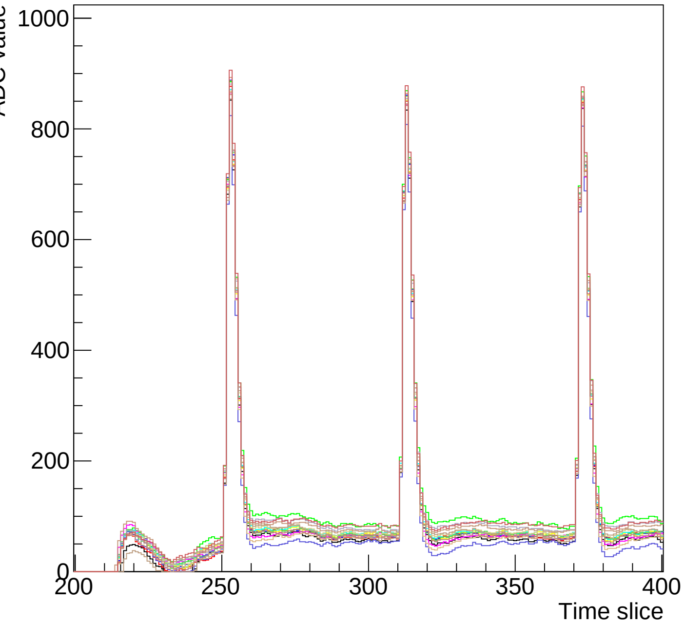
Run 0 event 8 mcm 0 chip 6 clk0-s3-zoom
