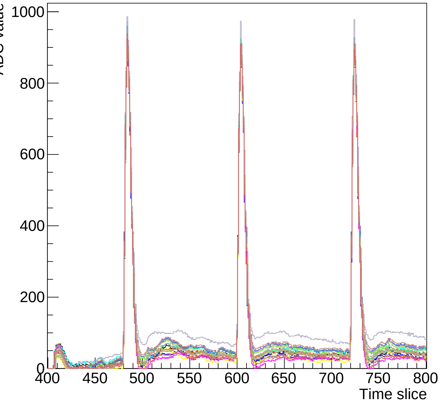
Run 3 event 8 mcm 0 chip 1 clk3-s3-zoom
