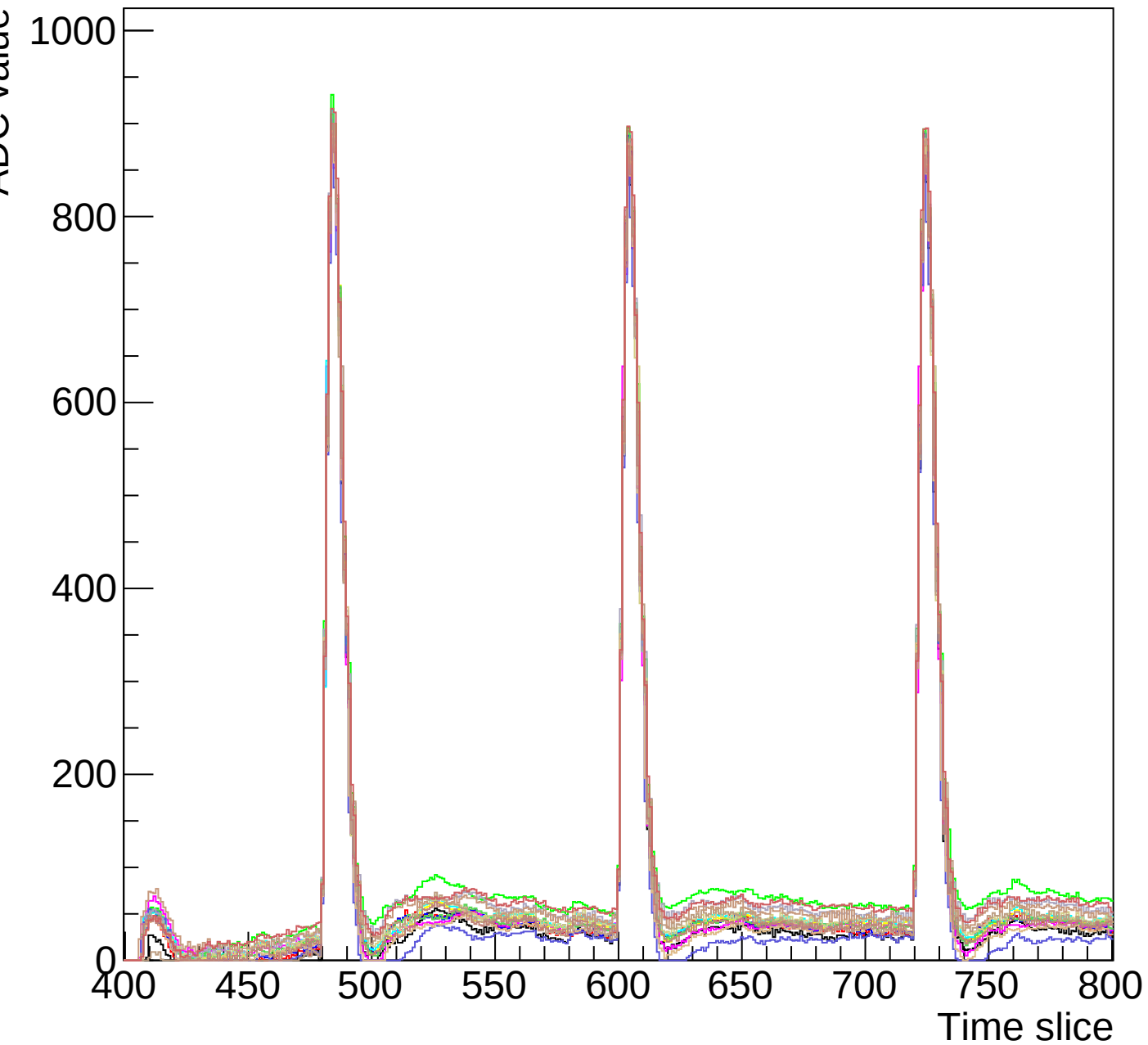
Run 3 event 8 mcm 0 chip 6 clk3-s3-zoom
