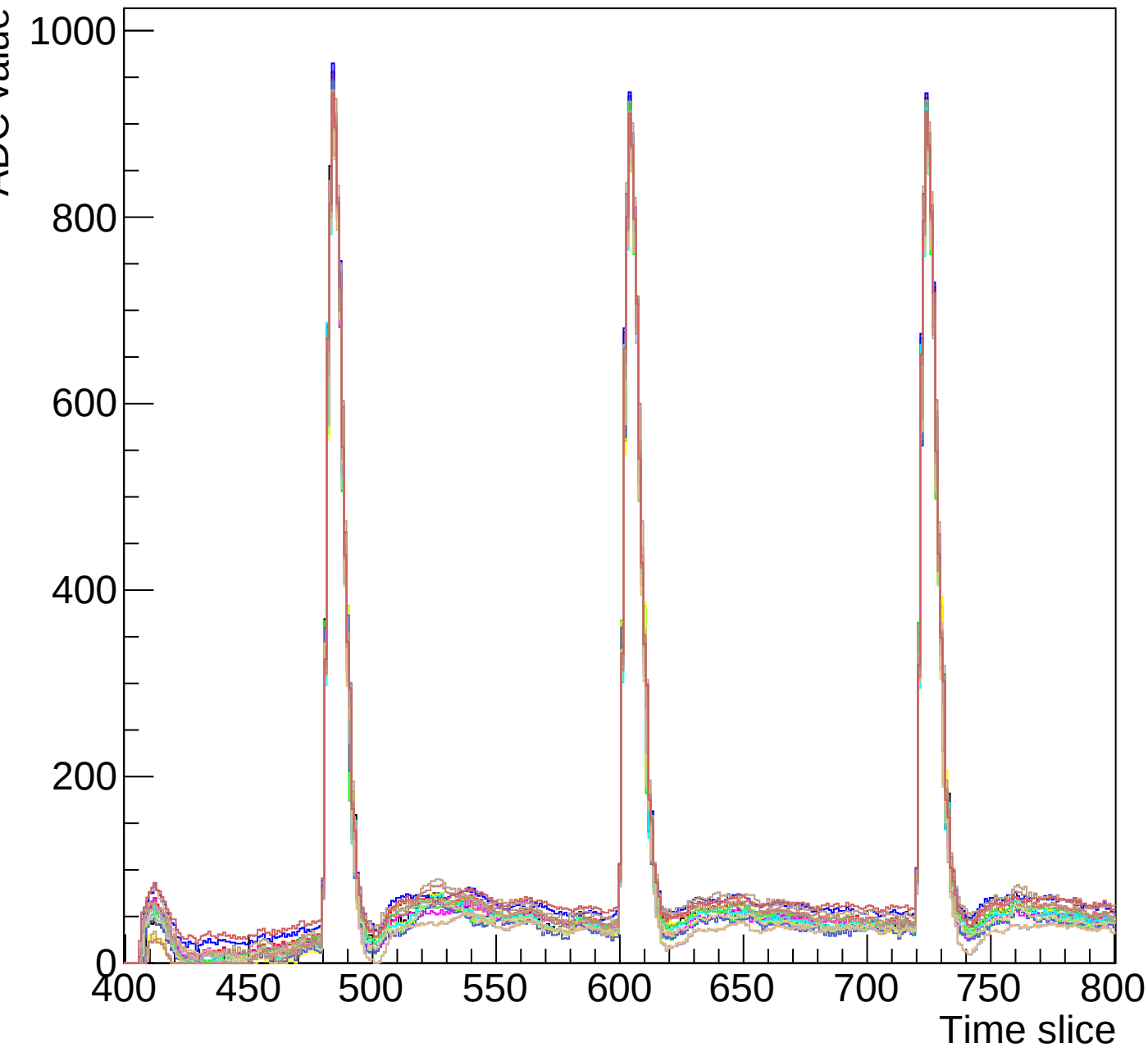
Run 3 event 8 mcm 0 chip 4 clk3-s3-zoom
