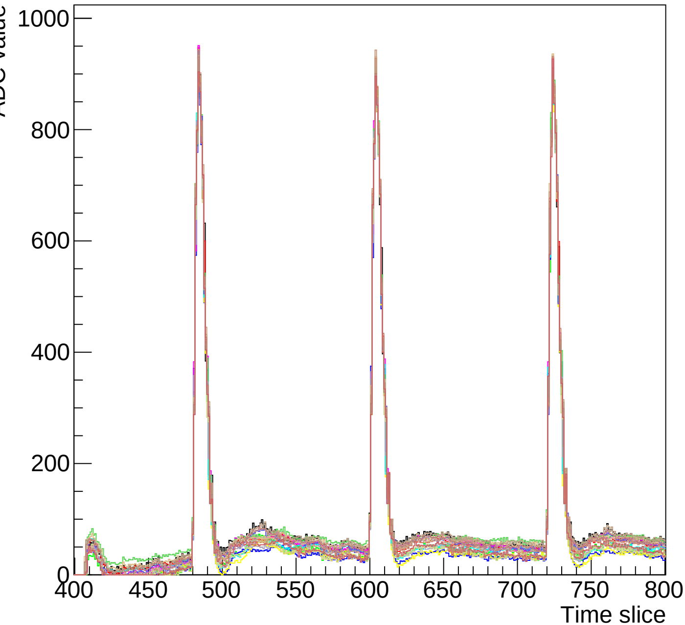
Run 3 event 8 mcm 0 chip 5 clk3-s3-zoom
