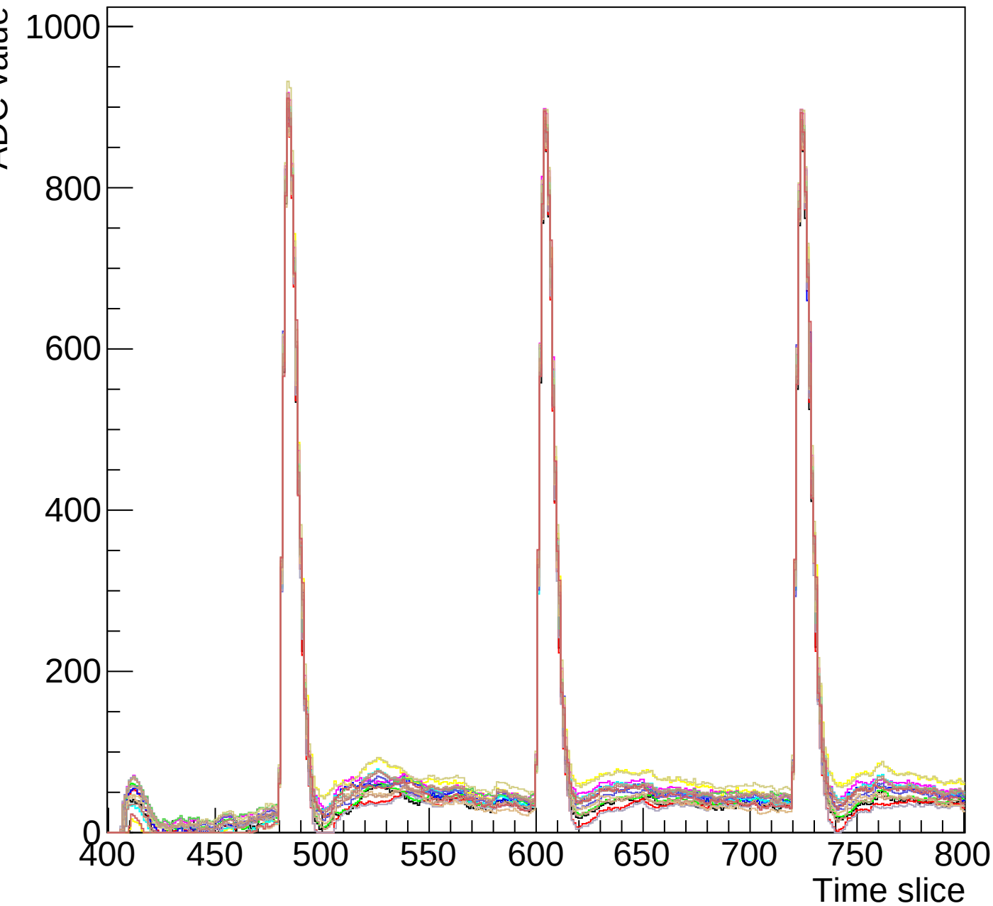
Run 3 event 8 mcm 0 chip 2 clk3-s3-zoom
