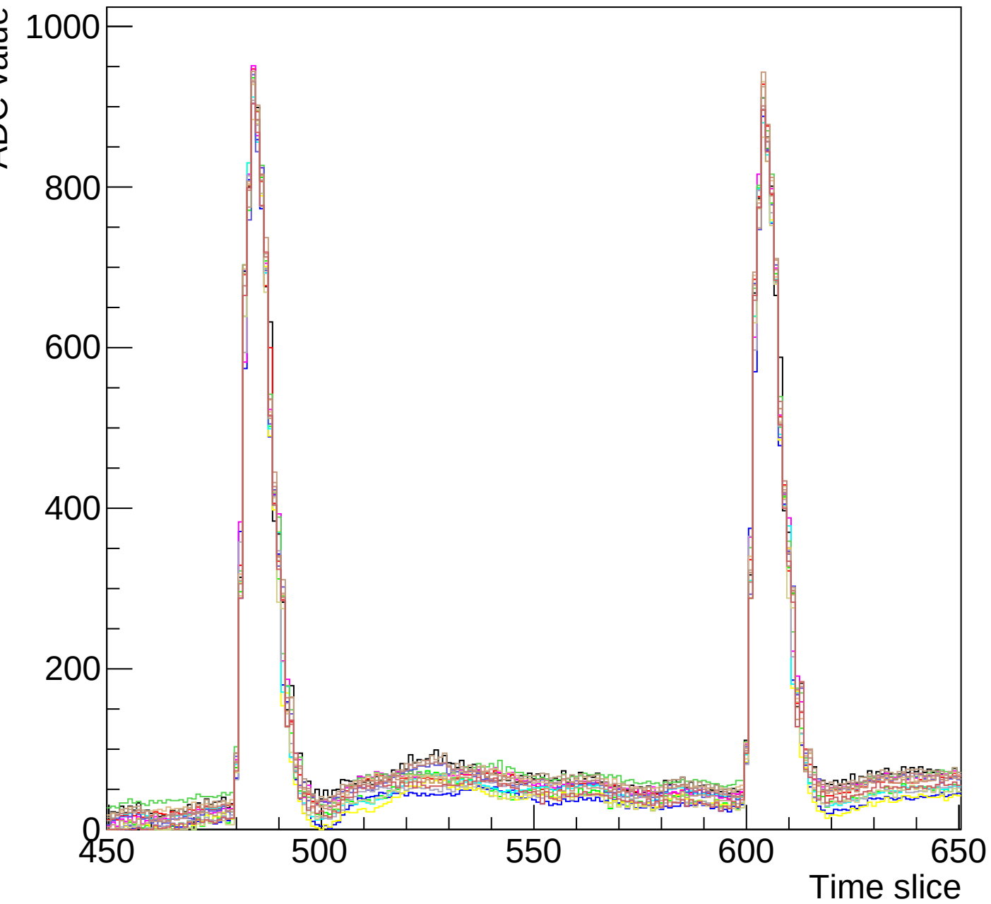
Run 3 event 8 mcm 0 chip 5 clk3-s3-zoom1
