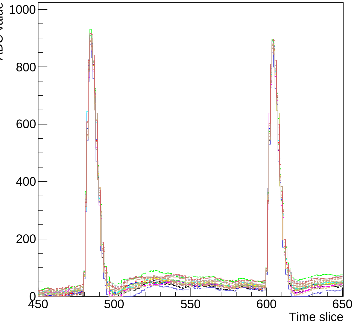
Run 3 event 8 mcm 0 chip 6 clk3-s3-zoom1
