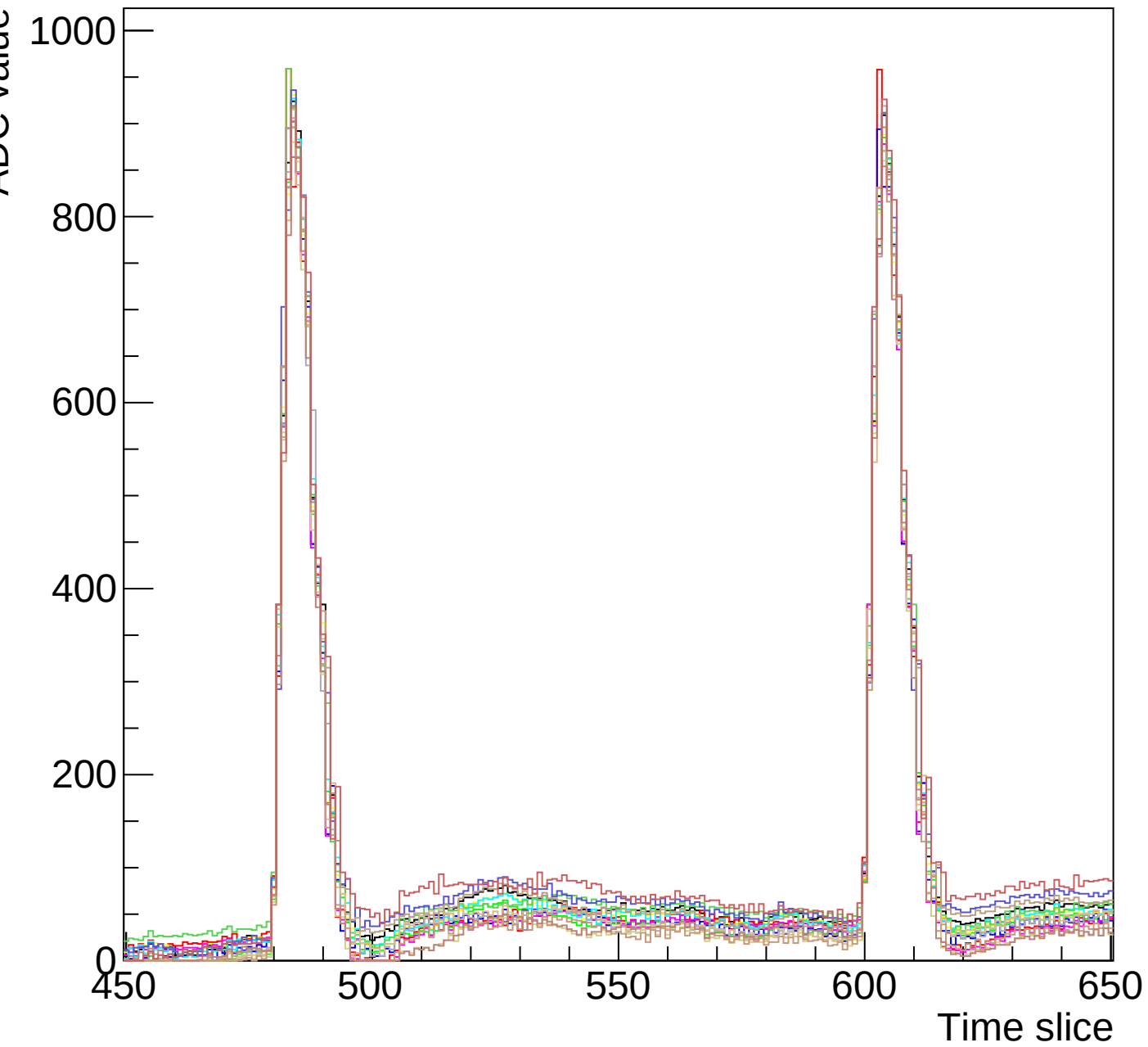
Run 3 event 8 mcm 0 chip 3 clk3-s3-zoom1
