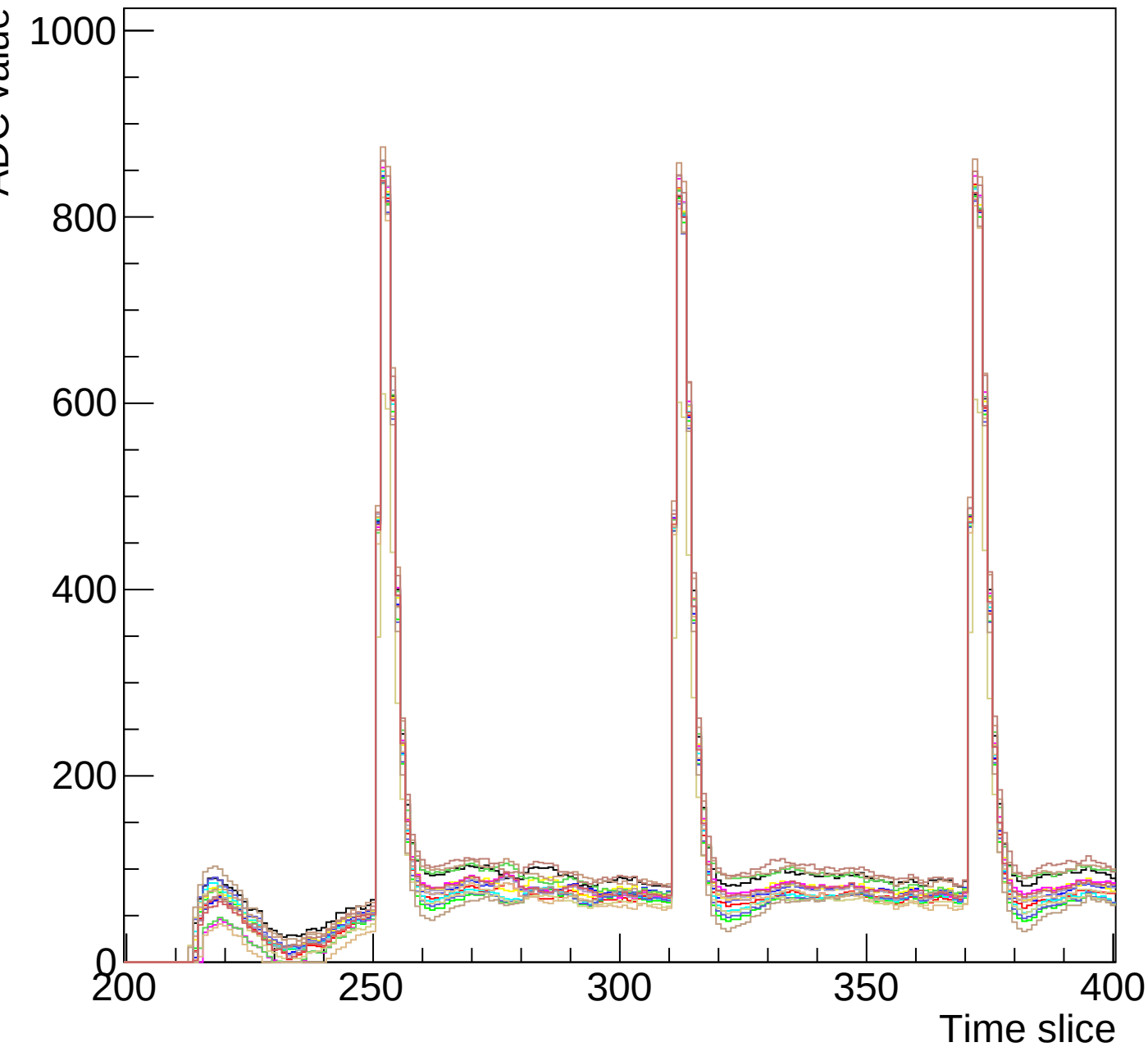
Run 0 event 9 mcm 0 chip 7 clk0-s3-zoom
