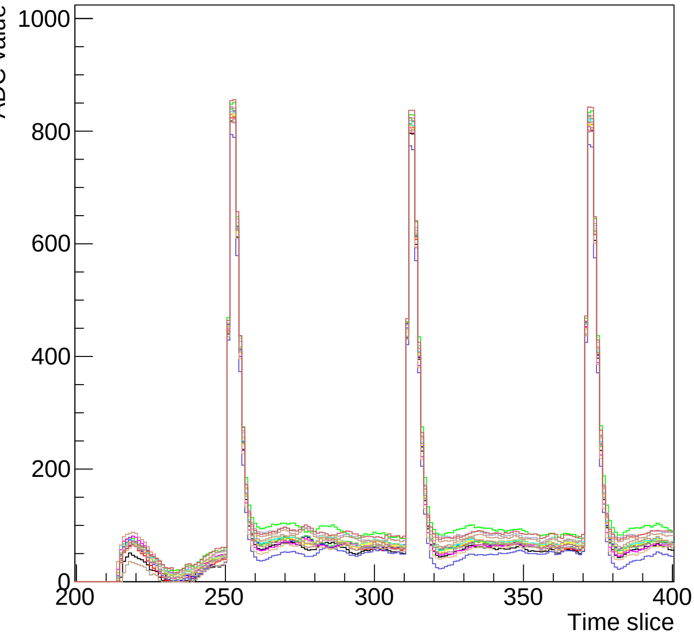
Run 0 event 9 mcm 0 chip 6 clk0-s3-zoom
