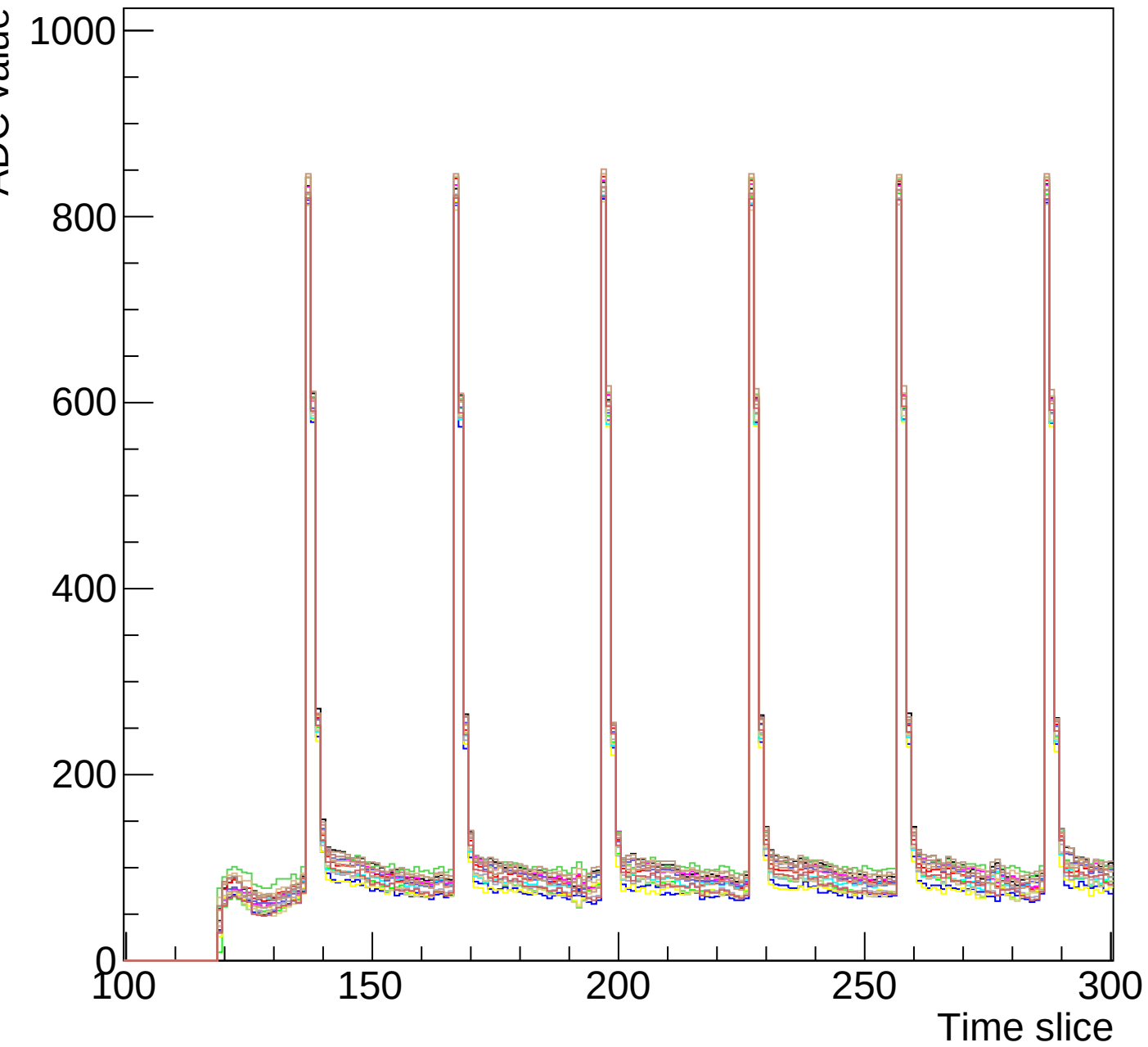
Run 1 event 9 mcm 0 chip 5 clk1-s3-zoom
