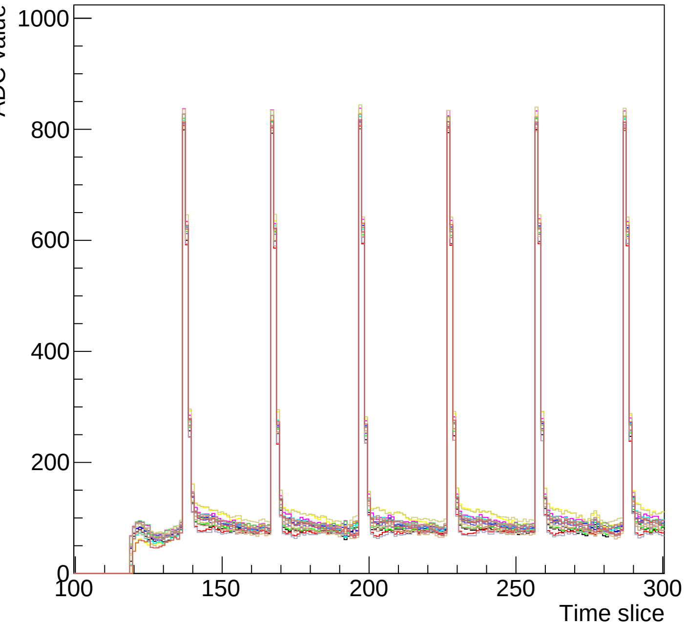
Run 1 event 9 mcm 0 chip 2 clk1-s3-zoom
