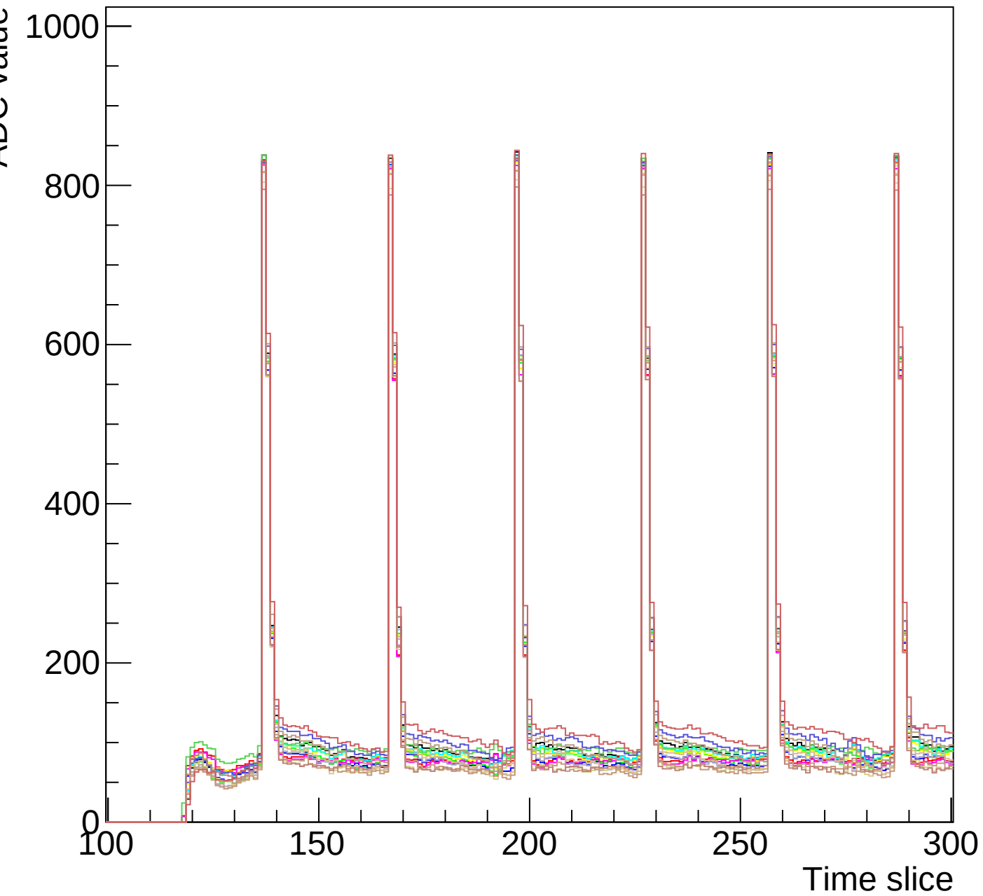
Run 1 event 9 mcm 0 chip 3 clk1-s3-zoom
