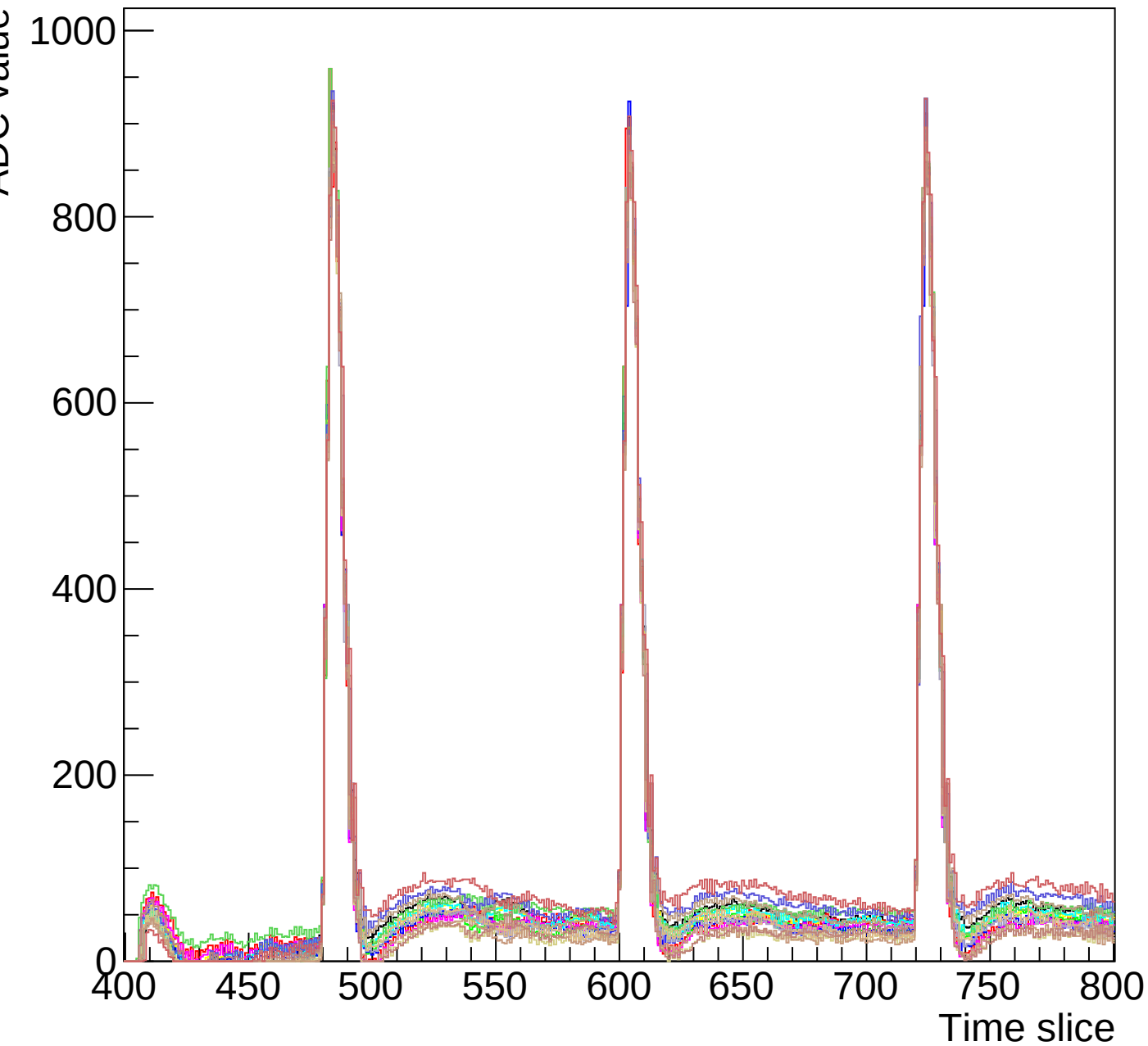
Run 3 event 9 mcm 0 chip 3 clk3-s3-zoom
