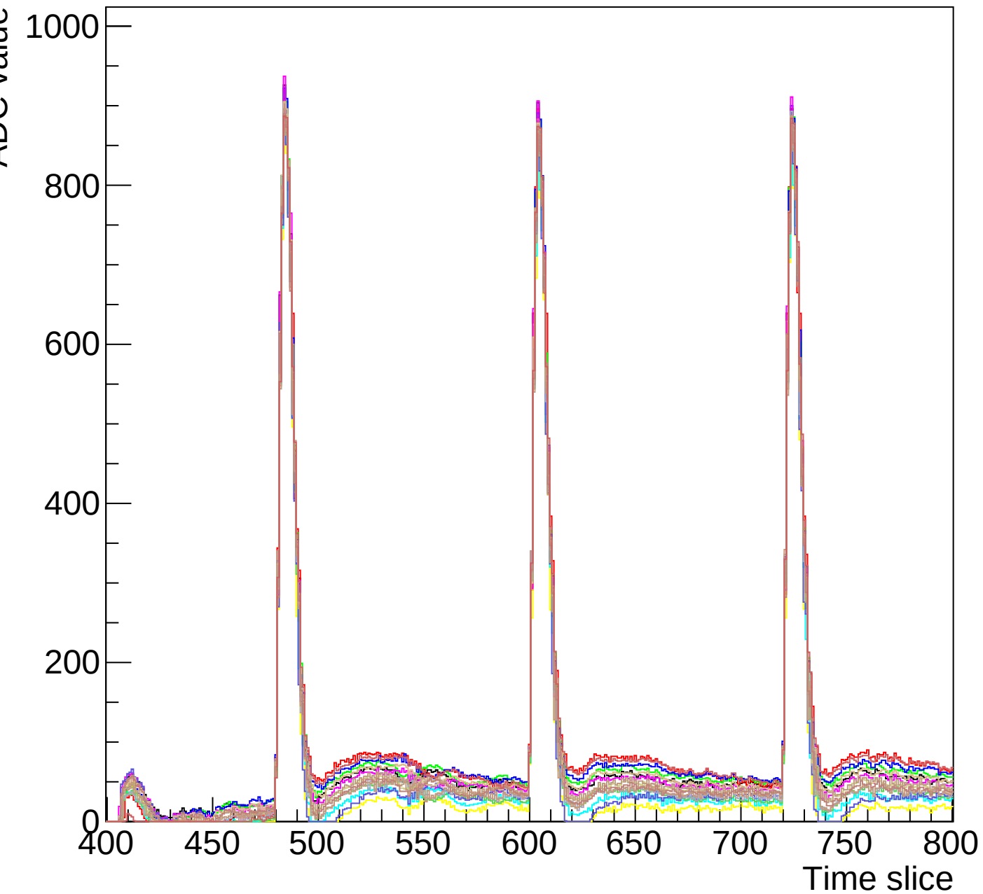
Run 3 event 9 mcm 0 chip 0 clk3-s3-zoom
