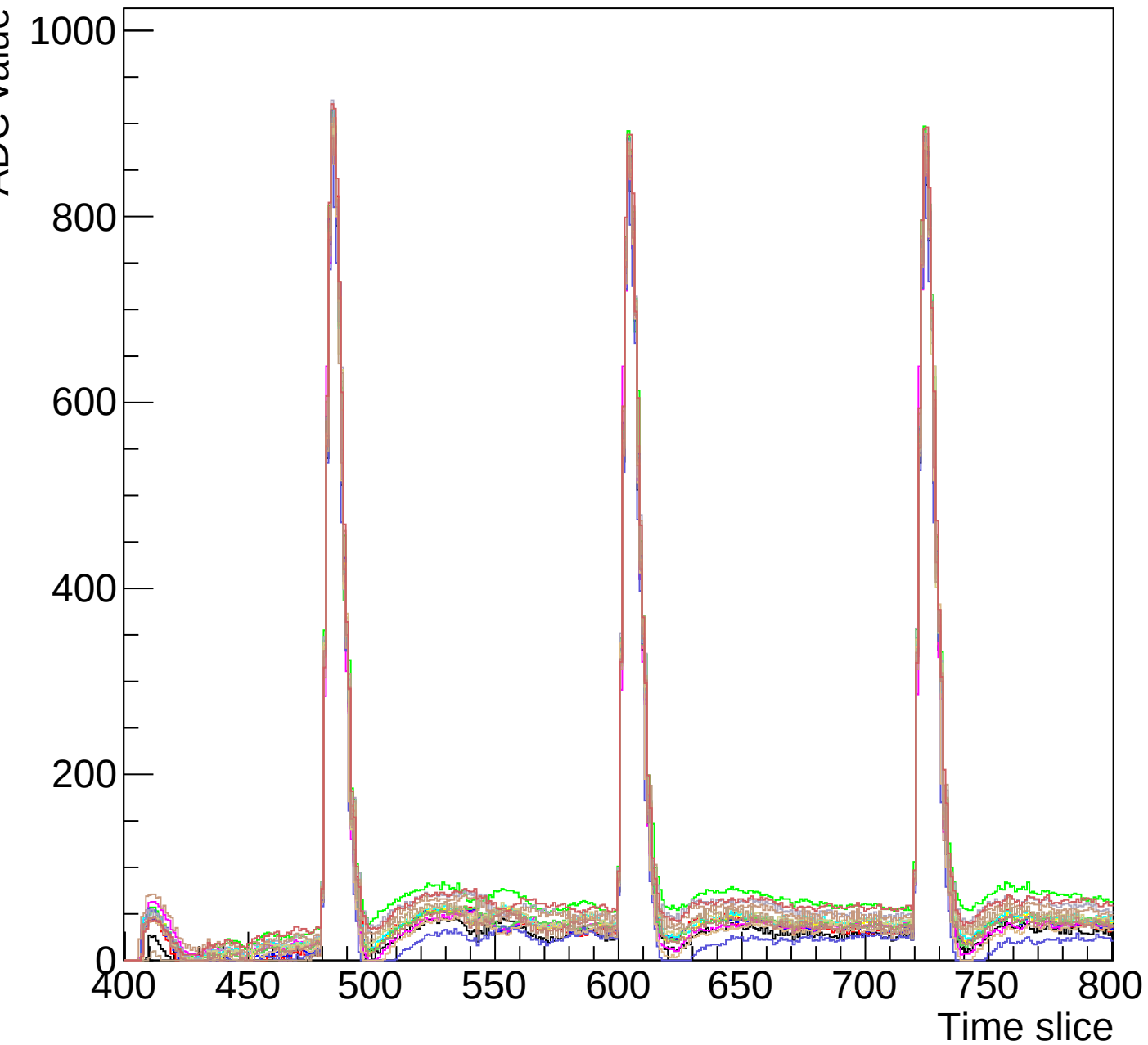
Run 3 event 9 mcm 0 chip 6 clk3-s3-zoom
