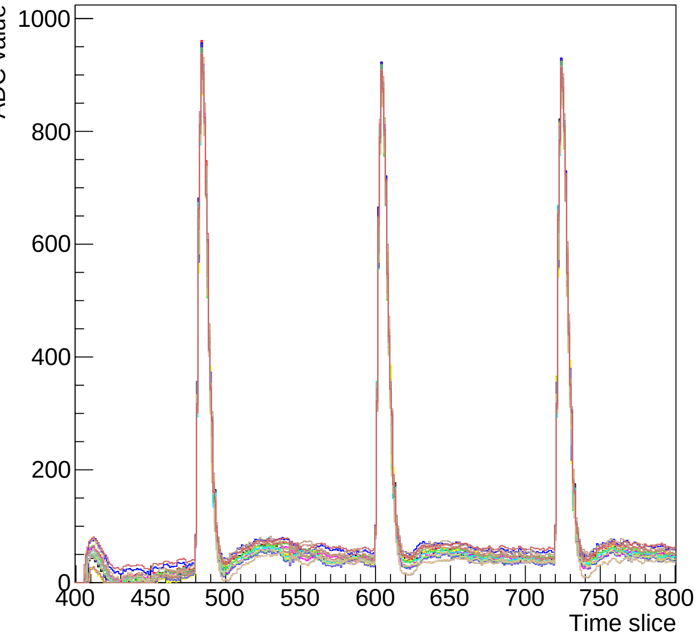
Run 3 event 9 mcm 0 chip 4 clk3-s3-zoom
