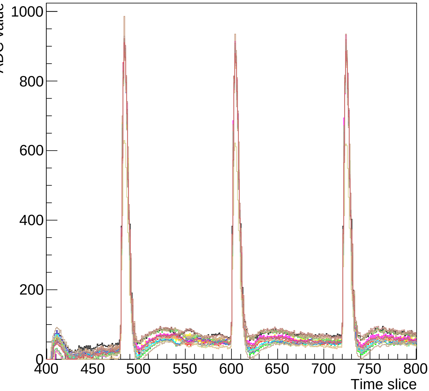
Run 3 event 9 mcm 0 chip 7 clk3-s3-zoom
