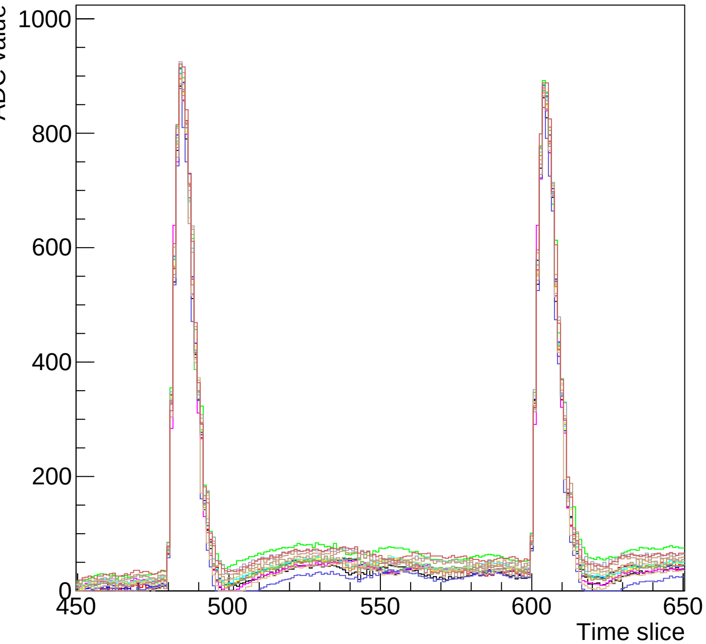
Run 3 event 9 mcm 0 chip 6 clk3-s3-zoom1
