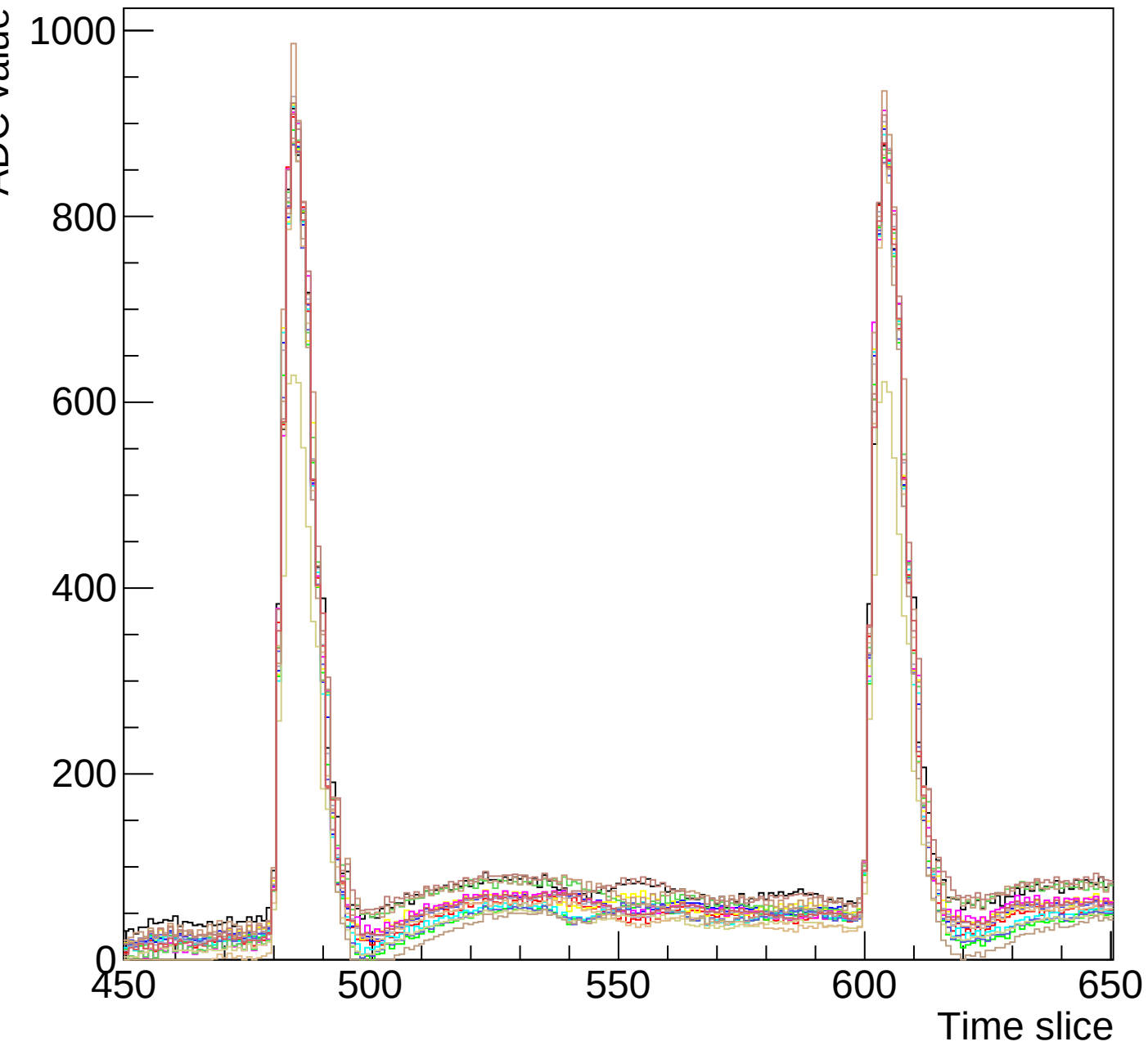
Run 3 event 9 mcm 0 chip 7 clk3-s3-zoom1
