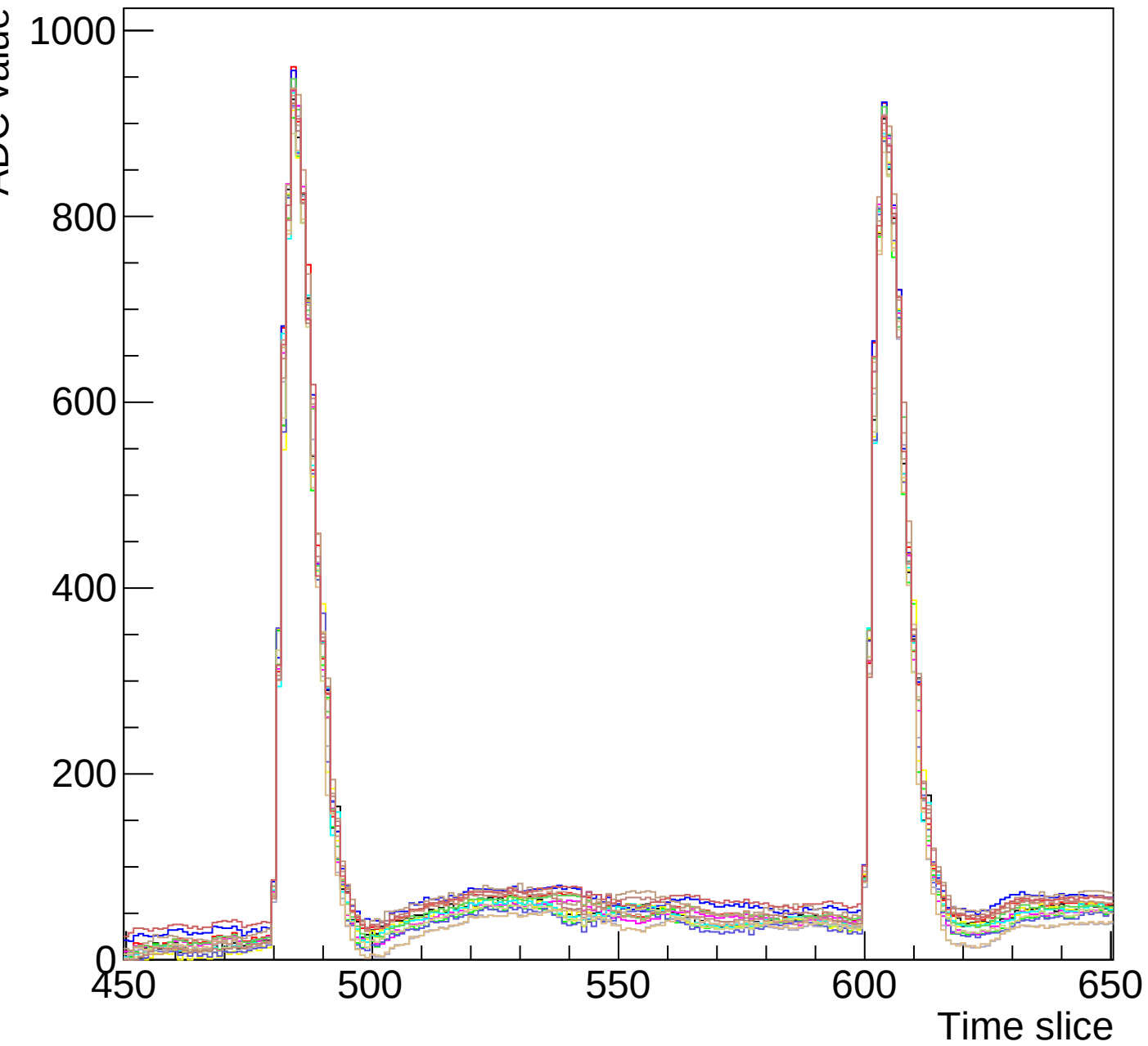
Run 3 event 9 mcm 0 chip 4 clk3-s3-zoom1
