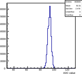
Pedestals readout-500evts ch 33 debug
