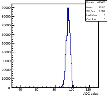
Pedestals readout-500evts ch 32 debug
