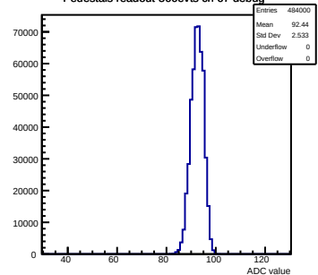
Pedestals readout-500evts ch 67 debug
