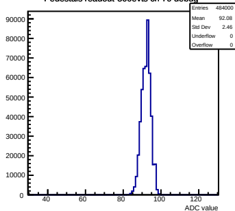
Pedestals readout-500evts ch 70 debug
