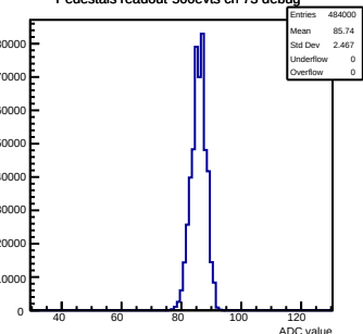
Pedestals readout-500evts ch 73 debug
