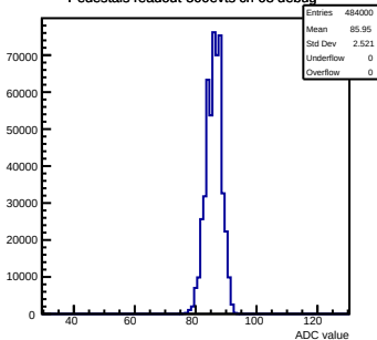
Pedestals readout-500evts ch 68 debug
