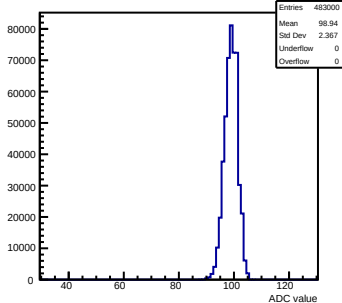
Pedestals readout-500evts ch 98 debug
