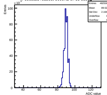
Pedestals readout-500evts ch 55 debug
