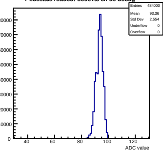
Pedestals readout-500evts ch 65 debug
