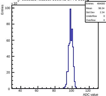
Pedestals readout-500evts ch 76 debug
