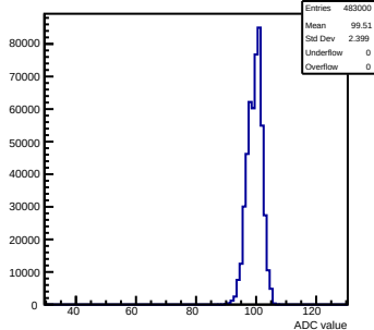
Pedestals readout-500evts ch 99 debug
