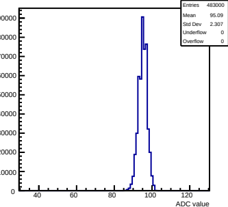
Pedestals readout-500evts ch 45 debug
