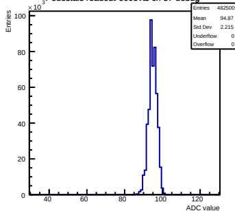
Pedestals readout-500evts ch 57 debug
