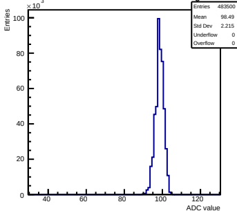
Pedestals readout-500evts ch 25 debug
