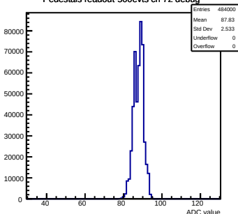
Pedestals readout-500evts ch 72 debug
