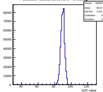
Pedestals readout-500evts ch 49 debug
