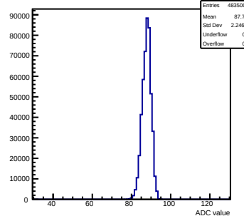
Pedestals readout-500evts ch 19 debug
