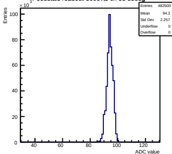
Pedestals readout-500evts ch 58 debug
