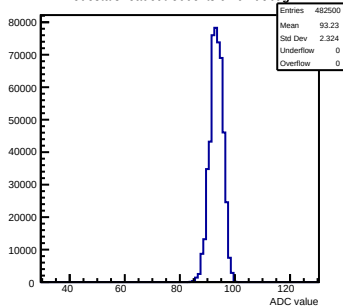
Pedestals readout-500evts ch 62 debug
