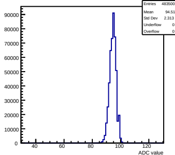
Pedestals readout-500evts ch 18 debug
