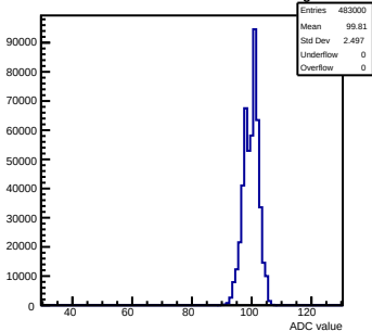
Pedestals readout-500evts ch 40 debug
