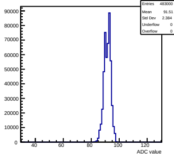
Pedestals readout-500evts ch 34 debug
