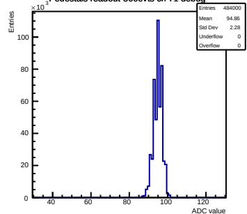
Pedestals readout-500evts ch 71 debug
