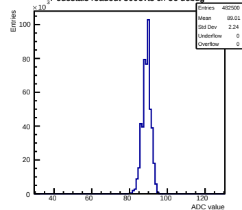
Pedestals readout-500evts ch 56 debug
