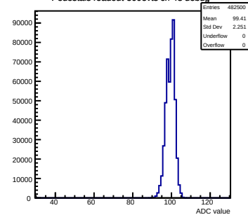
Pedestals readout-500evts ch 48 debug
