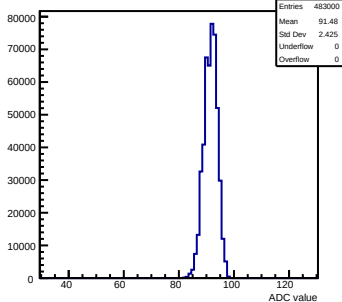
Pedestals readout-500evts ch 110 debug
