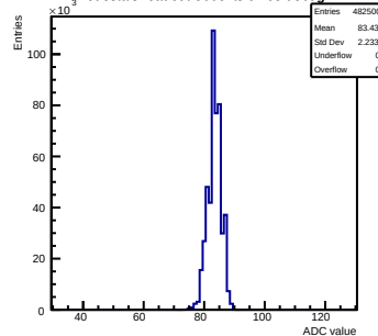
Pedestals readout-500evts ch 63 debug
