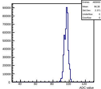
Pedestals readout-500evts ch 107 debug
