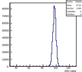
Pedestals readout-500evts ch 105 debug
