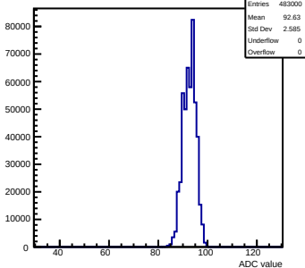
Pedestals readout-500evts ch 100 debug
