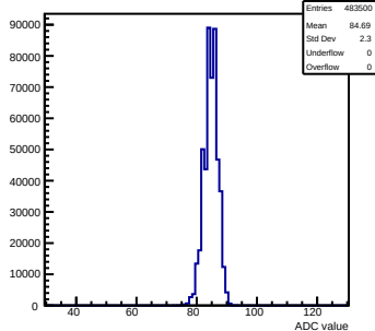
Pedestals readout-500evts ch 17 debug
