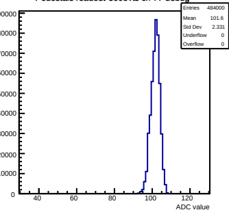
Pedestals readout-500evts ch 77 debug
