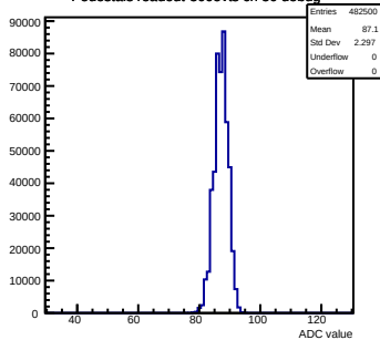
Pedestals readout-500evts ch 50 debug
