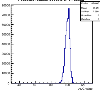
Pedestals readout-500evts ch 64 debug
