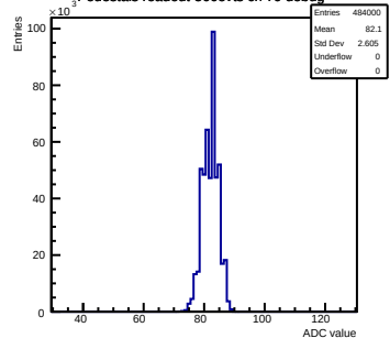
Pedestals readout-500evts ch 79 debug
