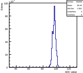
Pedestals readout-500evts ch 20 debug
