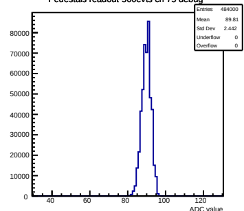
Pedestals readout-500evts ch 75 debug
