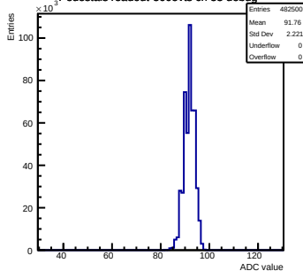
Pedestals readout-500evts ch 53 debug
