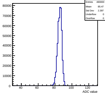
Pedestals readout-500evts ch 111 debug
