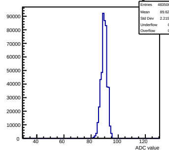
Pedestals readout-500evts ch 27 debug
