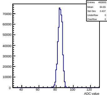
Pedestals readout-500evts ch 38 debug
