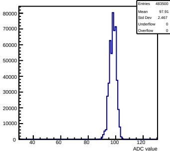
Pedestals readout-500evts ch 16 debug
