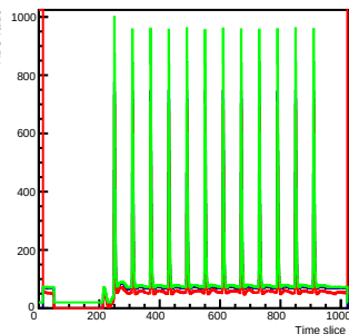
Run 0 Time mcm 0 chip 4 chan 4 debug
