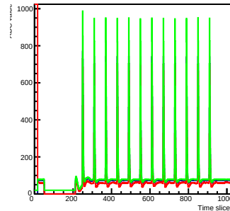
Run 0 Time mcm 0 chip 6 chan 14 debug
