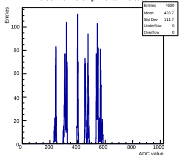
Pulse mcm 0 chip 2 chan 13 test1
