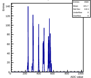
Pulse mcm 0 chip 2 chan 1 test1
