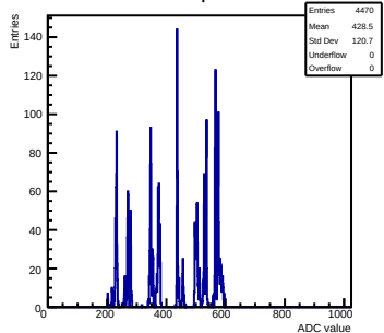
Pulse mcm 0 chip 6 chan 9 test1
