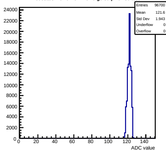
Pedestals mcm0-4C11-refV0-g0-s0-p1 ch 30 test1
