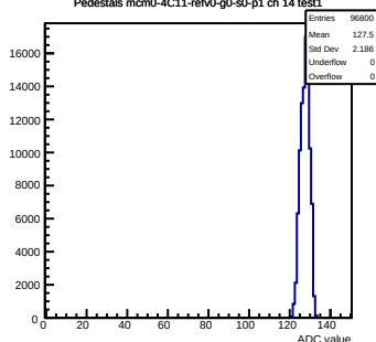
Pedestals mcm0-4C11-refV0-g0-s0-p1 ch 14 test1
