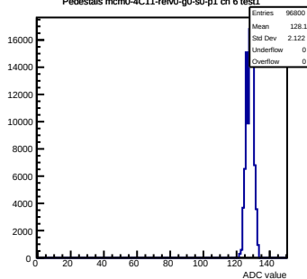
Pedestals mcm0-4C11-refV0-g0-s0-p1 ch 6 test1
