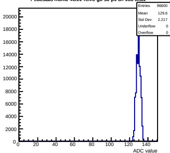
Pedestals mcm0-4C11-refV0-g0-s0-p1 ch 100 test1
