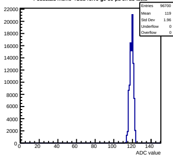
Pedestals mcm0-4C11-refV0-g0-s0-p1 ch 25 test1
