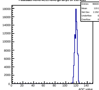
Pedestals mcm0-4C11-refV0-g0-s0-p1 ch 110 test1
