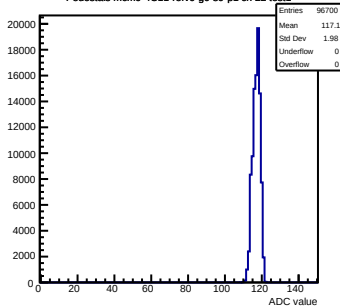
Pedestals mcm0-4C11-refV0-g0-s0-p1 ch 22 test1
