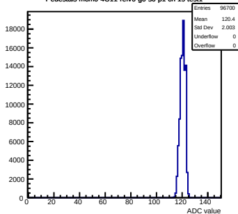
Pedestals mcm0-4C11-refV0-g0-s0-p1 ch 19 test1
