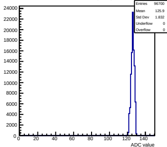
Pedestals mcm0-4C11-refV0-g0-s0-p1 ch 87 test1
