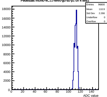
Pedestals mcm0-4C11-refV0-g0-s0-p1 ch 4 test1
