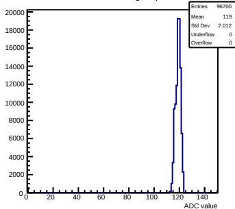
Pedestals mcm0-4C11-refV0-g0-s0-p1 ch 90 test1
