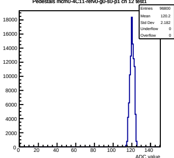
Pedestals mcm0-4C11-refV0-g0-s0-p1 ch 12 test1
