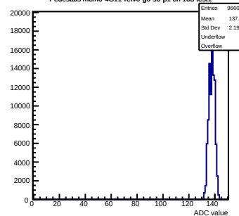
Pedestals mcm0-4C11-refV0-g0-s0-p1 ch 103 test1
