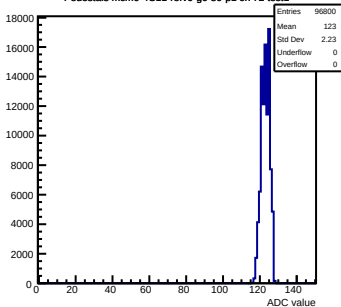
Pedestals mcm0-4C11-refV0-g0-s0-p1 ch 72 test1
