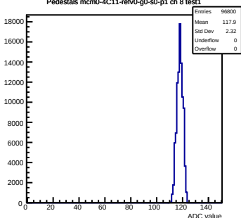
Pedestals mcm0-4C11-refV0-g0-s0-p1 ch 8 test1
