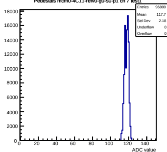
Pedestals mcm0-4C11-refV0-g0-s0-p1 ch 7 test1
