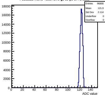
Pedestals mcm0-4C11-refV0-g0-s0-p1 ch 75 test1
