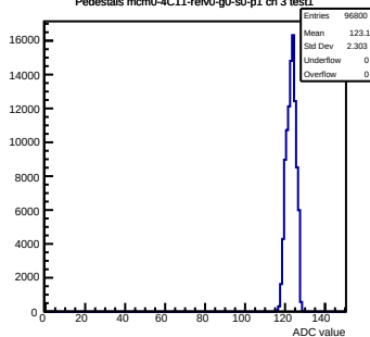
Pedestals mcm0-4C11-refV0-g0-s0-p1 ch 3 test1
