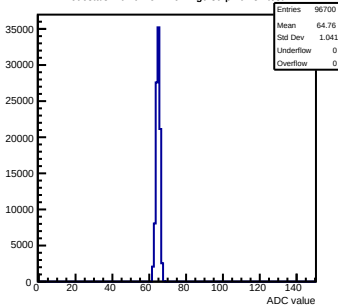
Pedestals mcm0-4C11-refV2-g0-s0-p1 ch 82 test1
