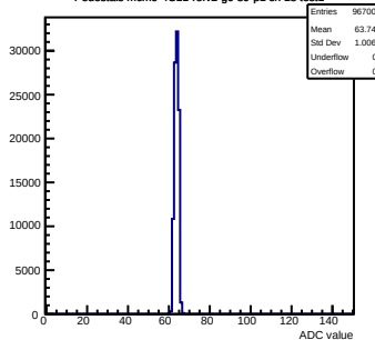
Pedestals mcm0-4C11-refV2-g0-s0-p1 ch 18 test1
