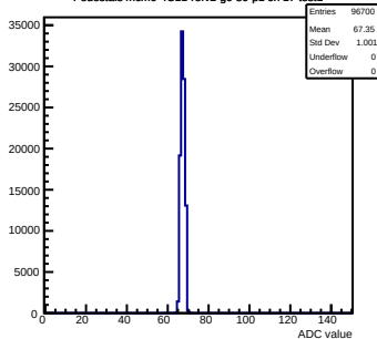
Pedestals mcm0-4C11-refV2-g0-s0-p1 ch 17 test1
