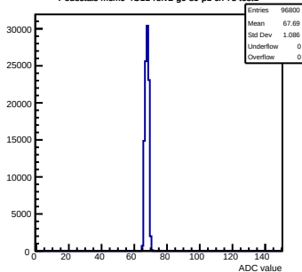
Pedestals mcn0-4C11-refV2-g0-s0-p1 ch 75 test1
