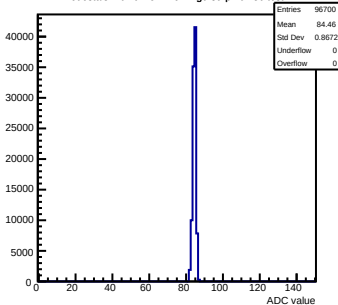
Pedestals mcm0-4C11-refV2-g0-s0-p1 ch 86 test1
