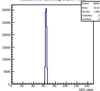
Pedestals mcn0-4C11-refV2-g0-s0-p1 ch 74 test1
