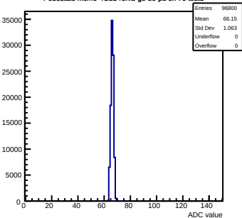
Pedestals mcn0-4C11-refV2-g0-s0-p1 ch 76 test1
