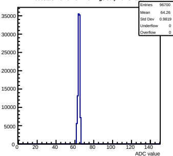
Pedestals mcm0-4C11-refV2-g0-s0-p1 ch 84 test1
