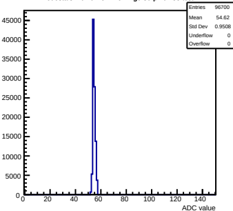
Pedestals mcm0-4C11-refV2-g0-s0-p1 ch 88 test1
