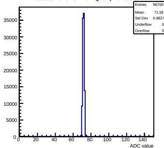
Pedestals mcm0-4C11-refV2-g0-s0-p1 ch 83 test1
