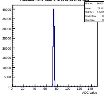
Pedestals mcn0-4C11-refV2-g0-s0-p1 ch 65 test1
