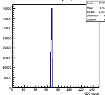
Pedestals mcm0-4C11-refV2-g0-s0-p1 ch 30 test1
