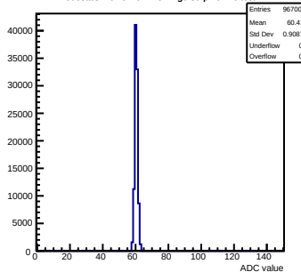
Pedestals mcm0-4C11-refV2-g0-s0-p1 ch 26 test1
