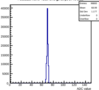
Pedestals mcn0-4C11-refV2-g0-s0-p1 ch 72 test1
