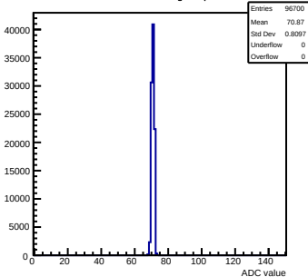
Pedestals mcm0-4C11-refV2-g0-s0-p1 ch 93 test1
