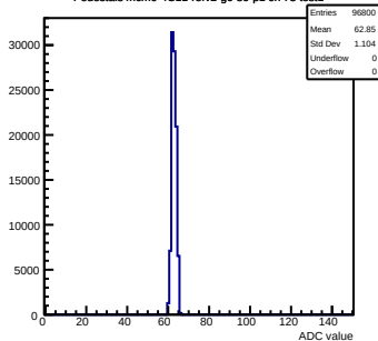
Pedestals mcn0-4C11-refV2-g0-s0-p1 ch 73 test1
