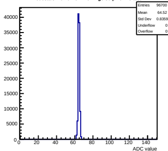
Pedestals mcm0-4C11-refV2-g0-s0-p1 ch 25 test1
