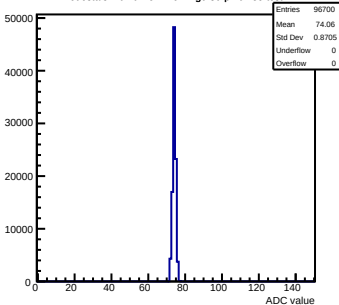
Pedestals mcm0-4C11-refV2-g0-s0-p1 ch 85 test1
