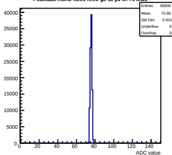
Pedestals mcn0-4C11-refV2-g0-s0-p1 ch 71 test1
