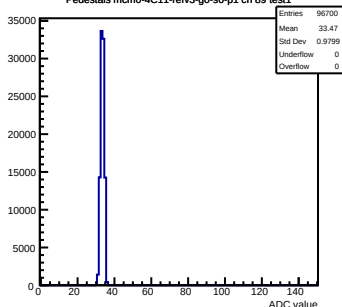
Pedestals mcm0-4C11-refV3-g0-s0-p1 ch 89 test1
