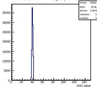
Pedestals mcm0-4C11-refV3-g0-s0-p1 ch 115 test1
