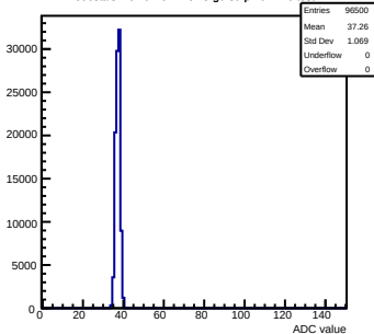
Pedestals mcm0-4C11-refV3-g0-s0-p1 ch 112 test1
