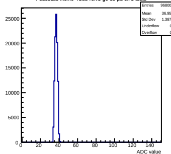
Pedestals mcm0-4C11-refv3-g0-s0-p1 ch 3 test1
