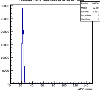
Pedestals mcm0-4C11-refv3-g0-s0-p1 ch 4 test1
