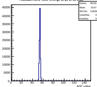
Pedestals mcm0-4C11-refV3-g0-s0-p1 ch 86 test1
