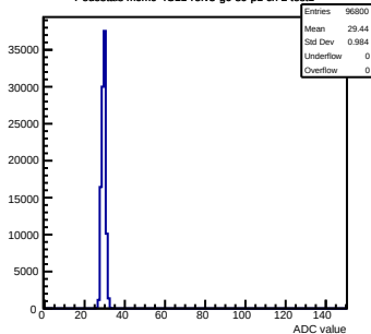
Pedestals mcm0-4C11-refv3-g0-s0-p1 ch 2 test1
