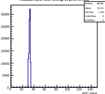
Pedestals mcm0-4C11-refV3-g0-s0-p1 ch 84 test1
