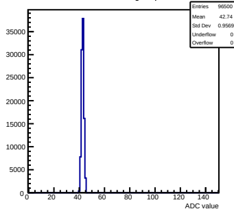
Pedestals mcm0-4C11-refV3-g0-s0-p1 ch 121 test1
