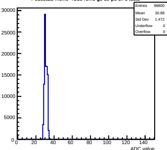
Pedestals mcm0-4C11-refv3-g0-s0-p1 ch 8 test1
