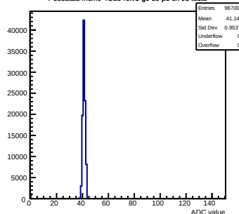
Pedestals mcm0-4C11-refV3-g0-s0-p1 ch 95 test1
