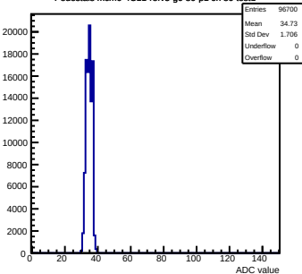
Pedestals mcm0-4C11-refV3-g0-s0-p1 ch 80 test1
