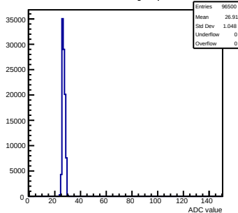
Pedestals mcm0-4C11-refV3-g0-s0-p1 ch 126 test1
