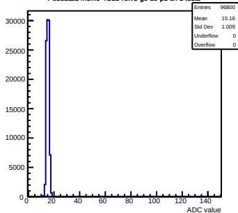
Pedestals mcm0-4C11-refv3-g0-s0-p1 ch 1 test1
