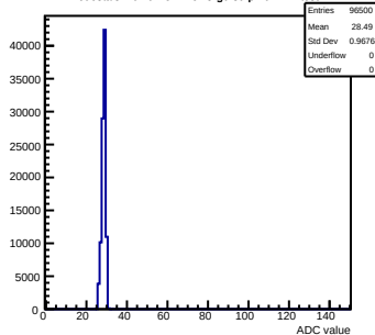
Pedestals mcm0-4C11-refV3-g0-s0-p1 ch 117 test1
