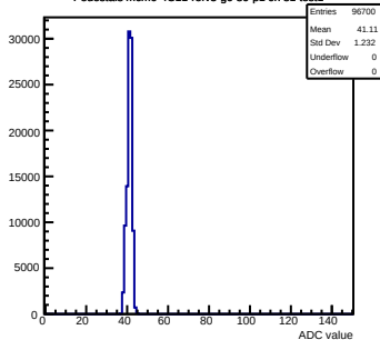
Pedestals mcm0-4C11-refV3-g0-s0-p1 ch 81 test1
