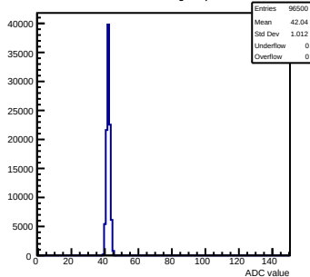
Pedestals mcm0-4C11-refV3-g0-s0-p1 ch 122 test1
